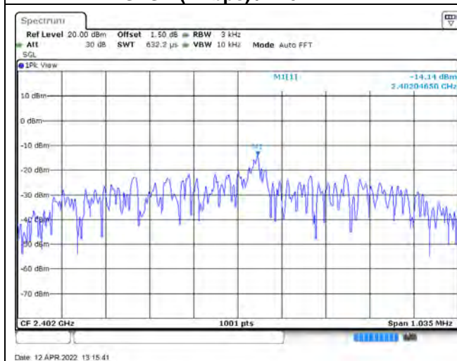
GFSK (1Mbps) / 2402 MHz
