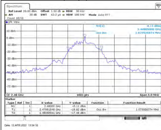
GFSK (1Mbps) / 2480 MHz
