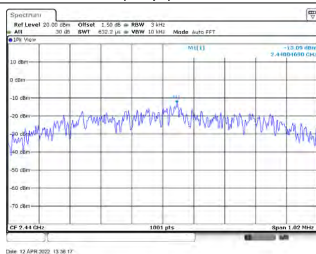
GFSK (1Mbps) / 2440 MHz
