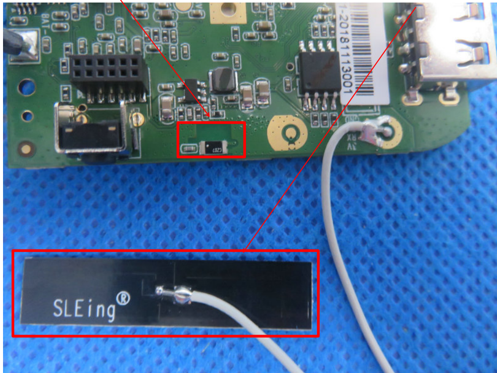
2.4GHz WiFi PCB Antenna
