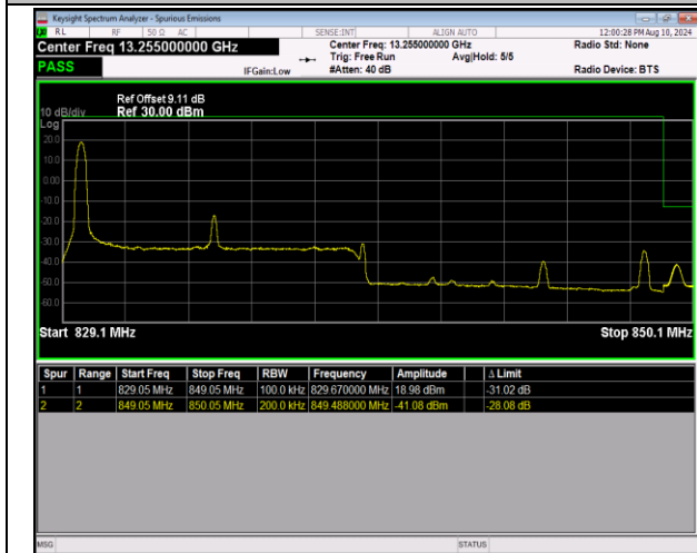
5-5-10MHz-10MHz-16QAM@16QAM-16QAM@16QAM-20501-20600-1RB#0@50RB#0-0RB#0@50RB#0-PASS
