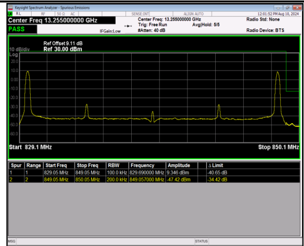
5-5-10MHz-10MHz-QPSK@QPSK-QPSK@QPSK-20501-20600-1RB#0@50RB#0-1RB#49@50RB#0-PASS
