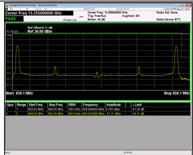
5-5-10MHz-10MHz-16QAM@16QAM-16QAM@16QAM-20501-20600-1RB#0@50RB#0-1RB#49@50RB#0-PASS
