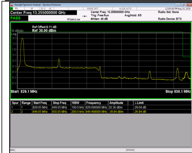
5-5-10MHz-10MHz-QPSK@QPSK-QPSK@QPSK-20501-20600-1RB#0@50RB#0-0RB#0@50RB#0-PASS
