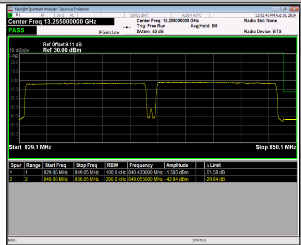
5-5-10MHz-10MHz-QPSK@QPSK-QPSK@QPSK-20501-20600-50RB#0@50RB#0-50RB#0@50RB#0-PASS
