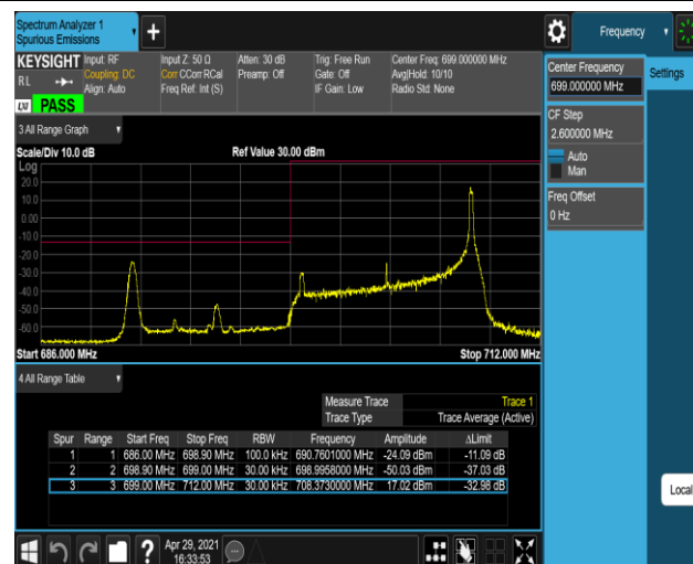
Band12-10MHz-16QAM-23130-1RB#0
