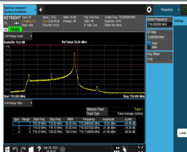
Band12-10MHz-16QAM-23130-1RB#49
