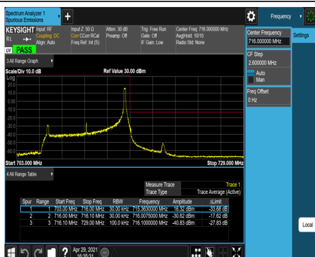
Band12-10MHz-QPSK-23130-1RB#49
