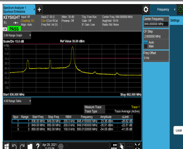
Band5-10MHz-QPSK-20600-1RB#49
