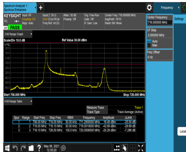
Band17-5MHz-QPSK-23825-25RB#0
