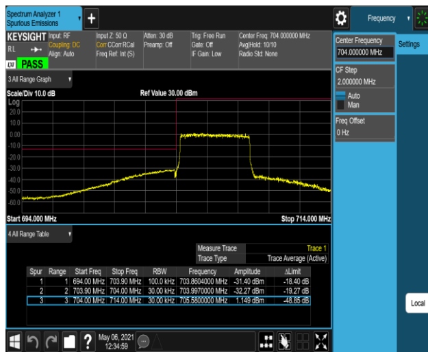
Band17-5MHz-16QAM-23825-1RB#24
