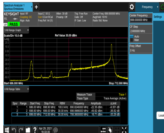
Band12-10MHz-QPSK-23130-1RB#0
