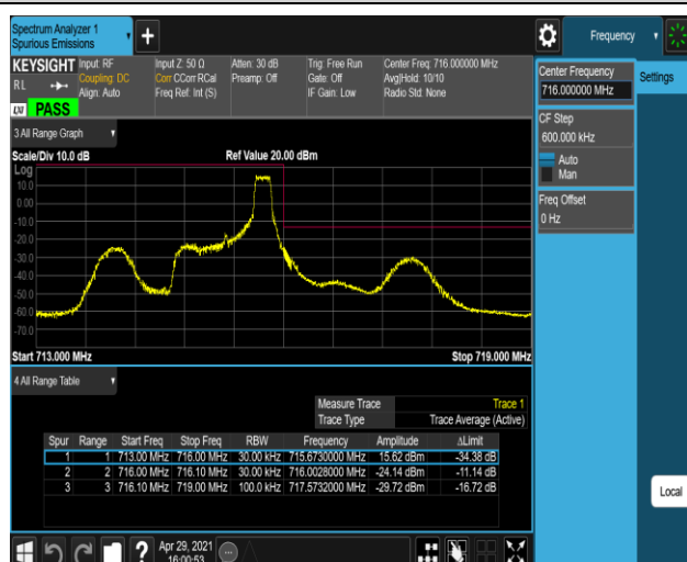
Band12-1.4MHz-16QAM-23173-1RB#5
