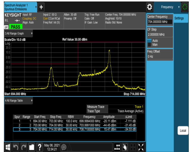
Band17-5MHz-16QAM-23825-1RB#0
