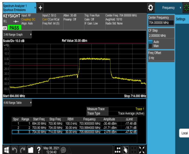
Band17-5MHz-QPSK-23825-1RB#24
