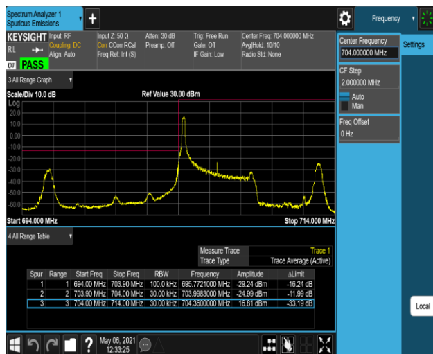
Band17-5MHz-QPSK-23755-25RB#0
