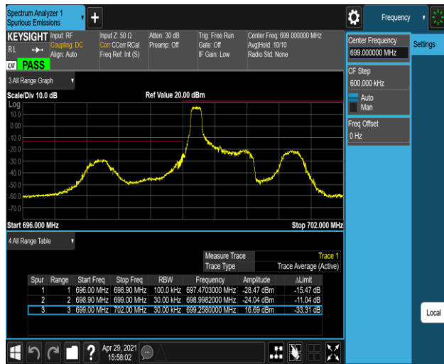
Band12-1.4MHz-QPSK-23017-6RB#0
