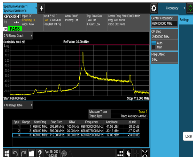
Band12-10MHz-QPSK-23060-50RB#0
