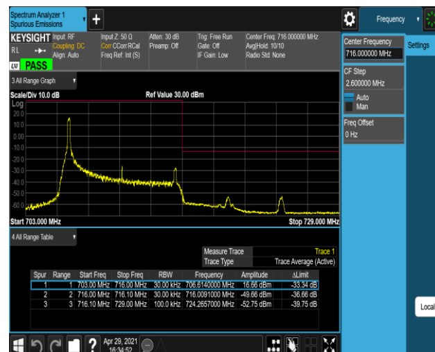
Band12-10MHz-QPSK-23130-50RB#0
