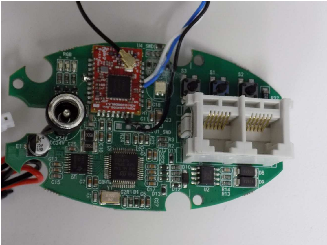
Figure 26: PCBA 1 Bottom
