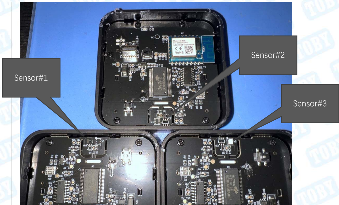
Photo 6 Appearance of PCB
