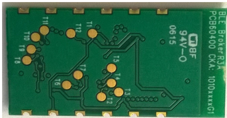
Bottom View
