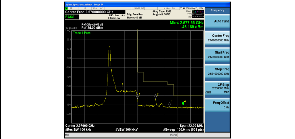
Band7-5MHz-16QAM-21425-1RB#24
