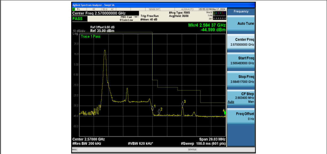
Band7-10MHz-16QAM-21400-1RB#49
