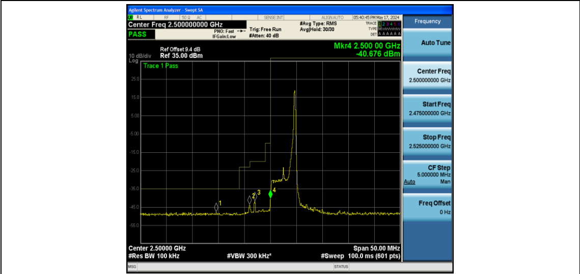
Band7-5MHz-QPSK-20775-25RB#0
