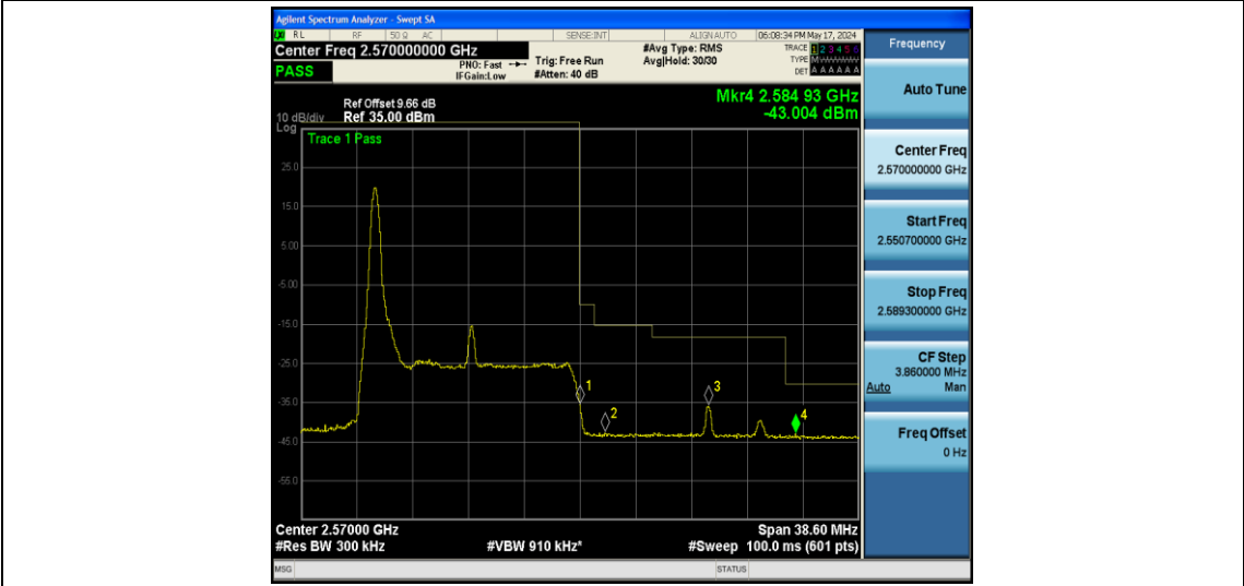
Band7-15MHz-QPSK-21375-1RB#74
