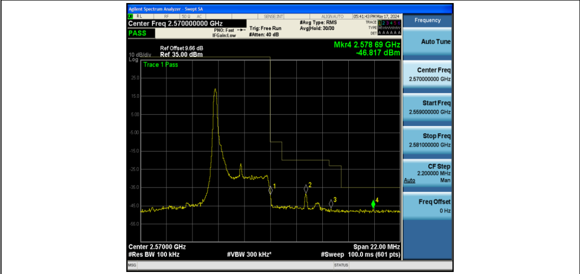
Band7-5MHz-QPSK-21425-1RB#24
