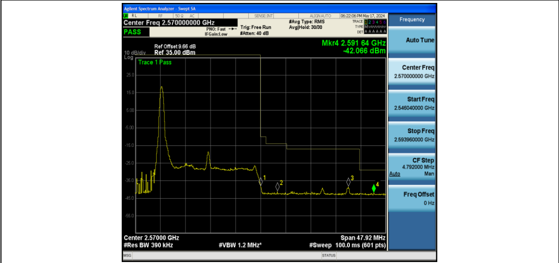
Band7-20MHz-16QAM-21350-1RB#99
