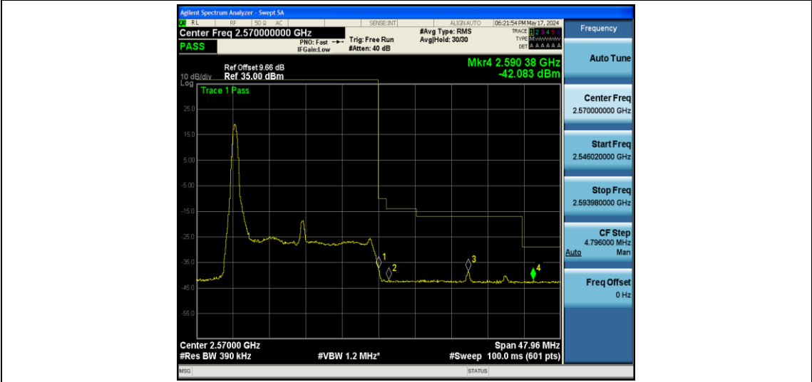
Band7-20MHz-QPSK-21350-1RB#99
