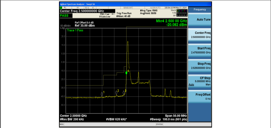
Band7-10MHz-16QAM-20800-1RB#49
