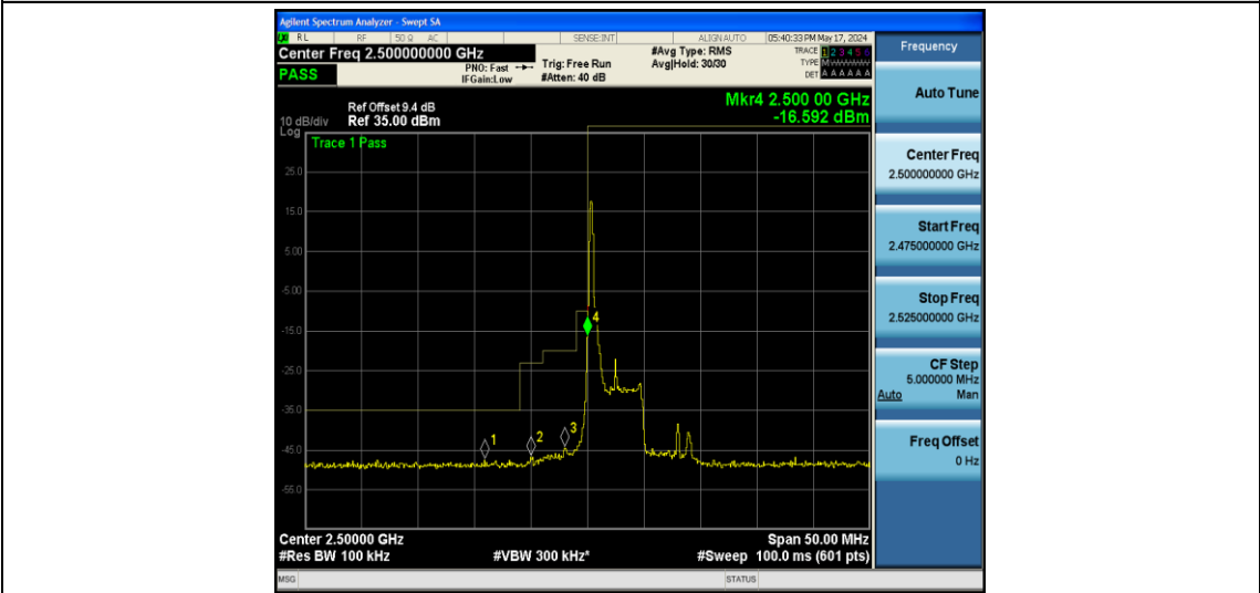
Band7-5MHz-16QAM-20775-1RB#24
