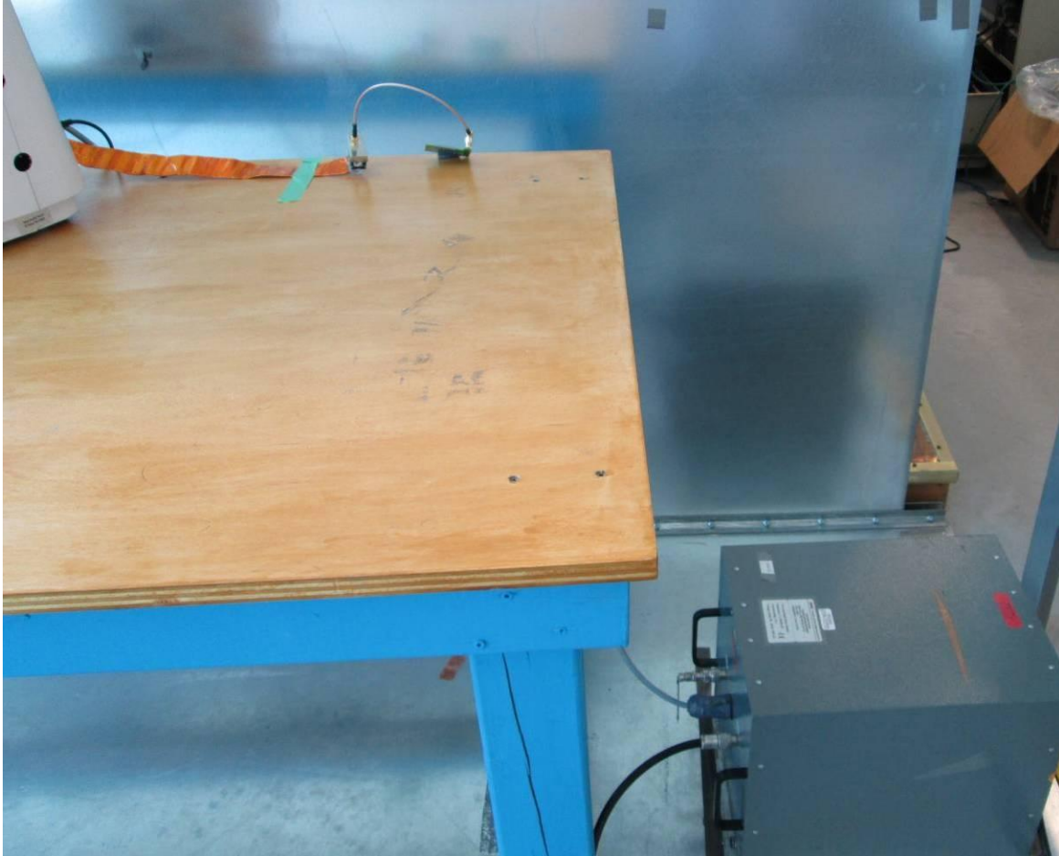
Conducted Emissions
