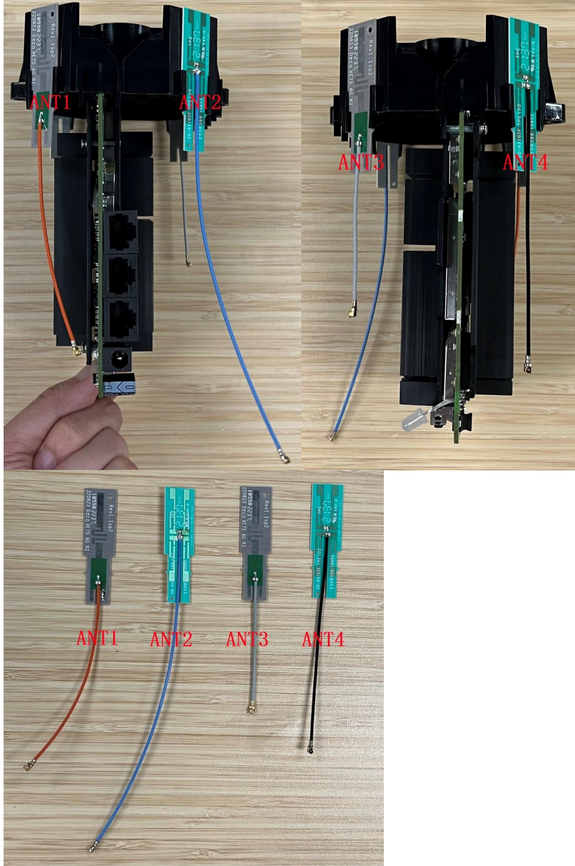
Internal View of EUT-23
