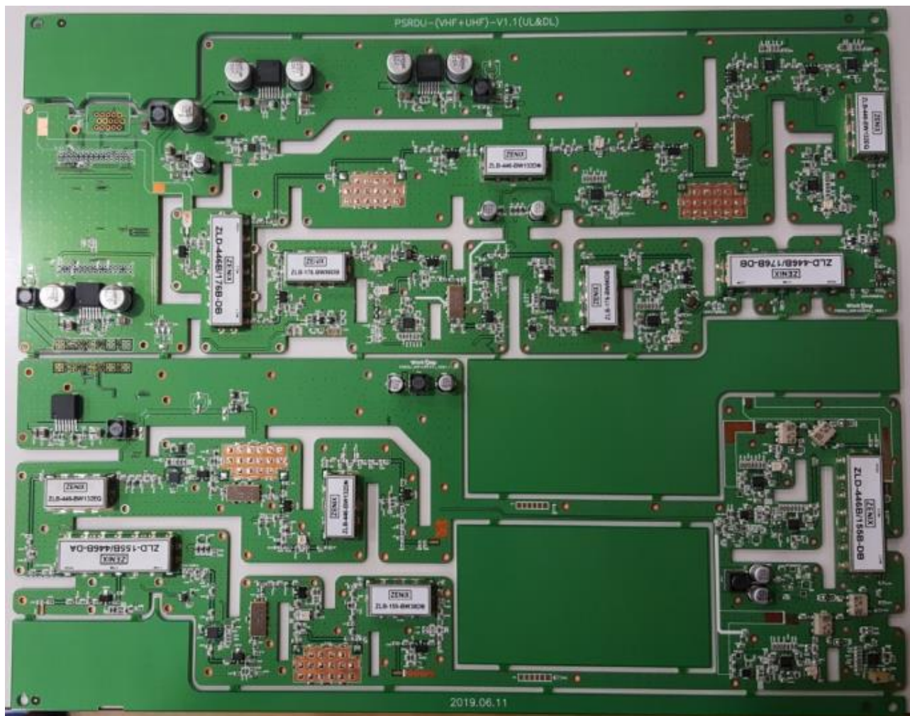
SMT (TOP)
