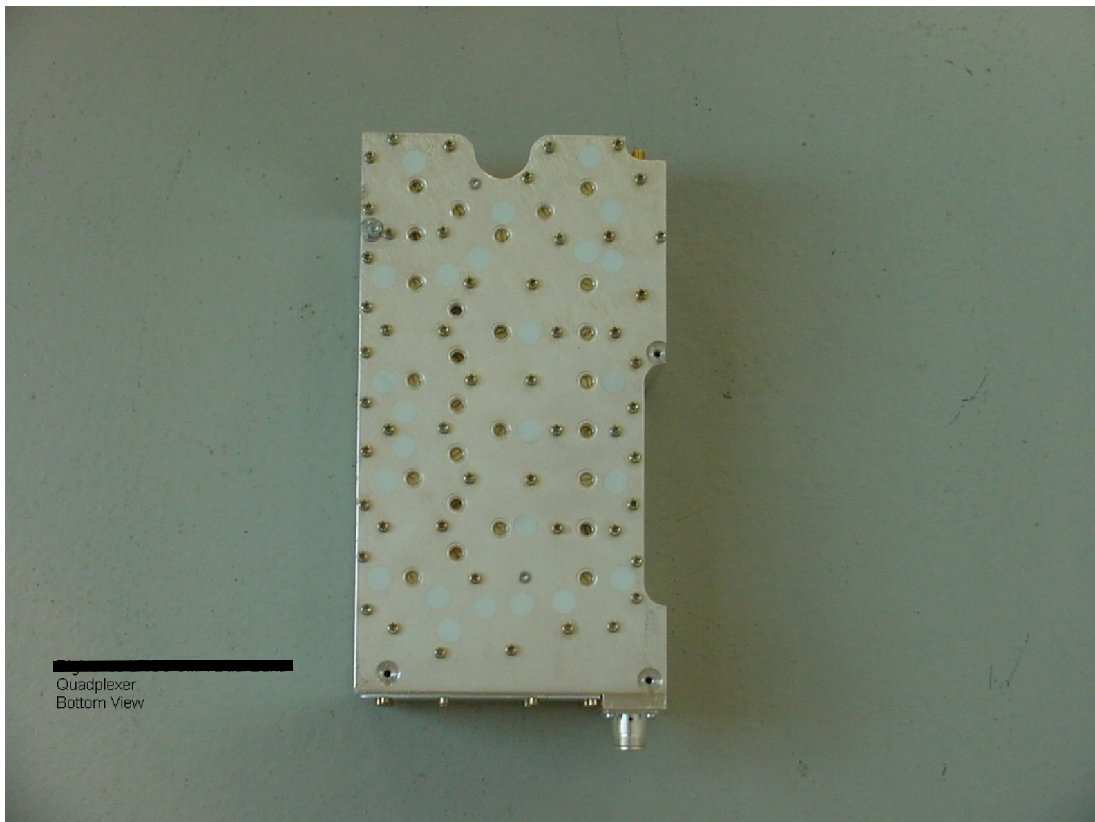
Digivance Street Coverage Solution (SCS) Quadplexer (a.k.a. Power Monitor/filter) Bottom View
