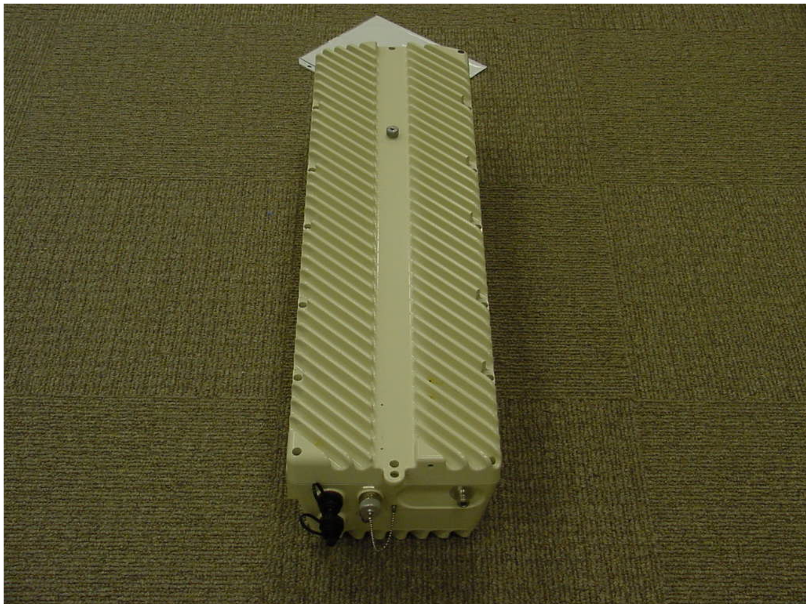
Digivance Street Coverage Solution Remote Unit Top View
