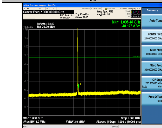
Band2_5MHz_QPSK_18900_1RB#0_1000~3000_1000~3000
