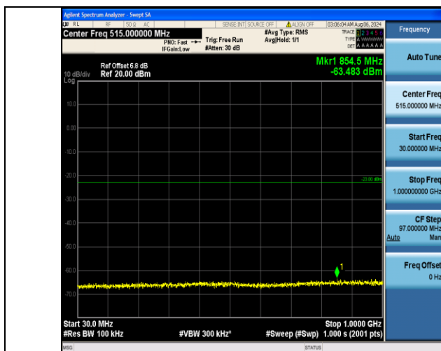
Band2_5MHz_QPSK_18625_25RB#0_30~1000_30~1000
