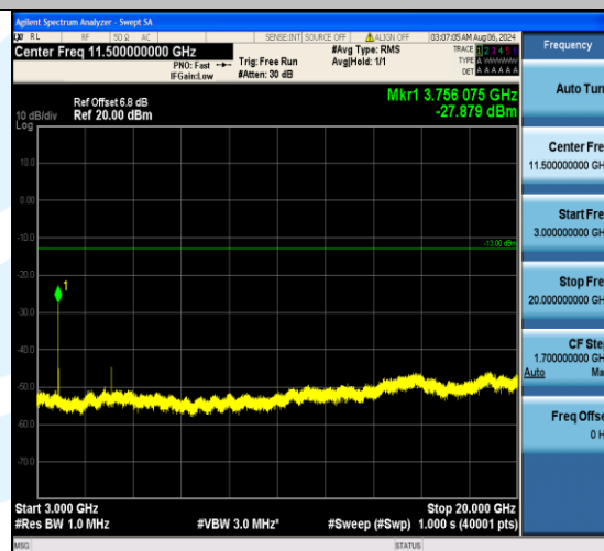
Band2_5MHz_QPSK_18900_1RB#0_3000~20000_3000~20000
