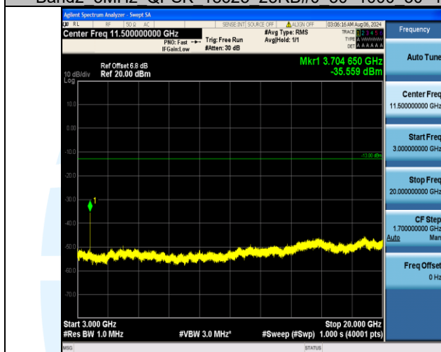
Band2_5MHz_QPSK_18625_25RB#0_3000~20000_3000~20000
