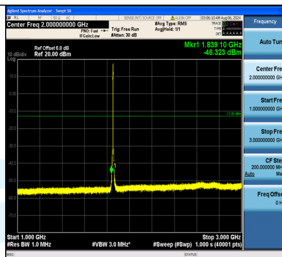
Band2_5MHz_QPSK_18625_25RB#0_1000~3000_1000~3000
