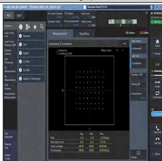
1-N12-PC3-15-15-M-8-CP-64QAM-Outer_Full-79@0-Ant1-see graph-PASS
