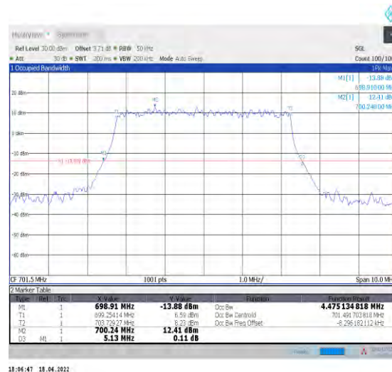
1-N12--15-5-L-4-DFT-64QAM-Outer_Full-25@0-Ant 1-4.475-5.130-≤5-PASS
