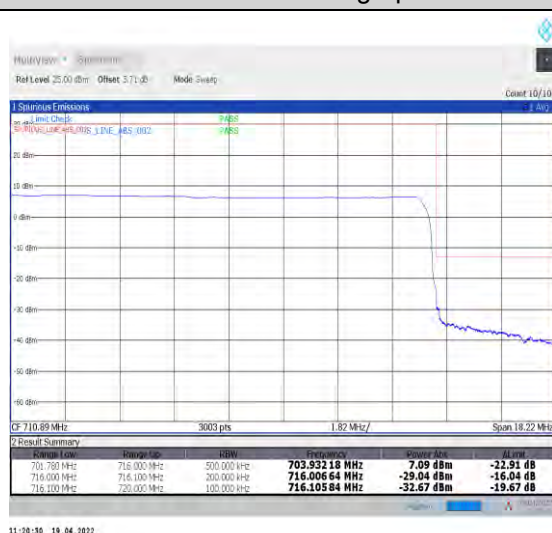
1-N12--15-15-H-6-CP-QPSK-Outer_Full-79@0-Ant1-PASS-see graph
