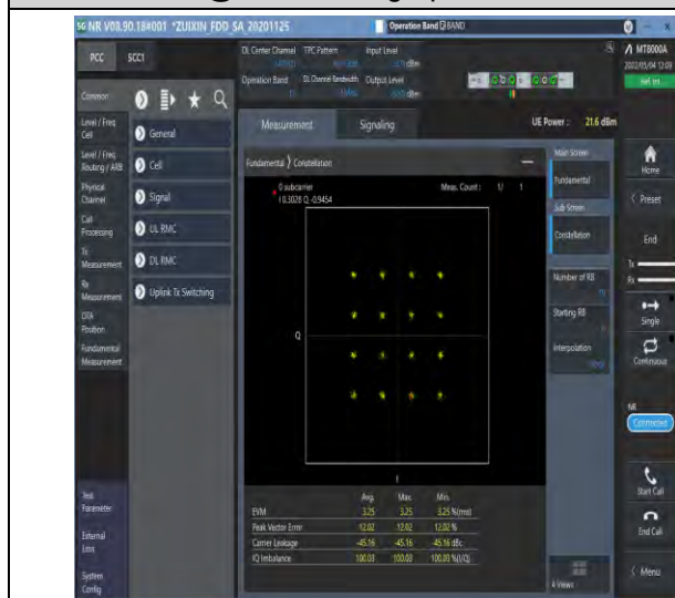
1-N12-PC3-15-15-M-7-CP-16QAM-Outer_Full-79@0-Ant1-see graph-PASS
