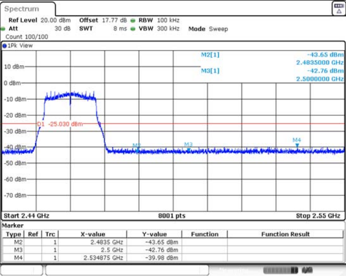
11G_Ant2_High_2462
