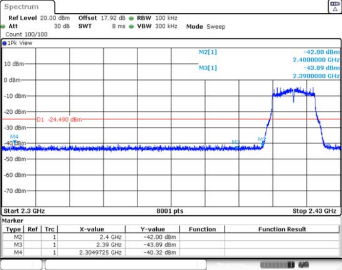
11G Ant2_Low_2412
