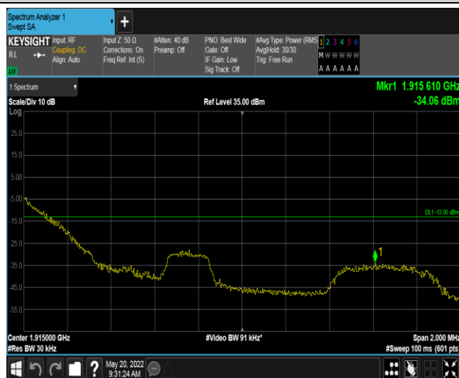
Band25-1.4MHz-16QAM-26683-1RB#0
