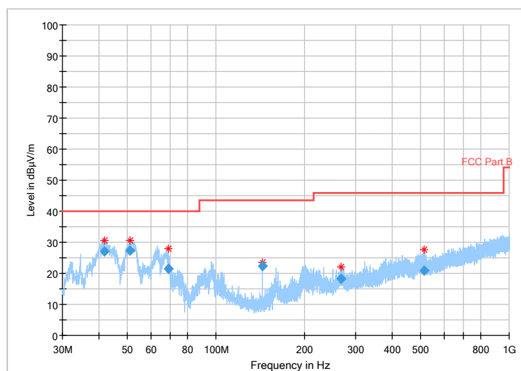
Fig 64. Radiated Spurious Emission (802.11g,Ch11,30MHz~1GHz)
