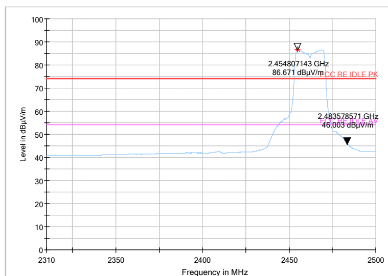
Fig 63. Radiated emission (Power): 802.11g, high channel
