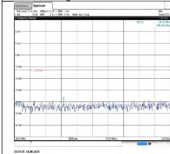
Band2-1.4MHz-16QAM-18900-1RB#0- Range1:30~1000MHz
