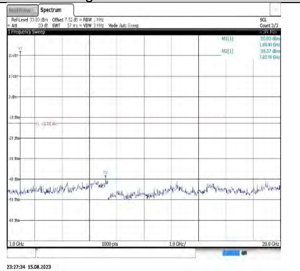
Band2-1.4MHz-16QAM-18900-1RB#0- Range2:1000~20000MHz
