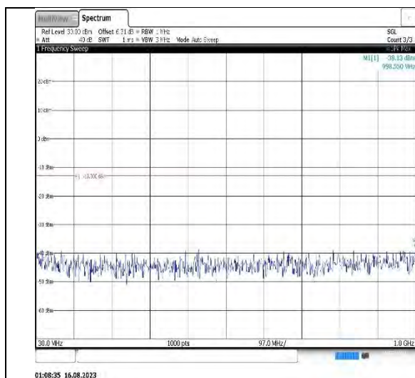
Band2-15MHz-16QAM-18900-1RB#0- Range1:30~1000MHz
