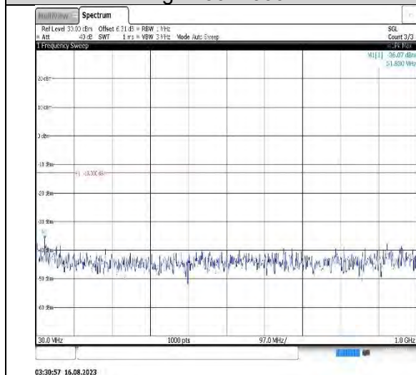
Band4-5MHz-QPSK-20175-1RB#0-Range1:30~1000MHz
