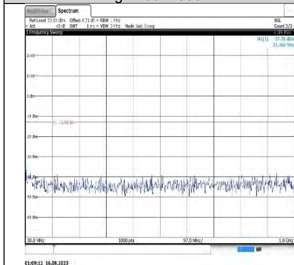
Band2-15MHz-16QAM-19125-1RB#0- Range1:30~1000MHz
