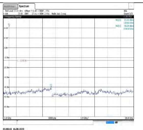
Band2-15MHz-16QAM-18900-1RB#0- Range2:1000~20000MHz
