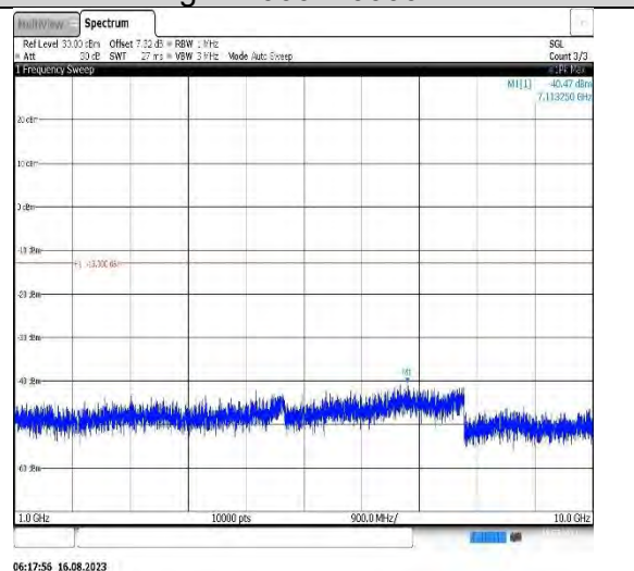
Band5-3MHz-QPSK-20525-1RB#0- Range2:1000~10000MHz
