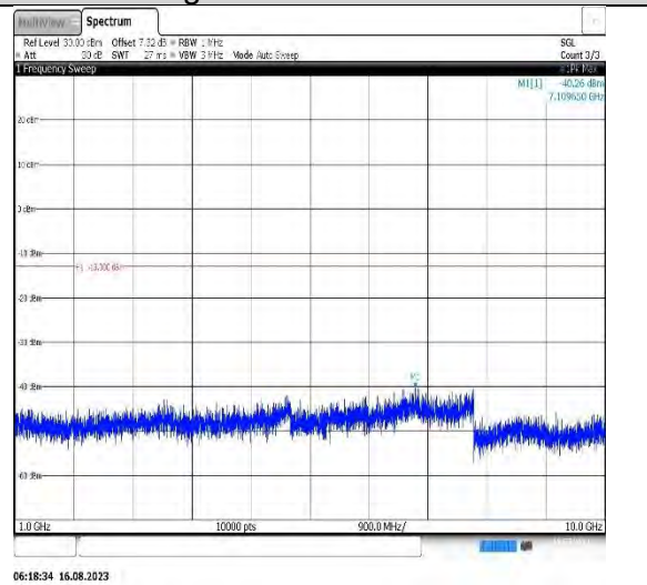
Band5-3MHz-QPSK-20525-1RB#0- Range2:1000~10000MHz
