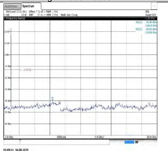
Band2-15MHz-16QAM-19125-1RB#0- Range2:1000~20000MHz
