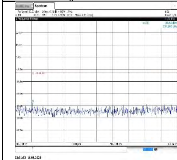
Band4-5MHz-QPSK-20175-1RB#0-Range1:30~1000MHz
