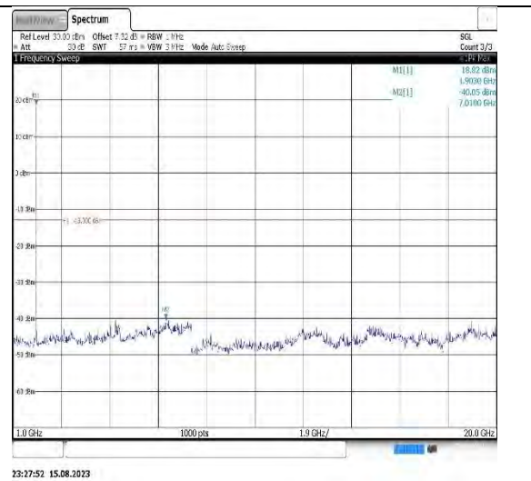
Band2-1.4MHz-16QAM-18607-1RB#0- Range2:1000~20000MHz
