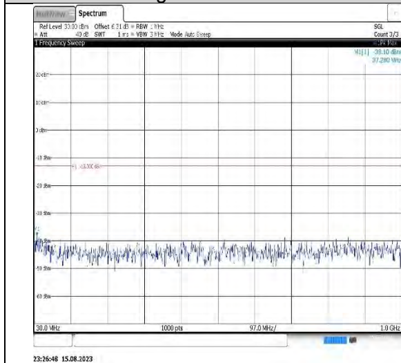
Band2-1.4MHz-16QAM-18900-1RB#0- Range1:30~1000MHz
