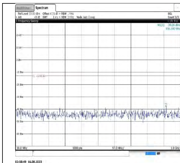
Band4-5MHz-QPSK-19975-1RB#0-Range1:30~1000MHz
