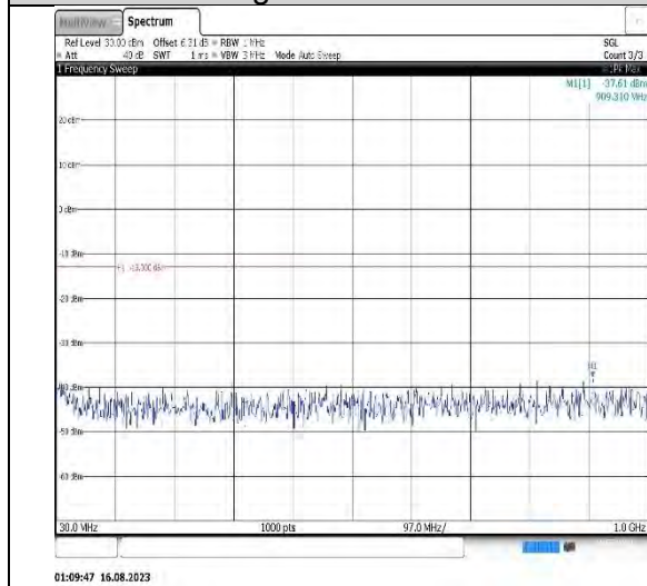
Band2-15MHz-16QAM-19125-1RB#0- Range1:30~1000MHz
