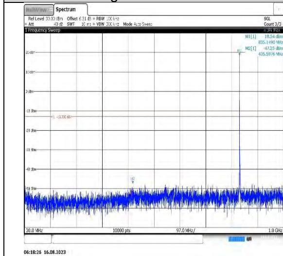
Band5-3MHz-QPSK-20525-1RB#0- Range1:30~1000MHz
