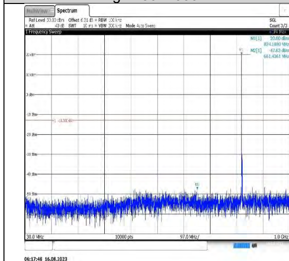
Band5-3MHz-QPSK-20525-1RB#0- Range1:30~1000MHz
