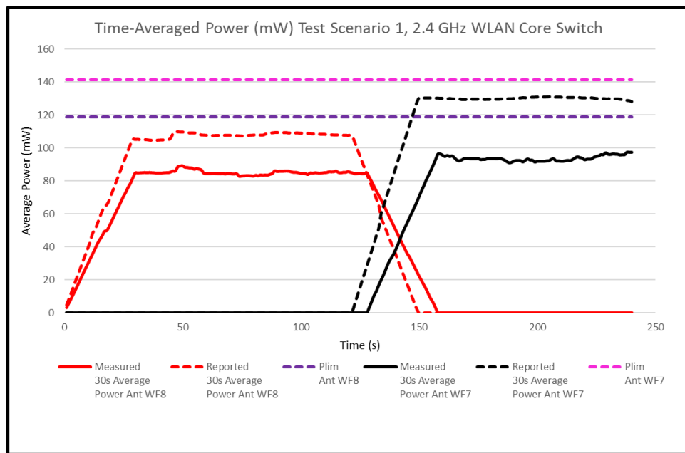
Figure H-2 30s Average Power vs. Time, 2.4 GHz
