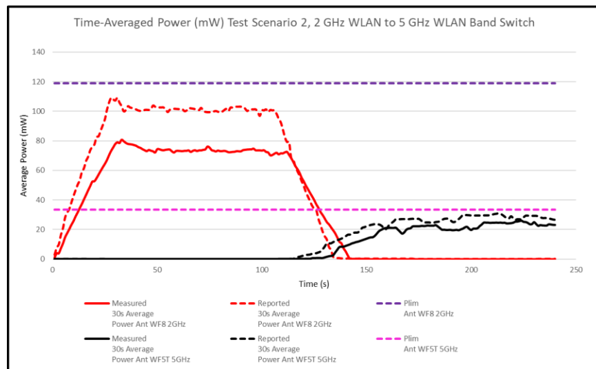
Figure H-8 30s Average Power vs. Time during Band Switch
