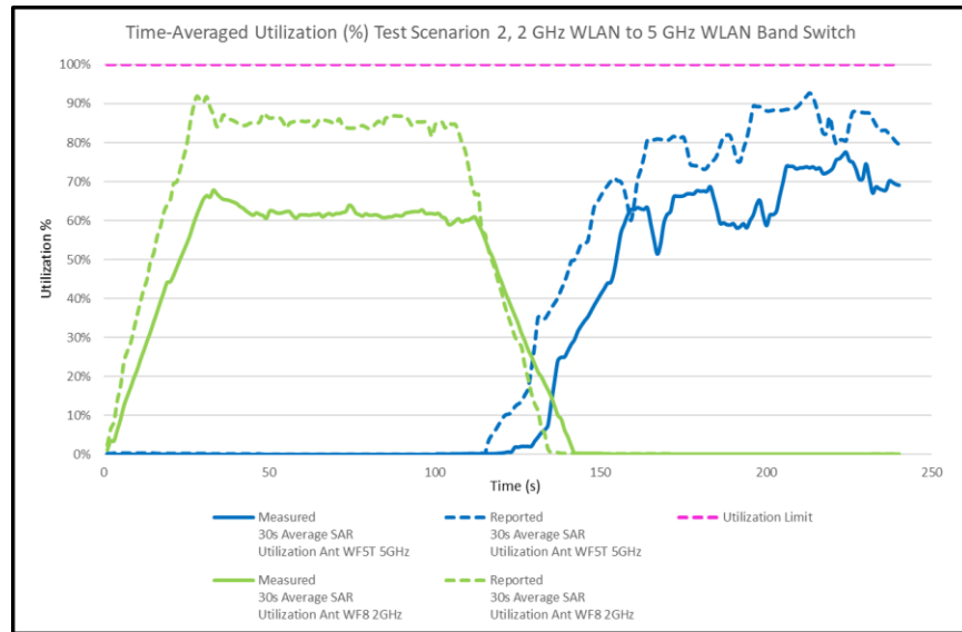
Figure H-7 30s Average Utilization vs. Time during Band Switch
