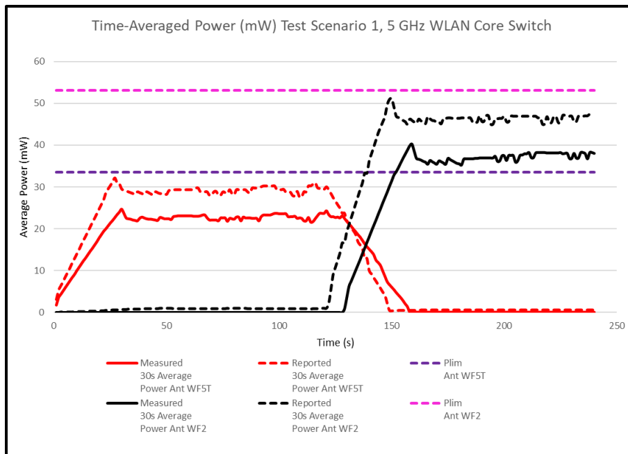
Figure H-4 30s Average Power vs. Time, 5 GHz
