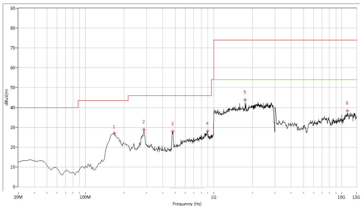
(Plot B: 30MHz – 13GHz, Test Antenna Horizontal)
