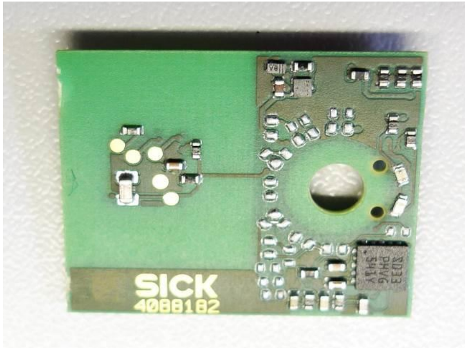
Photo 7: PCB 3 back side view
