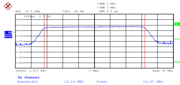
Mode: TX 11ax HT20 channel 6
