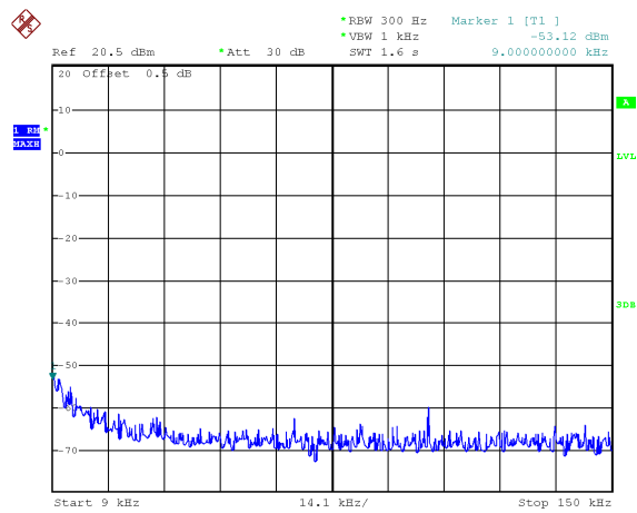
Mode: TX 11ax HT20 channel 3
