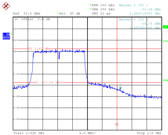
TX 11 ax HT20: Band edge-right side
