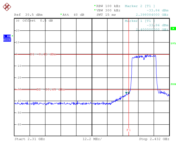
TX 11ax HT20: Band edge-left side
