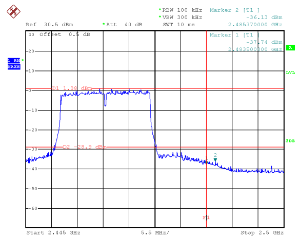
TX 11 ax HT20: Band edge-right side
