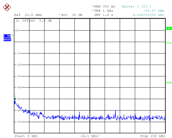
Mode: TX 11 ax HT20 channel 9
