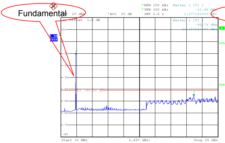
Mode: TX 11 ax HT20 channel 3
