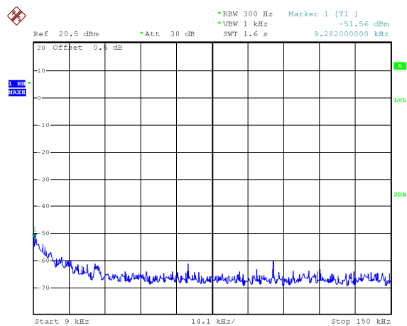
Mode: TX 11 ax HT20 channel 9
