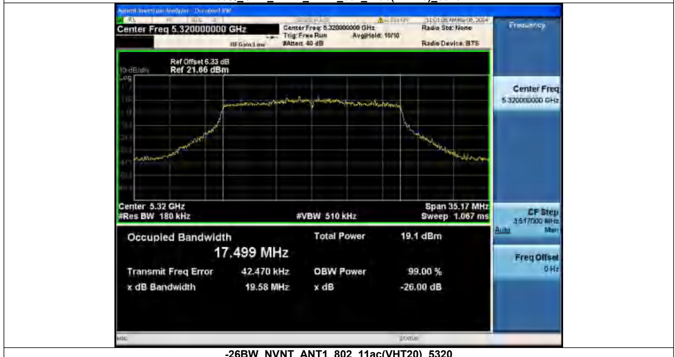
-26BW_NVNT_ANT1_802_11ac(VHT20)_5320
