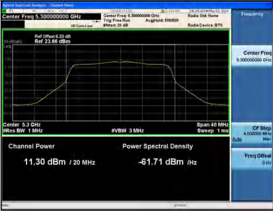
Maximum_Conducted_Output_Power_NVNT_ANT2_802_11ac(VHT20)_5300_20M
