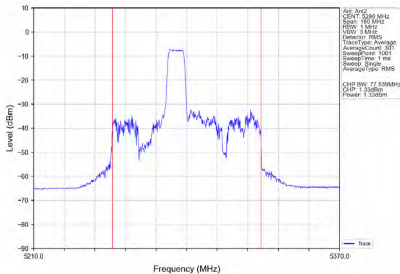
802.11ax(HE80) MCH 5290MHz RU106 Mid Ant2 NTNv
