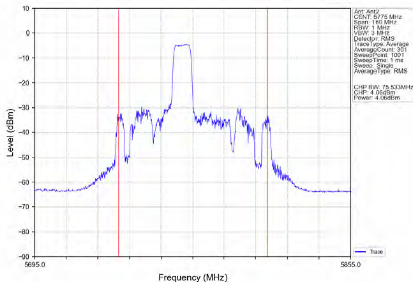
802.11ax(HE80) MCH 5775MHz RU106 Mid Ant2 NTNv
