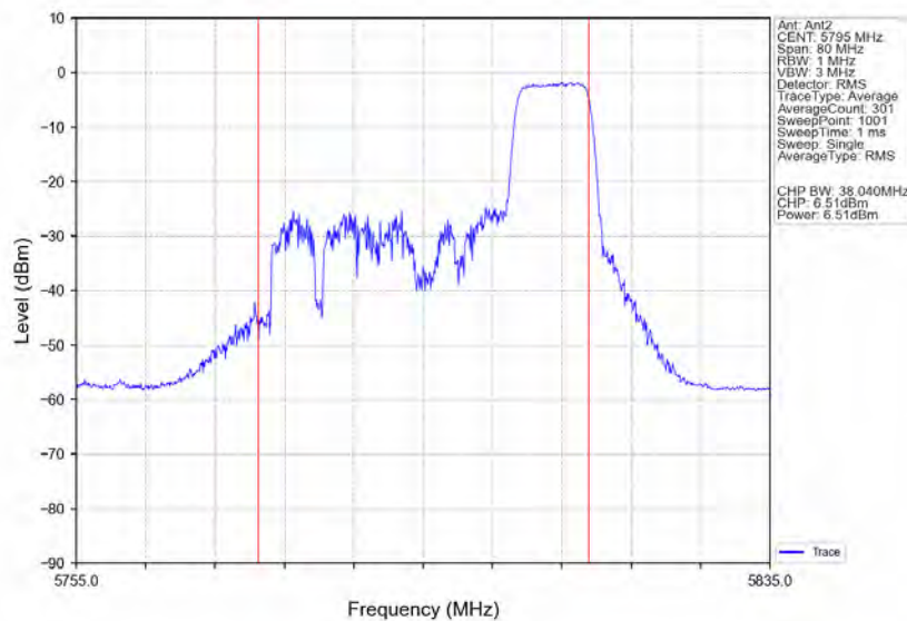
802.11ax(HE40) HCH 5795MHz RU106 Right Ant2 NTVN
