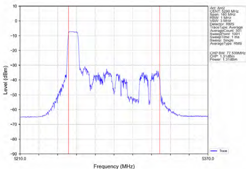
802.11ax(HE80) MCH 5290MHz RU106 Left Ant2 NTN
