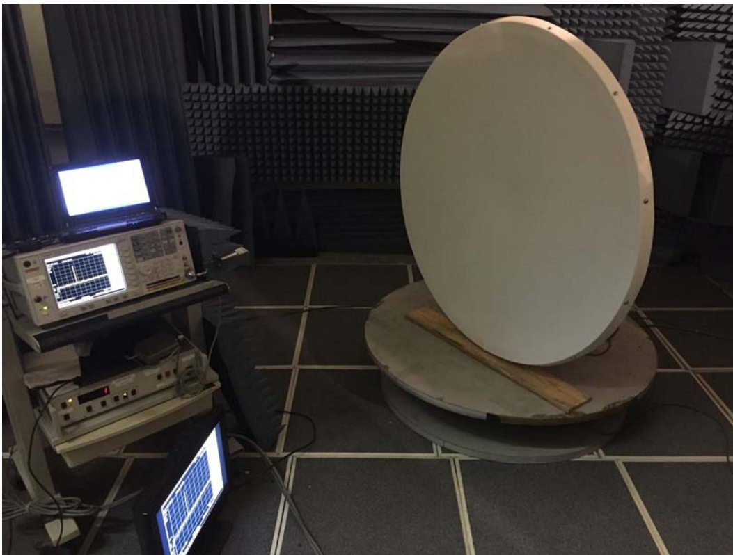
Radiated Emissions: 18 to 26.5 GHz, Front
