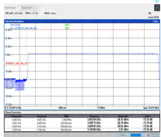
1-N78-3700-3800-PASS-30-60-L-6-CP-QPSK-Outer_Full-162@0-Ant1-1--PASS-see graph
