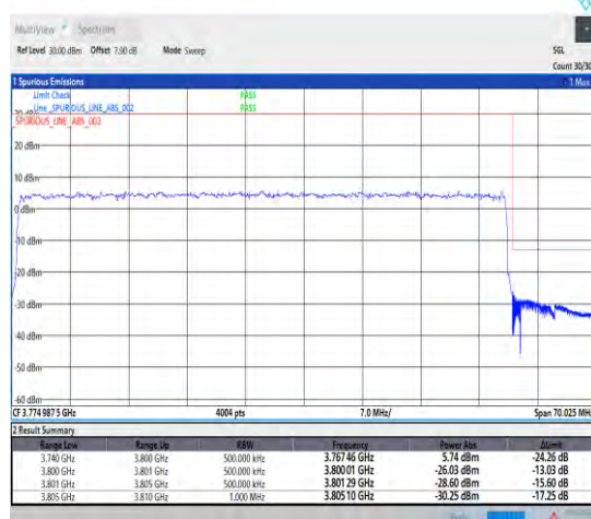
1-N78-3700-3800-PASS-30-60-H-6-CP-QPSK-Outer_Full-162@0-Ant1-1--PASS-see graph
