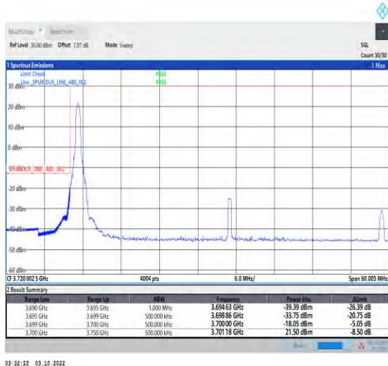
1-N78-3700-3800-PASS-30-50-L-4-CP-QPSK-Edge_1RB_Left-1@0-Ant1-1--PASS-see graph
