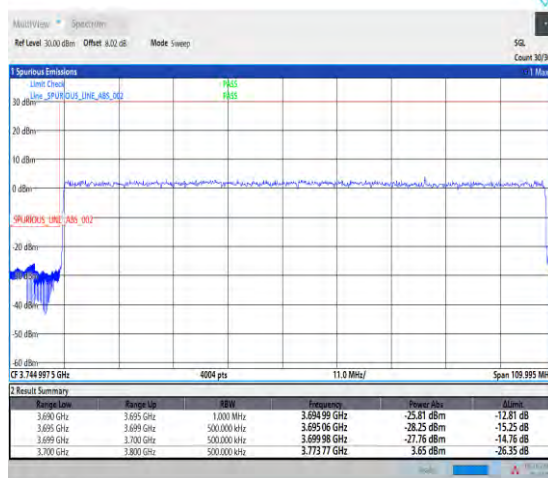
1-N78-3700-3800-PASS-30-100-L-3-DFT-PI2BPSK-K-Outer_Full-270@0-Ant1-1--PASS-see graph
