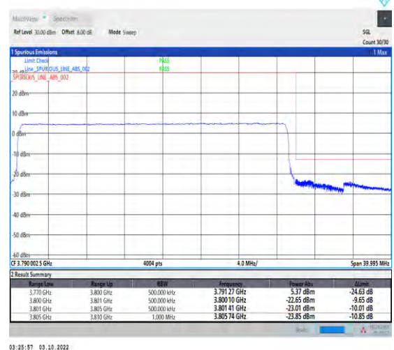
1-N78-3700-3800-PASS-30-30-H-6-CP-QPSK-Outer_Full-78@0-Ant1-1--PASS-see graph
