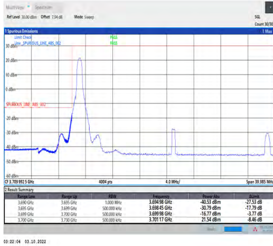
1-N78-3700-3800-PASS-30-30-L-1-DFT-PI2BPSK-Edge_1RB_Left-1@0-Ant1-1--PASS-see graph
