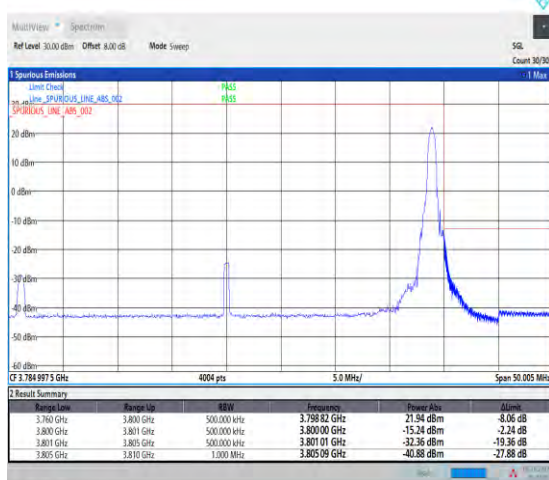
1-N78-3700-3800-PASS-30-40-H-5-CP-QPSK-Edge_1RB_Right-1@105-Ant1-1--PASS-see graph
