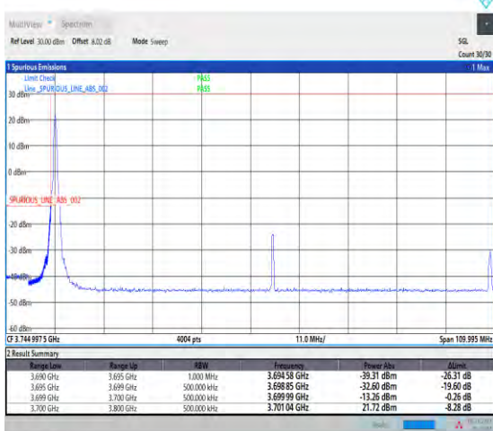
1-N78-3700-3800-PASS-30-100-L-4-CP-QPSK-Edge_1RB_Left-1@0-Ant1-1--PASS-see graph
