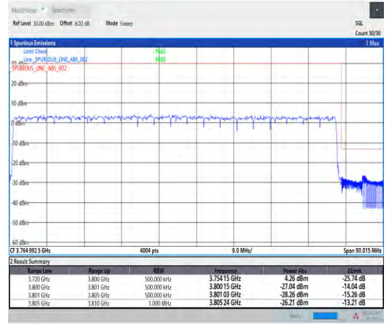
1-N78-3700-3800-PASS-30-80-H-3-DFT-PI2BPSK-Outer_Full-216@0-Ant1-1--PASS-see graph
