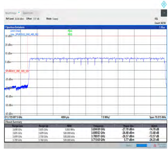
1-N78-3700-3800-PASS-30-60-L-3-DFT-PI2BPSK-Outer_Full-162@0-Ant1-1--PASS-see graph
