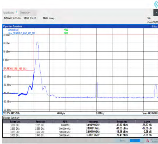
1-N78-3700-3800-PASS-30-40-L-1-DFT-PI2BPSK-Edge_1RB_Left-1@0-Ant1-1--PASS-see graph
