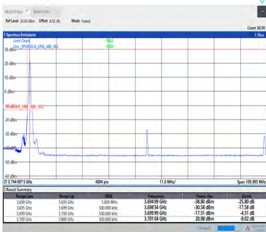
1-N78-3700-3800-PASS-30-100-L-1-DFT-PI2BPSK-Edge_1RB_Left-1@0-Ant1-1--PASS-see graph
