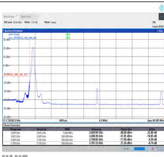
1-N78-3700-3800-PASS-30-50-L-1-DFT-PI2BPSK-Edge_1RB_Left-1@0-Ant1-1--PASS-see graph
