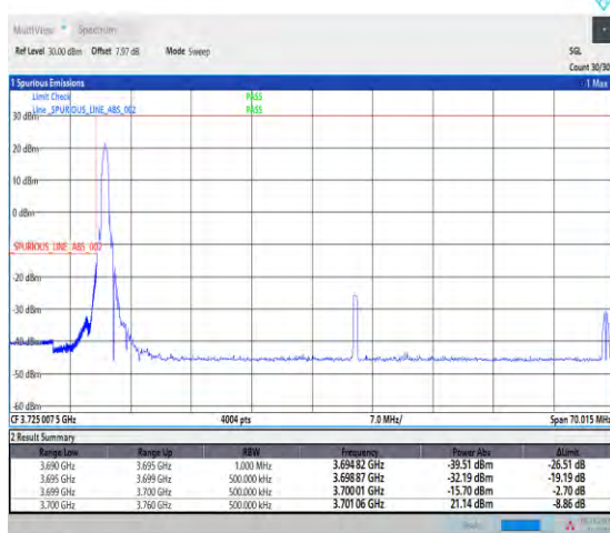
1-N78-3700-3800-PASS-30-60-L-4-CP-QPSK-Edge_1RB_Left-1@0-Ant1-1--PASS-see graph
