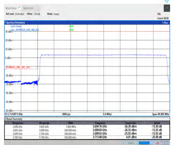
1-N78-3700-3800-PASS-30-40-L-6-CP-QPSK-Outer_Full-106@0-Ant1-1--PASS-see graph
