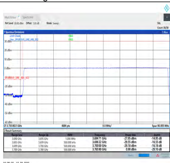
1-N78-3700-3800-PASS-30-80-L-3-DFT-PI2BPSK-Outer_Full-216@0-Ant1-1--PASS-see graph
