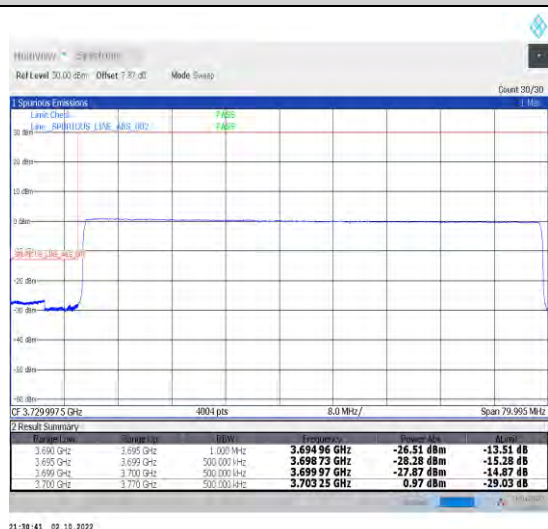
1-N78-3700-3800-PASS-30-70-L-6-CP-QPSK-Outer_Full-189@0-Ant1-1--PASS-see graph
