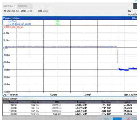
1-N78-3700-3800-PASS-30-60-H-3-DFT-PI2BPSK-Outer_Full-162@0-Ant1-1--PASS-see graph
