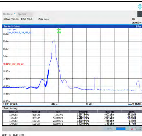
1-N78-3700-3800-PASS-30-20-L-1-DFT-PI2BPSK-Edg_e_1RB_Left-1@0-Ant1-1--PASS-see graph
