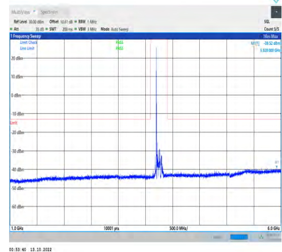
1-N78-3700-3800-PC2-30-100-H-1-DFT-PI2BPSK-I nner_1RB_Left-1@1-1000-6000-Ant1-5404.50--39.94--13-PASS
