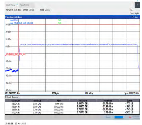
1-N78-3700-3800-PASS-30-90-L-6-CP-QPSK-Outer_Full-245@0-Ant1-1--PASS-see graph
