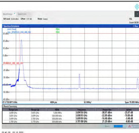
1-N78-3700-3800-PASS-30-70-L-4-CP-QPSK-Edge_1RB_Left-1@0-Ant1-1--PASS-see graph
