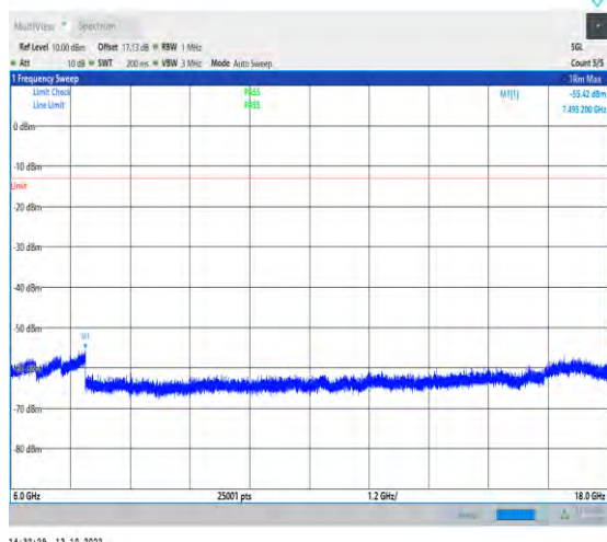
1-N78-3700-3800-PC2-30-100-L-1-DFT-PI2BPSK-Inner_1RB_Left-1@1-6000-18000-Ant1-7495.20--55.4 2--13-PASS
