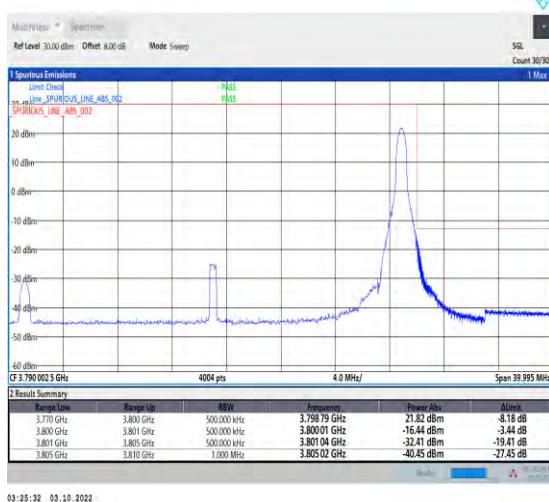
1-N78-3700-3800-PASS-30-30-H-5-CP-QPSK-Edge_1RB_Right-1@77-Ant1-1--PASS-see graph
