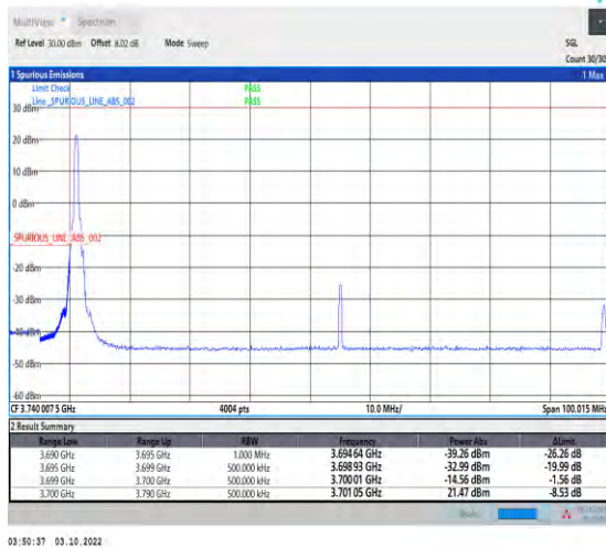
1-N78-3700-3800-PASS-30-90-L-4-CP-QPSK-Edge_1RB_Left-1@0-Ant1-1--PASS-see graph
