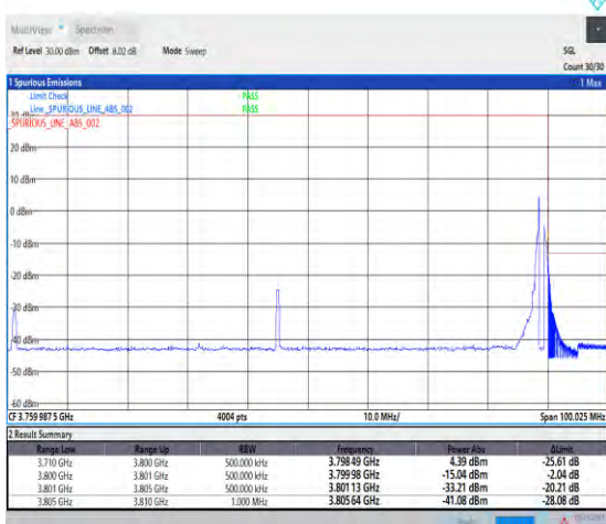
1-N78-3700-3800-PASS-30-90-H-5-CP-QPSK-Edge_1RB_Right-1@244-Ant1-1--PASS-see graph
