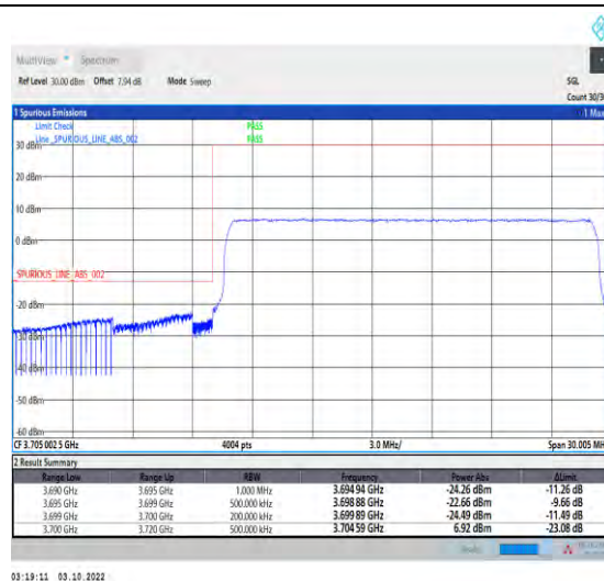
1-N78-3700-3800-PASS-30-20-L-3-DFT-PI2BPSK-Outer_Full-50@0-Ant1-1--PASS-see graph
