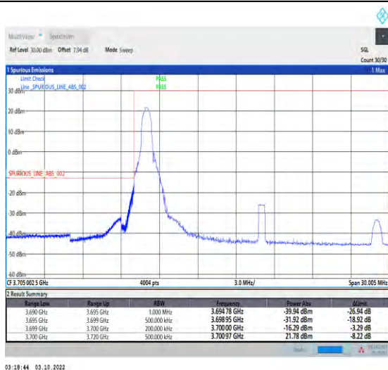
1-N78-3700-3800-PASS-30-20-L-4-CP-QPSK-Edge_1RB_Left-1@0-Ant1-1--PASS-see graph
