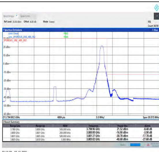
1-N78-3700-3800-PASS-30-20-H-2-DFT-PI2BPSK-Edge_1RB_Right-1@50-Ant1-1--PASS-see graph
