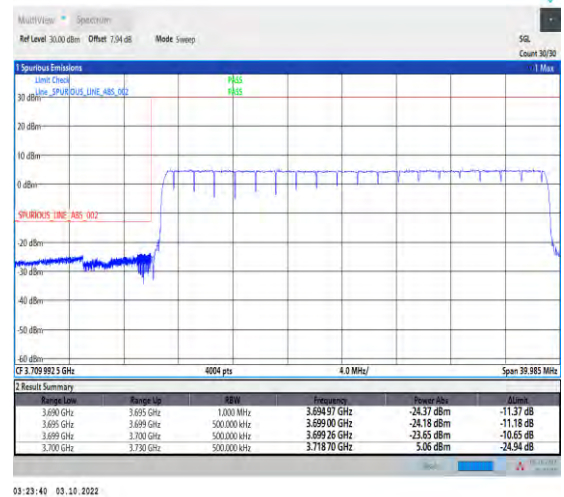
1-N78-3700-3800-PASS-30-30-L-6-CP-QPSK-Outer_Full-78@0-Ant1-1--PASS-see graph
