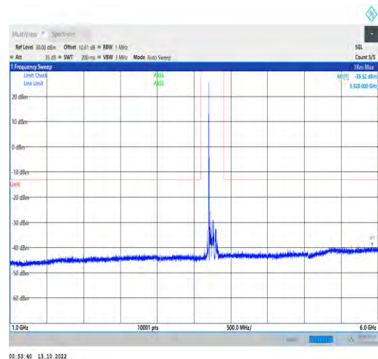
1-N78-3700-3800-PC2-30-100-L-1-DFT-PI2BPSK-Inn er_1RB_Left-1@1-1000-6000-Ant1-5896.50--40.17-- 13-PASS
