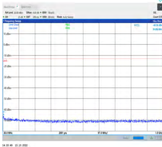
1-N78-3700-3800-PC2-30-100-H-1-DFT-PI2BPSK-I nner_1RB_Left-1@1-30-1000-Ant1-34.85--65.58--13-PASS
