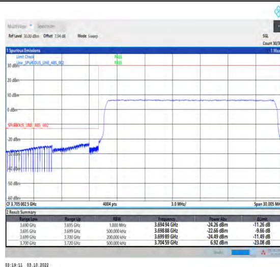
1-N78-3700-3800-PASS-30-20-L-6-CP-QPSK-Outer_Full-51@0-Ant1-1--PASS-see graph
