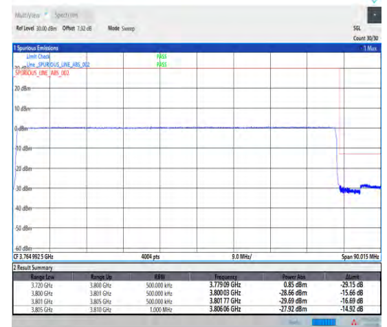
1-N78-3700-3800-PASS-30-80-H-6-CP-QPSK-Outer_Full-217@0-Ant1-1--PASS-see graph
