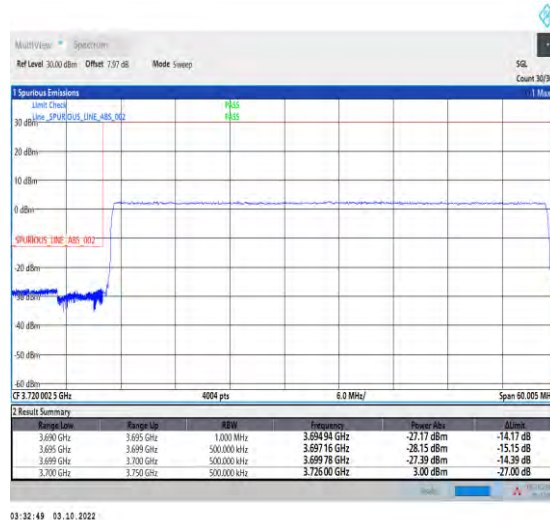
1-N78-3700-3800-PASS-30-50-L-6-CP-QPSK-Outer_Full-133@0-Ant1-1--PASS-see graph
