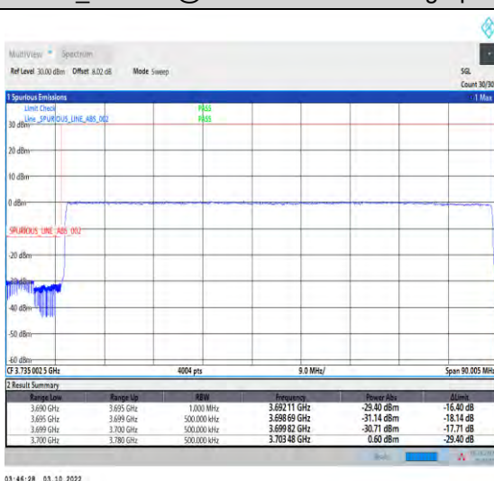
1-N78-3700-3800-PASS-30-80-L-6-CP-QPSK-Outer_Full-217@0-Ant1-1--PASS-see graph
