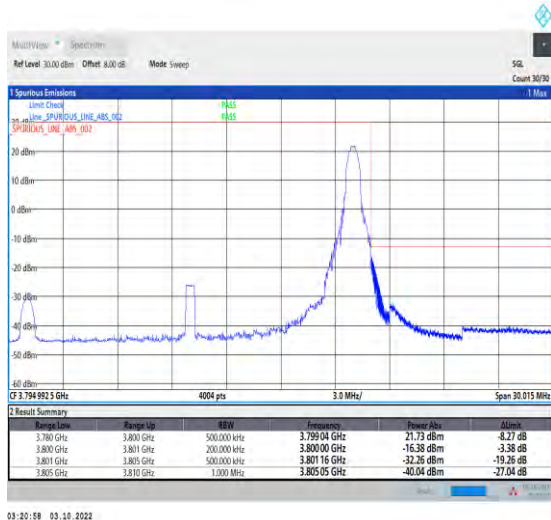
1-N78-3700-3800-PASS-30-20-H-5-CP-QPSK-Edge_1RB_Right-1@50-Ant1-1--PASS-see graph
