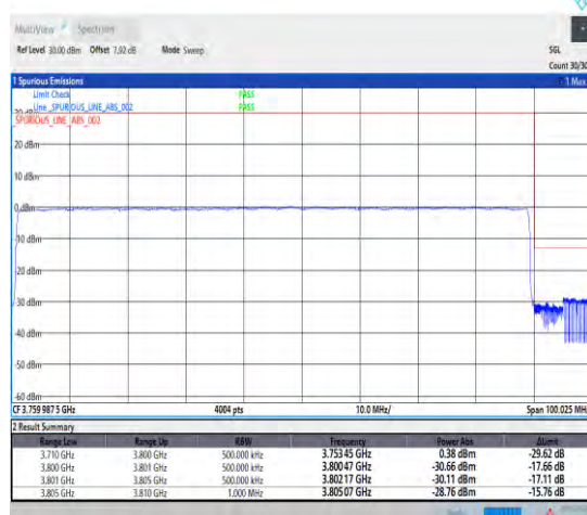
1-N78-3700-3800-PASS-30-90-H-6-CP-QPSK-Outer_Full-245@0-Ant1-1--PASS-see graph
