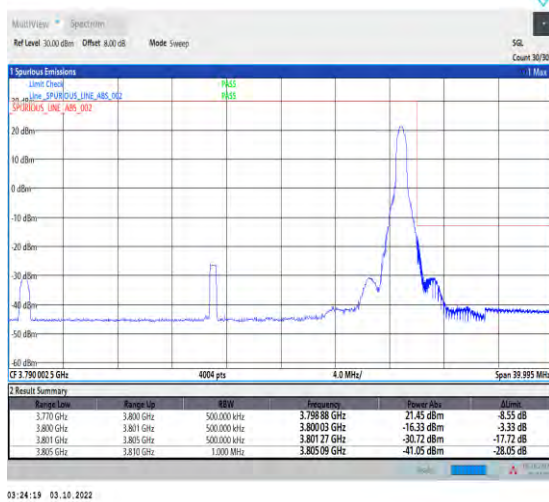
1-N78-3700-3800-PASS-30-30-H-2-DFT-PI2BPSK-Edge_1RB_Right-1@77-Ant1-1--PASS-see graph
