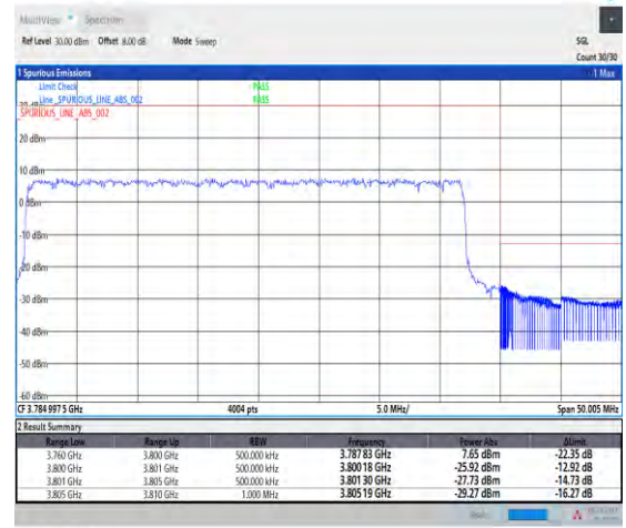
1-N78-3700-3800-PASS-30-40-H-3-DFT-PI2BPSK-Outer_Full-100@0-Ant1-1--PASS-see graph
