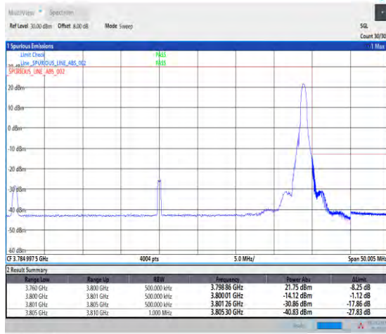
1-N78-3700-3800-PASS-30-40-H-2-DFT-PI2BPSK-Edge_1RB_Right-1@105-Ant1-1--PASS-see graph
