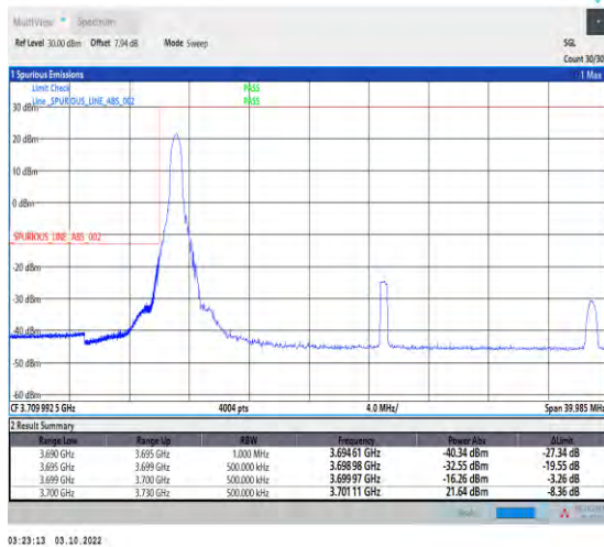
1-N78-3700-3800-PASS-30-30-L-4-CP-QPSK-Edge_1RB_Left-1@0-Ant1-1--PASS-see graph
