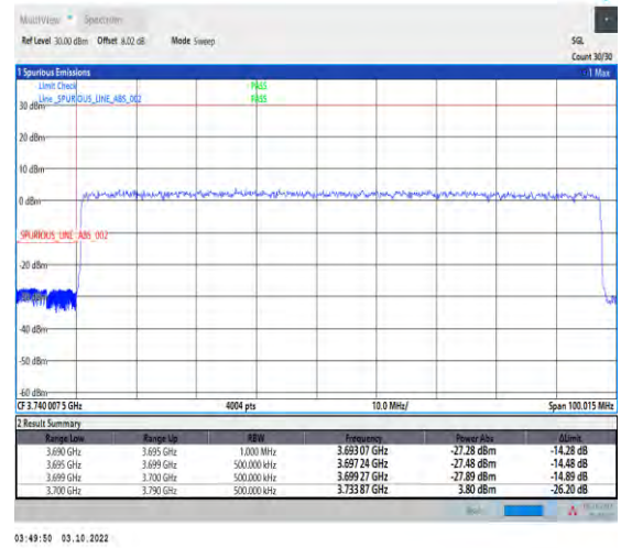
1-N78-3700-3800-PASS-30-90-L-3-DFT-PI2BPSK-Outer_Full-240@0-Ant1-1--PASS-see graph
