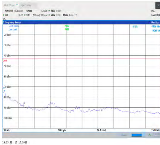
1-N78-3700-3800-PC2-30-100-H-1-DFT-PI2BPSK-I nner_1RB_Left-1@1-0.009-0.15-Ant1-0.01--74.59--43-PASS
