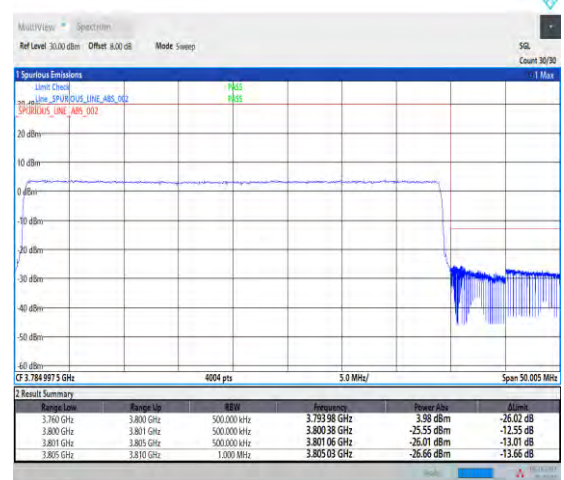
1-N78-3700-3800-PASS-30-40-H-6-CP-QPSK-Outer_Full-106@0-Ant1-1--PASS-see graph
