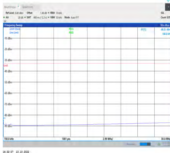
1-N78-3700-3800-PC2-30-100-L-1-DFT-PI2BPSK-Inn er_1RB_Left-1@1-0.15-30-Ant1-0.15--86.31--33-PAS S
