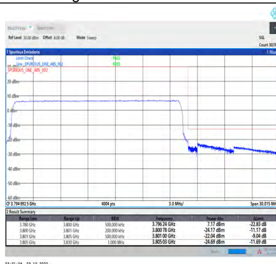
1-N78-3700-3800-PASS-30-20-H-3-DFT-PI2BPSK-Outer_Full-50@0-Ant1-1--PASS-see graph
