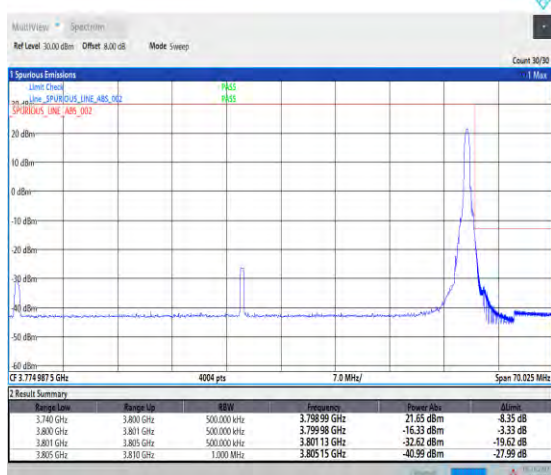
1-N78-3700-3800-PASS-30-60-H-5-CP-QPSK-Edge_1RB_Right-1@161-Ant1-1--PASS-see graph
