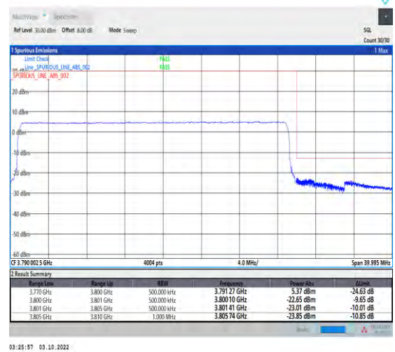
1-N78-3700-3800-PASS-30-30-H-3-DFT-PI2BPSK-Outer_Full-75@0-Ant1-1--PASS-see graph
