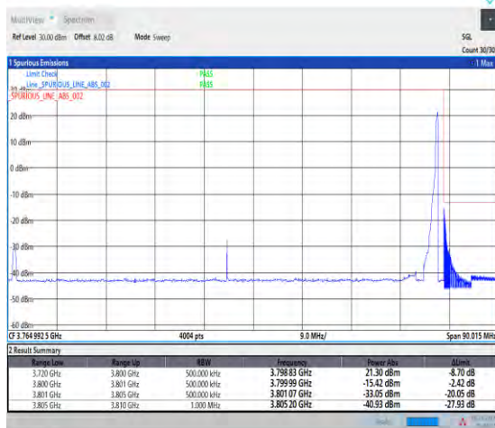
1-N78-3700-3800-PASS-30-80-H-5-CP-QPSK-Edge_1RB_Right-1@216-Ant1-1--PASS-see graph
