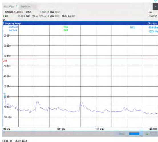
1-N78-3700-3800-PC2-30-100-L-1-DFT-PI2BPSK-In ner_1RB_Left-1@1-0.009-0.15-Ant1-0.01--80.60--4 3-PASS
