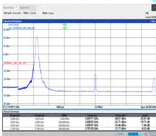
1-N78-3700-3800-PASS-30-40-L-4-CP-QPSK-Edge_1RB_Left-1@0-Ant1-1--PASS-see graph
