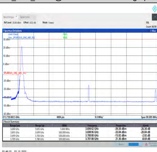
1-N78-3700-3800-PASS-30-80-L-4-CP-QPSK-Edge_1RB_Left-1@0-Ant1-1--PASS-see graph
