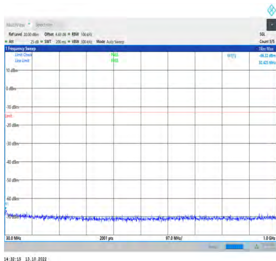
1-N78-3700-3800-PC2-30-100-L-1-DFT-PI2BPSK-In ner_1RB_Left-1@1-30-1000-Ant1-32.43--66.32--13- PASS
