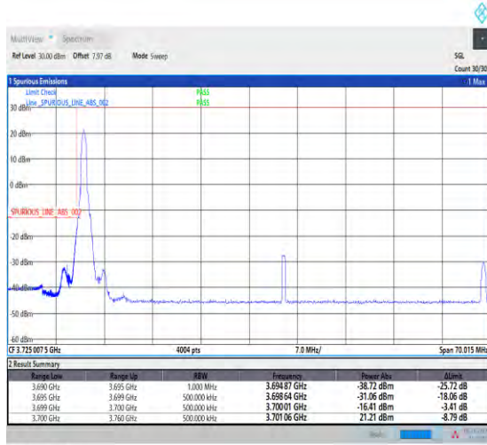
1-N78-3700-3800-PASS-30-60-L-1-DFT-PI2BPSK-Edge_1RB_Left-1@0-Ant1-1--PASS-see graph
