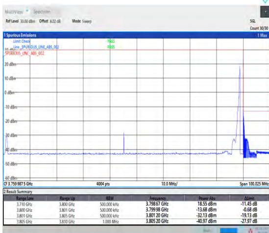
1-N78-3700-3800-PASS-30-90-H-2-DFT-PI2BPSK-Edge_1RB_Right-1@244-Ant1-1--PASS-see graph
