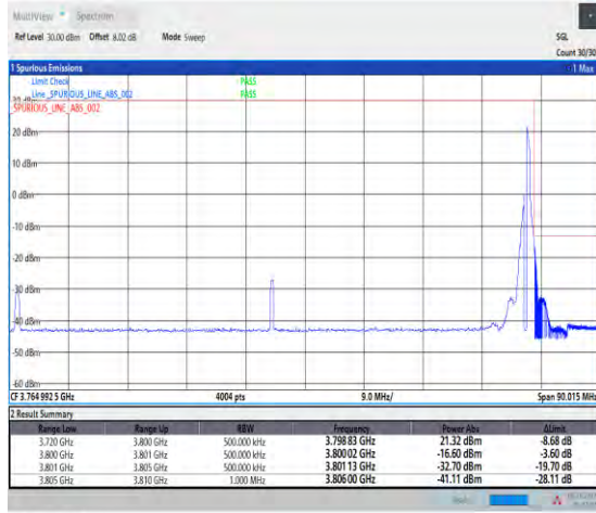
1-N78-3700-3800-PASS-30-80-H-2-DFT-PI2BPSK-Edge_1RB_Right-1@216-Ant1-1--PASS-see graph
