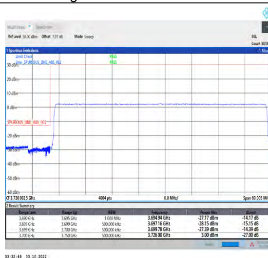
1-N78-3700-3800-PASS-30-50-L-3-DFT-PI2BPSK-Outer_Full-128@0-Ant1-1--PASS-see graph
