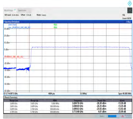
1-N78-3700-3800-PASS-30-40-L-3-DFT-PI2BPSK-Outer_Full-100@0-Ant1-1--PASS-see graph
