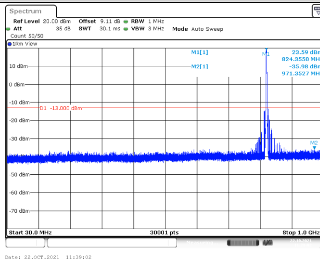
Band5-1.4MHz-16QAM-20407-6-0-Low-1000-5000--40.75-PASS
