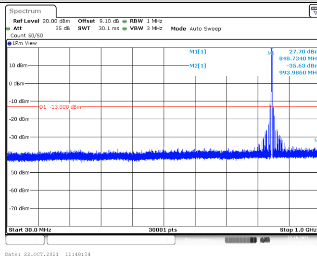
Band5-1.4MHz-QPSK-20643-1-5-Low-1000-5000--40.67-PASS
