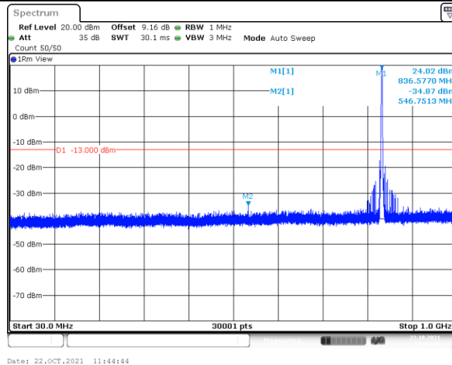
Band5-1.4MHz-QPSK-20525-6-0-Low-1000-5000--40.58-PASS
