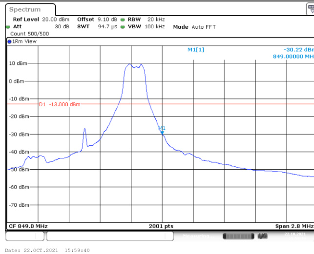
Band5-1.4MHz-QPSK-20643-6-0-Low--37.47-PASS
