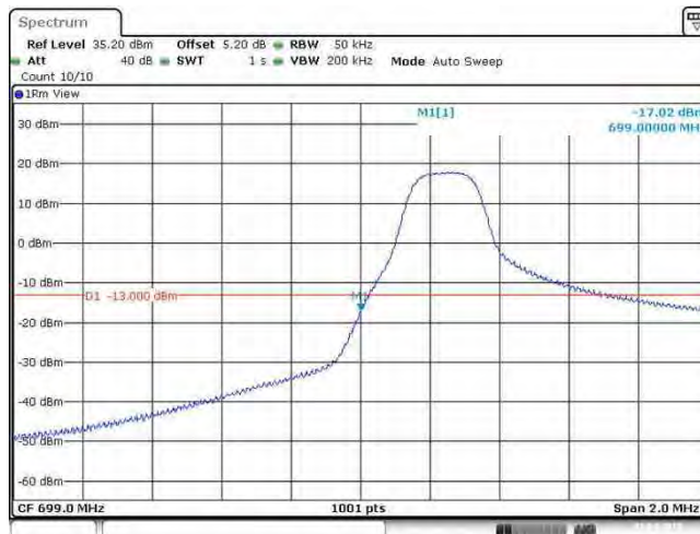
Band12_3MHz_64QAM_23025_15RB#0
