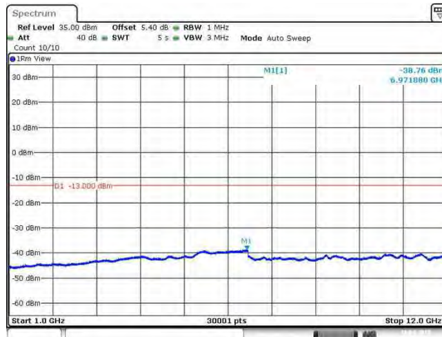
Band12_10MHz_64QAM_23095_1RB#0
