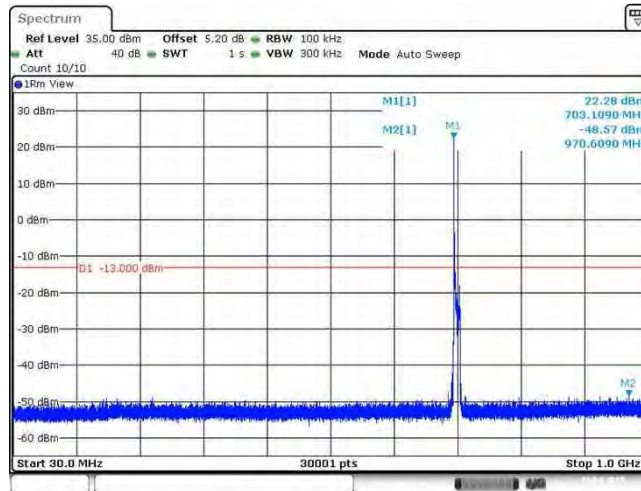
Band12_10MHz_64QAM_23095_1RB#0
