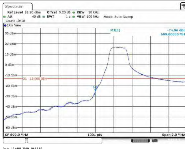
Band12_1.4MHz_QPSK_23017_6RB#0
