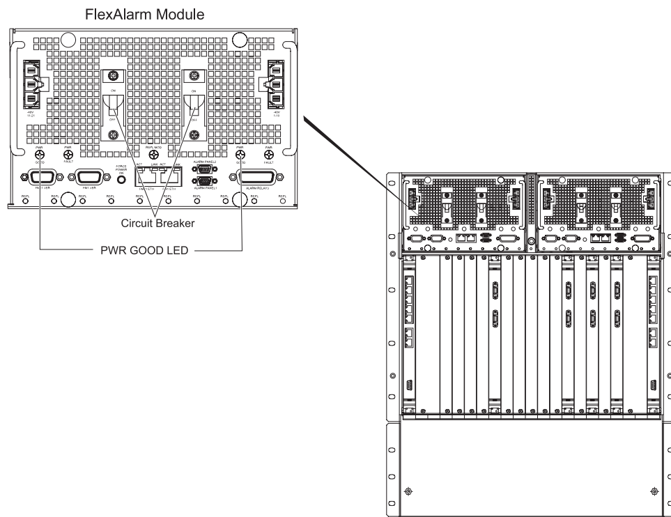
Figure 6.1 Circuit Breakers on the Digital Shelf
