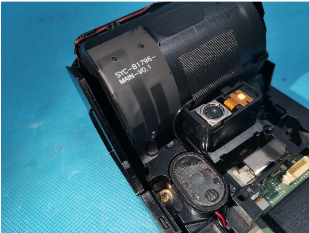
INTERNAL VIEW-3 OF EUT(GSM&amp;WCDMA&amp;LTE Antenna)
