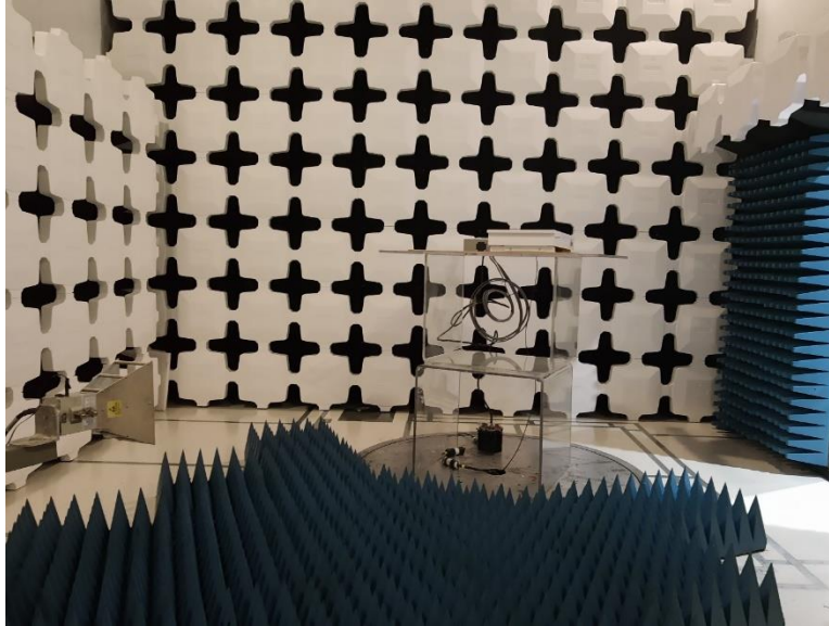
Photograph 3. REE Test Setup, 1-18 GHz
