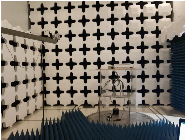
Photograph 4. REE Test Setup, 18-25 GHz
