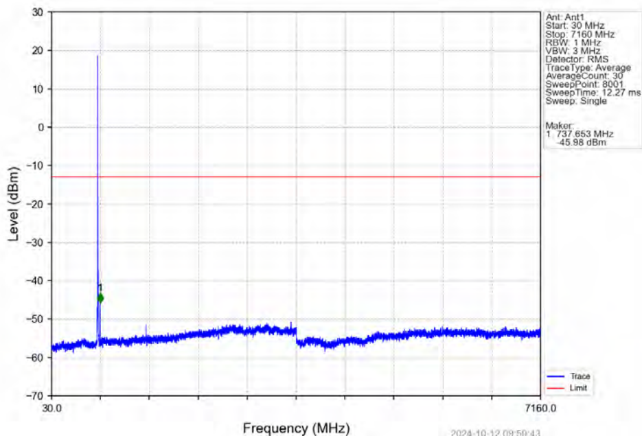
Band17_5MHz_QPSK_LCH_706.5MHz_RB_25_0 NTN
