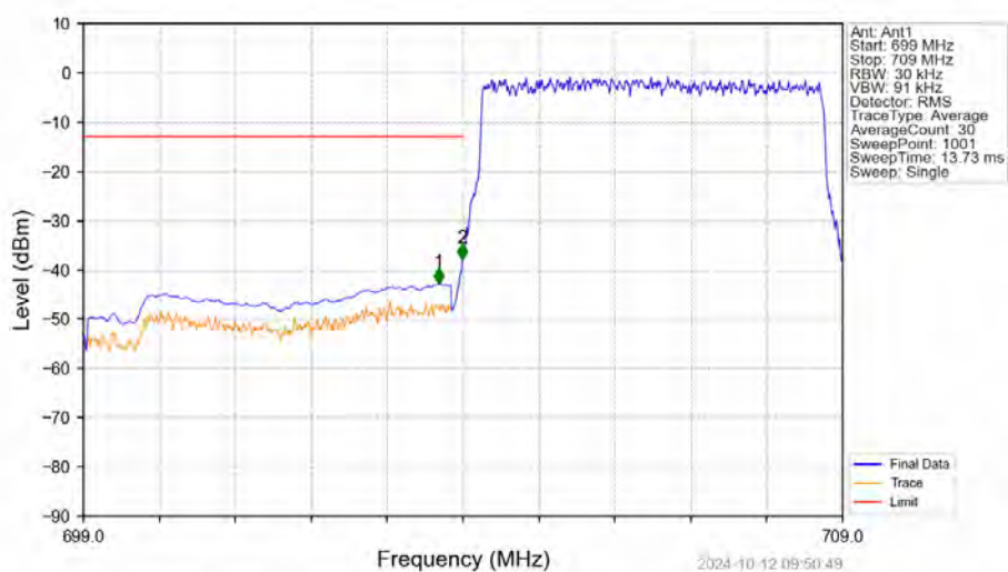
Band17_5MHz_QPSK_LCH_706.5MHz_RB_25_0 NTN
