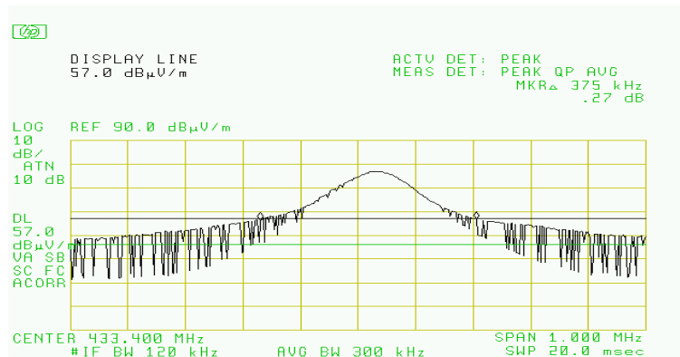
Figure 6.1 Occupied Bandwidth
