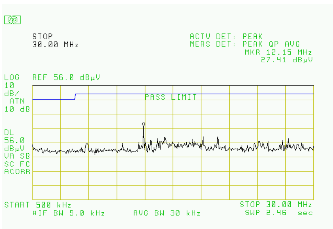
Fig. 5.1 Conducted Emission-Line
