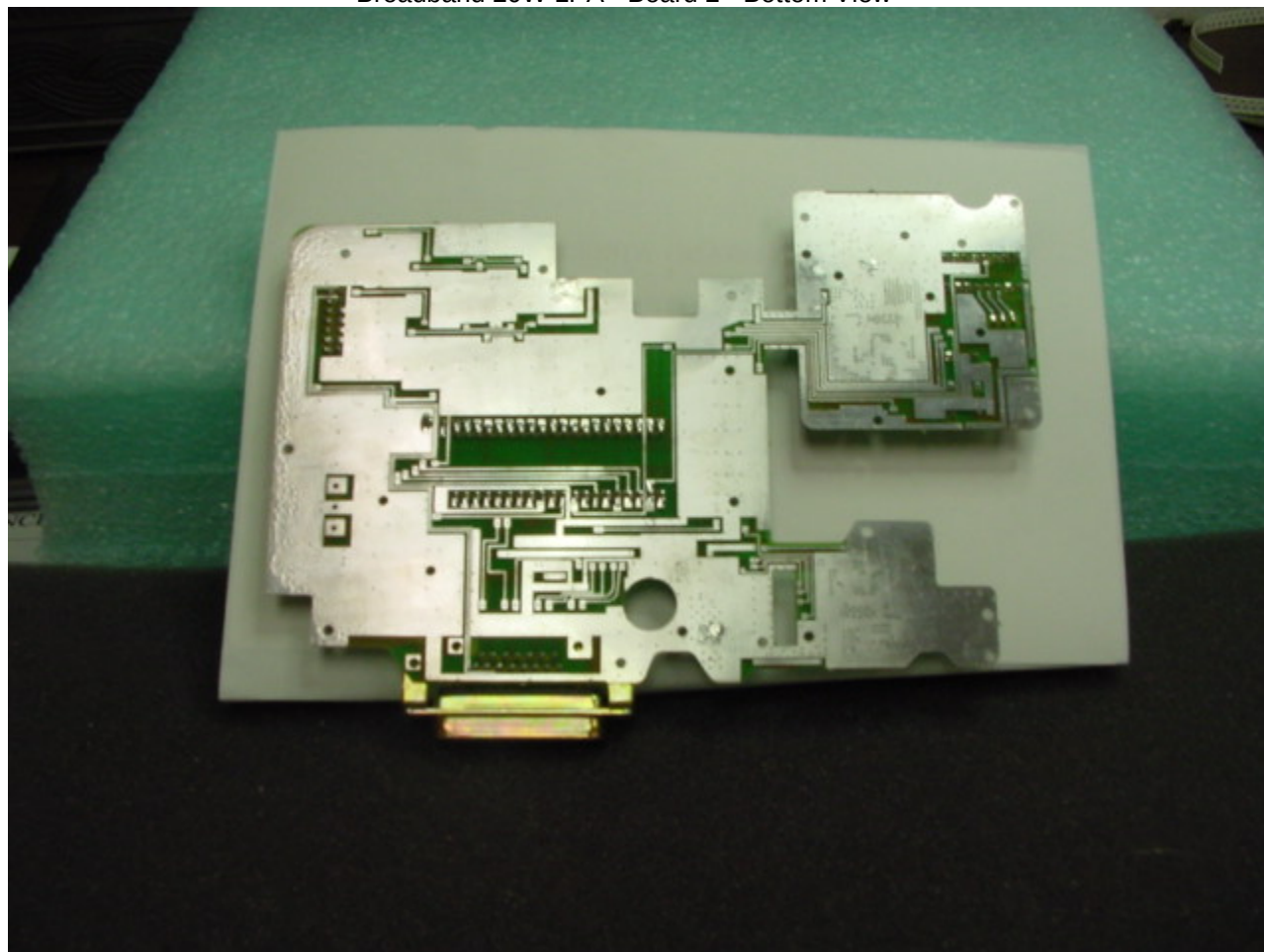
Broadband 20W LPA - Board 2 - Bottom View
