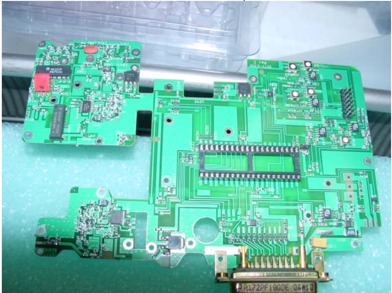
Broadband 20W LPA - Board 2 - Top View
