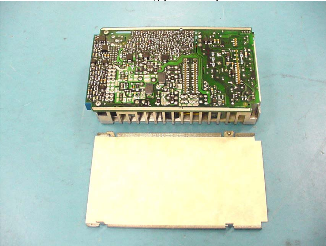
Cherokee Power Supply - Disassembly View 2
