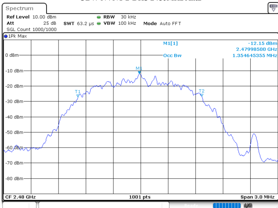
OBW NVNT 2-DH5 2480MHz Ant2
