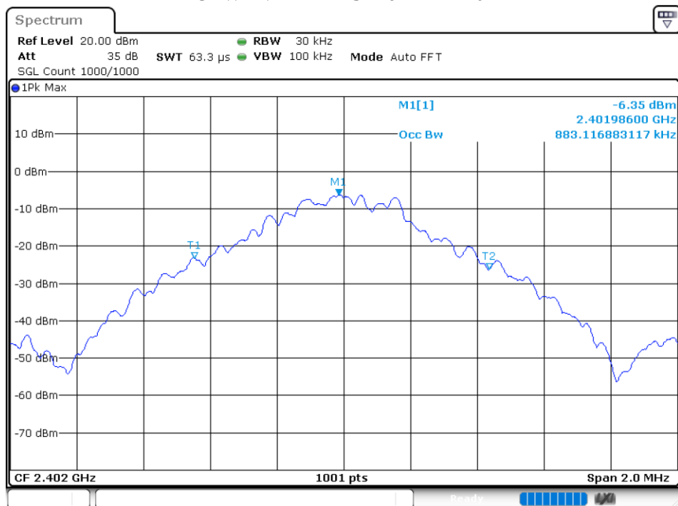
OBW NVNT 1-DH5 2402MHz Ant2
