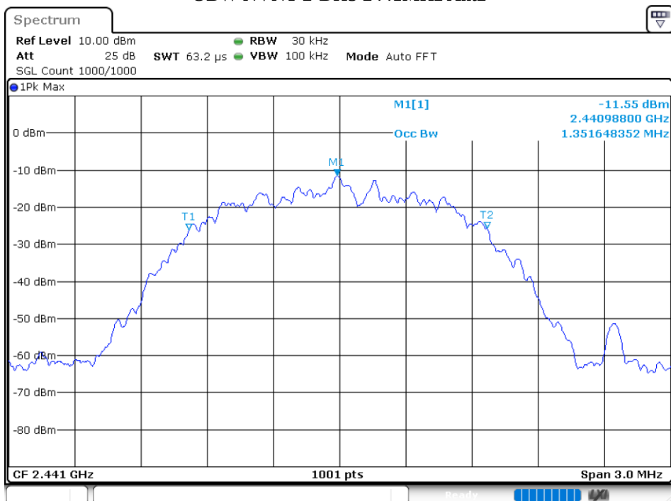
OBW NVNT 2-DH5 2441MHz Ant2
