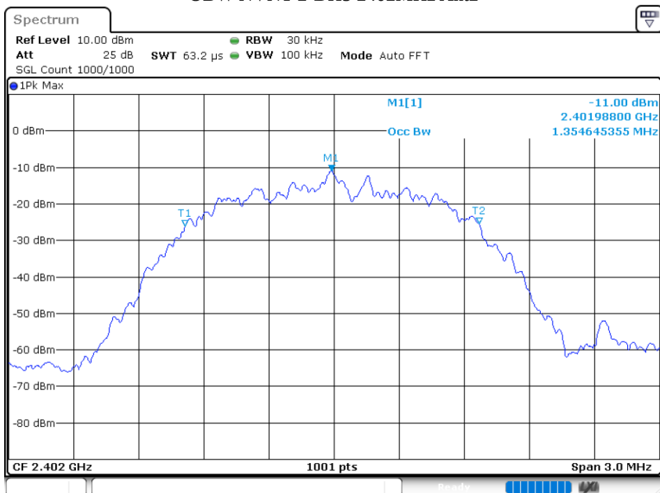
OBW NVNT 2-DH5 2402MHz Ant2
