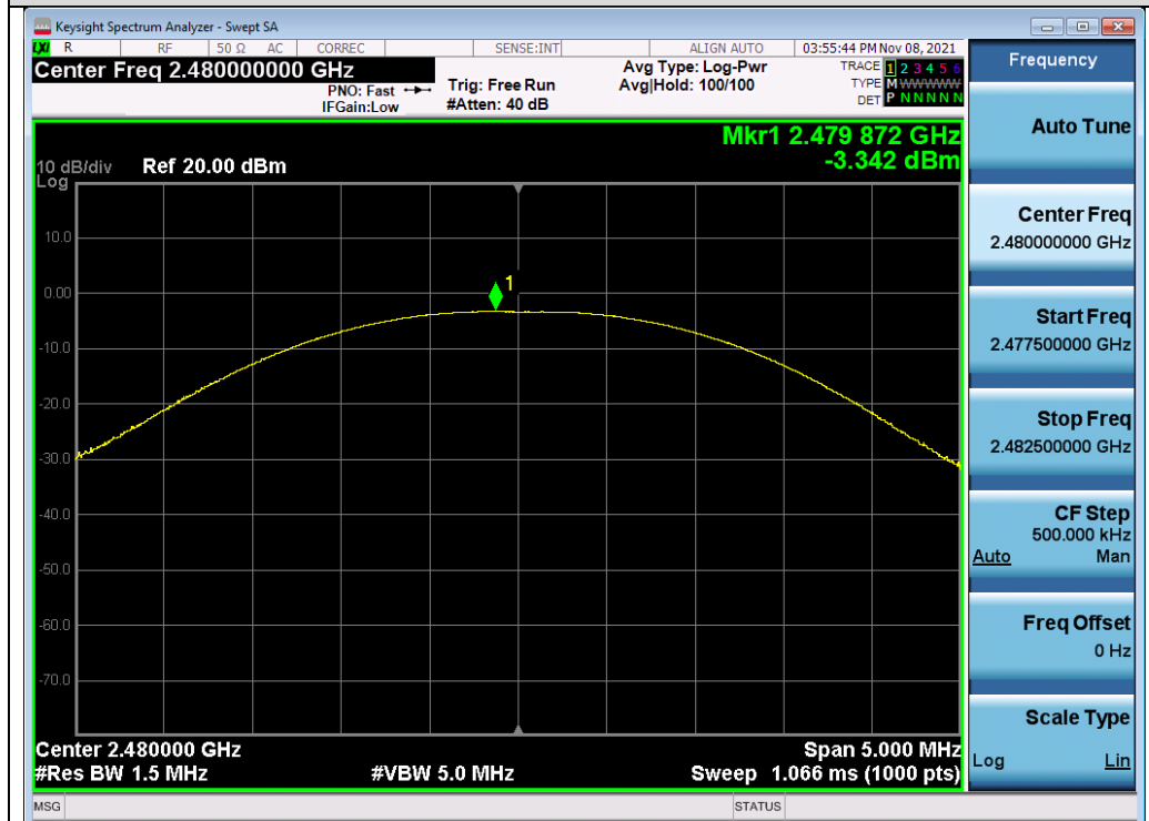
Test_Graph_BR_ANT1_2480_1Mbps_Peak Power
