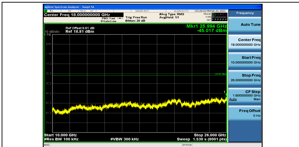
RF Conducted Spurious Emissions_11B_2437
