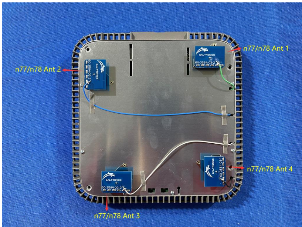
(2) EUT Photo (Model name: AV27-F370-P4CXP-FM-C)
