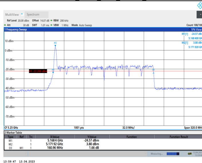
11AX160_Ant10_5250_52Tone_RU37
