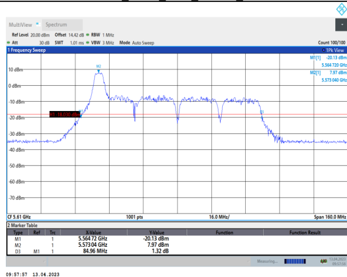
11AX80_Ant10_5610_106Tone_RU53
