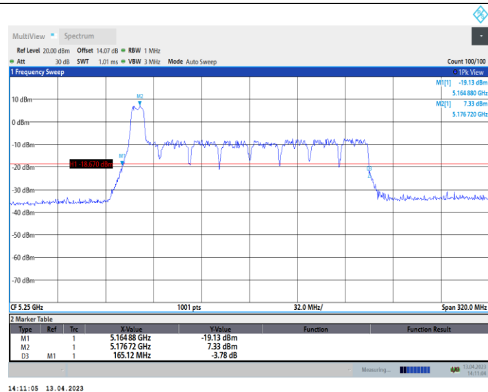
11AX160_Ant10_5250_242Tone_RU61
