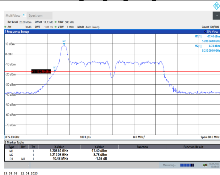
11AX40_Ant10_5230_52Tone_RU37
