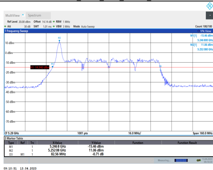
11AX80_Ant10_5290_52Tone_RU37
