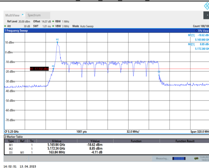
11AX160_Ant10_5250_106Tone_RU53
