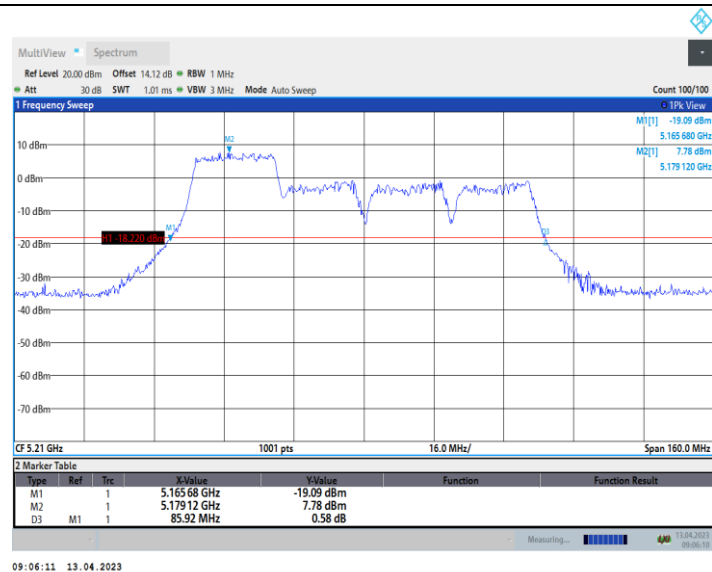
11AX80_Ant10_5210_484Tone_RU65
