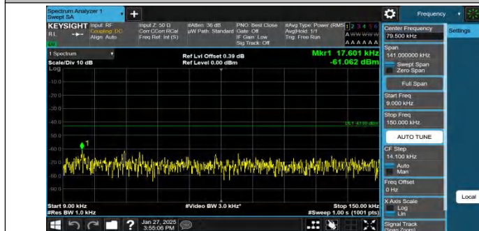
Band2-9400-1-0.009~0.15MHz-PASS
