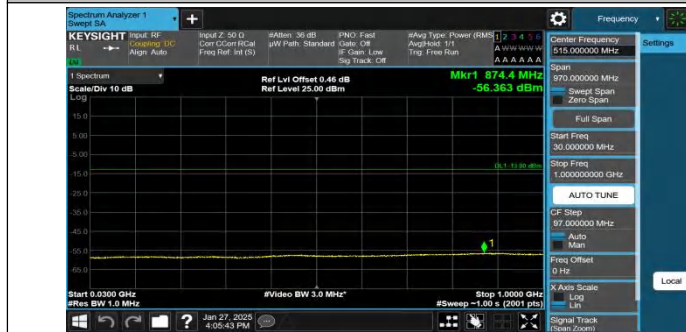
Band2-9262-5-30~1000MHz-PASS
