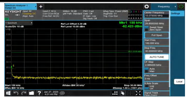
Band2-9538-3-0.15~30MHz-PASS
