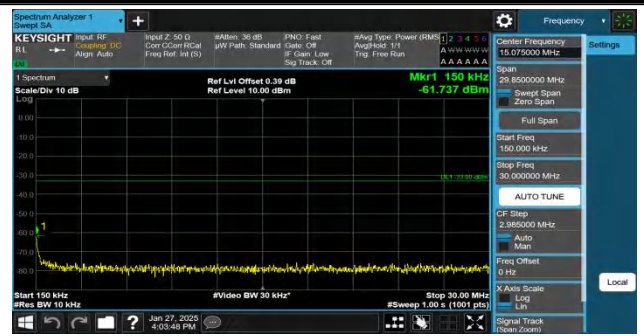
Band2-9400-4-0.15~30MHz-PASS
