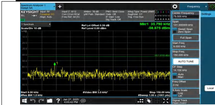
Band2-9400-4-0.009~0.15MHz-PASS
