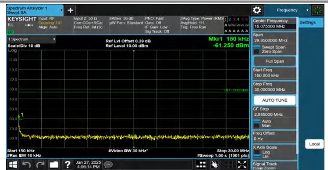
Band2-9400-5-0.15~30MHz-PASS
