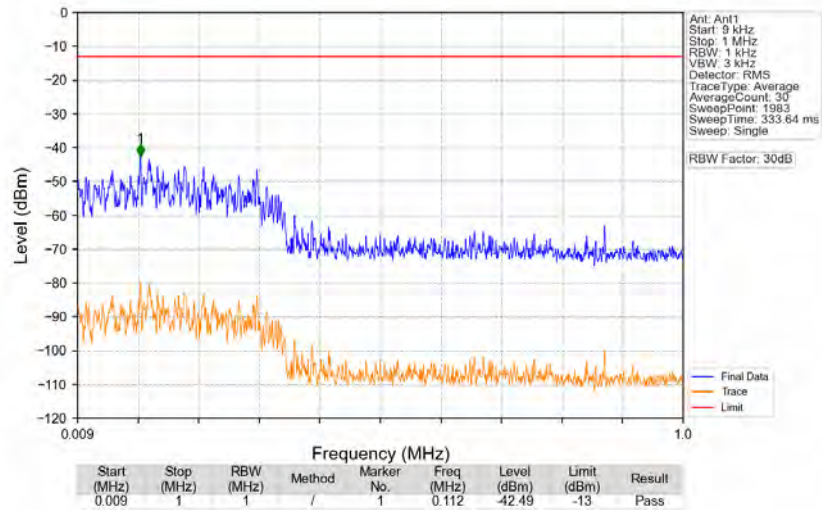
n77a_30kHz_SISO_NTNV_80MHz_DFT-s-OFDM_QPSK_3740.01MHz_Edge_1RB_Left
