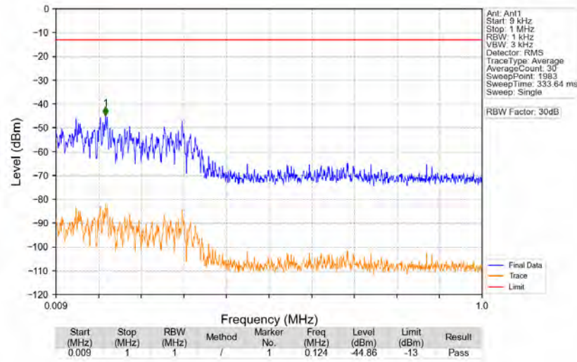
n77a_30kHz_SISO_NTNV_100MHz_DFT-s-OFDM_PI/2_BPSK_3840MHz_Edge_1RB_Left
