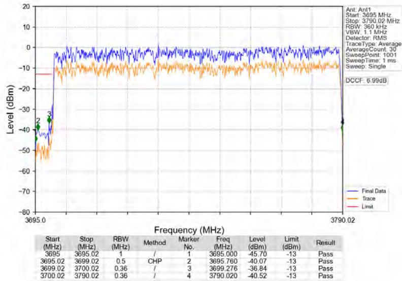
n77a_30kHz_SISO_NTNV_90MHz_CP-OFDM_QPSK_3745.02MHz_Outer_Full
