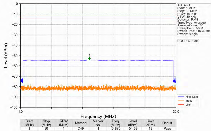
n77a_30kHz_SISO_NTNV_100MHz_DFT-s-OFDM_QPSK_3930MHz_Edge_1RB_Right
