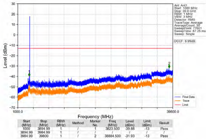
n77a_30kHz_SISO_NTNV_80MHz_DFT-s-OFDM_PI/2_BPSK_3939.99MHz_Edge_1RB_Right
