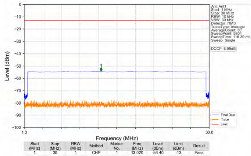
n77a_30kHz_SISO_NTNV_70MHz_CP-OFDM_QPSK_3840MHz_Edge_1RB_Left
