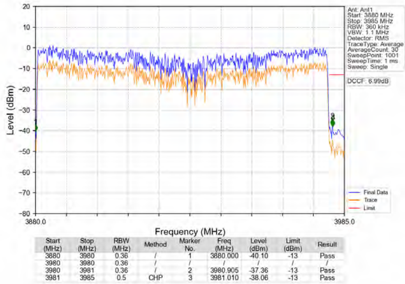
n77a_30kHz_SISO_NTNV_100MHz_CP-OFDM_QPSK_3930MHz_Outer_Full
