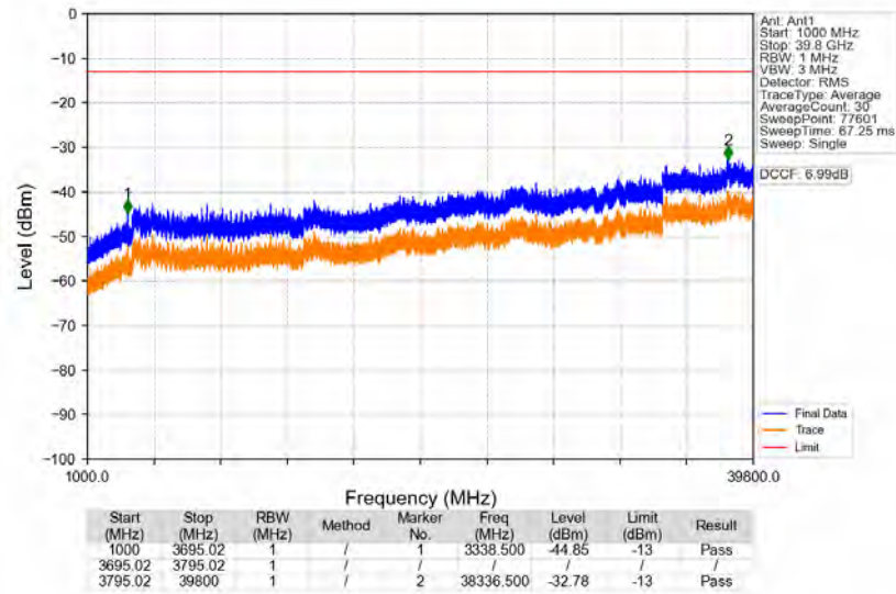
n77a_30kHz_SISO_NTNV_90MHz_DFT-s-OFDM_PI/2_BPSK_3745.02MHz_Edge_1RB_Left
