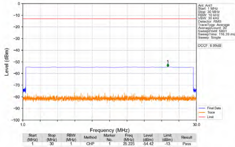
n77a_30kHz_SISO_NTNV_100MHz_DFT-s-OFDM_PI/2_BPSK_3840MHz_Edge_1RB_Left
