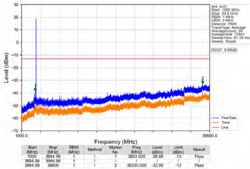
n77a_30kHz_SISO_NTNV_90MHz_DFT-s-OFDM_PI/2_BPSK_3934.98MHz_Edge_1RB_Right
