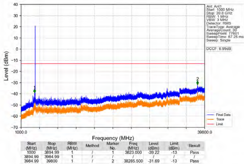
n77a_30kHz_SISO_NTNV_80MHz_DFT-s-OFDM_QPSK_3939.99MHz_Edge_1RB_Right
