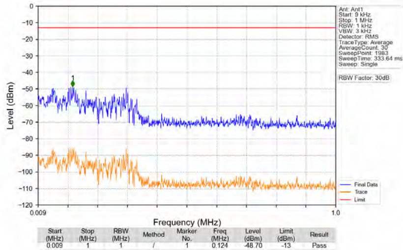
n77a_30kHz_SISO_NTNV_100MHz_DFT-s-OFDM_PI/2_BPSK_3930MHz_Edge_1RB_Right
