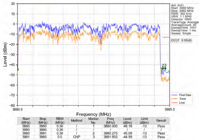
n77a 30kHz SISO NTN 100MHz DFT-s-OFDM PI/2 BPSK 3930MHz Outer_Full
