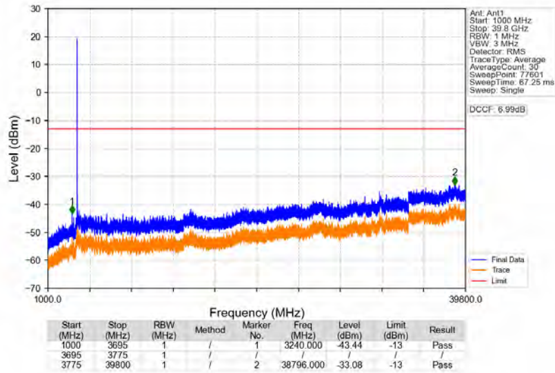
n77a_30kHz_SISO_NTNV_70MHz_CP-OFDM_QPSK_3735MHz_Edge_1RB_Left
