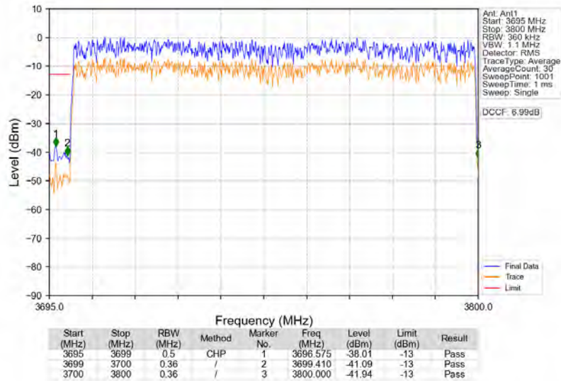
n77a 30kHz SISO_NTNV_100MHz_CP-OFDM QPSK 3750MHz_Outer_Full
