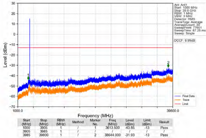
n77a 30kHz SISO NTN 70MHz CP-OFDM QPSK 3945MHz Edge_1RB_Right
