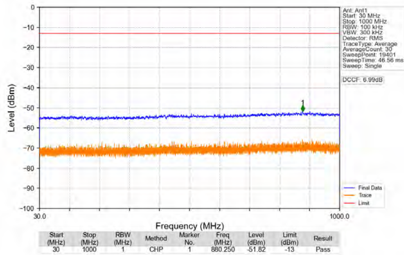
n77a_30kHz_SISO_NTNV_100MHz_DFT-s-OFDM_QPSK_3750MHz_Edge_1RB_Left
