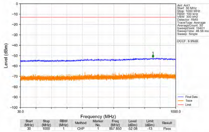
n77a_30kHz_SISO_NTNV_80MHz_DFT-s-OFDM_QPSK_3840MHz_Edge_1RB_Left
