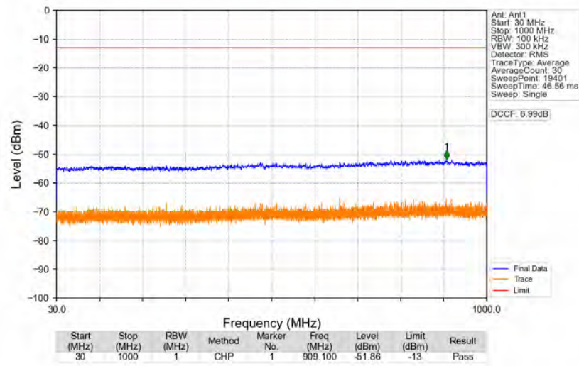
n77a_30kHz_SISO_NTNV_90MHz_DFT-s-OFDM_QPSK_3840MHz_Edge_1RB_Left
