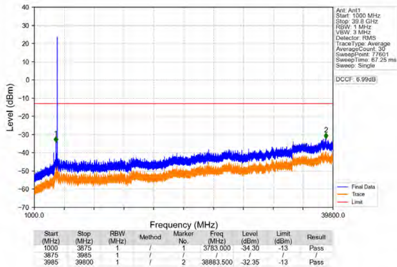
n77a_30kHz_SISO_NTNV_100MHz_DFT-s-OFDM_QPSK_3930MHz_Edge_1RB_Right
