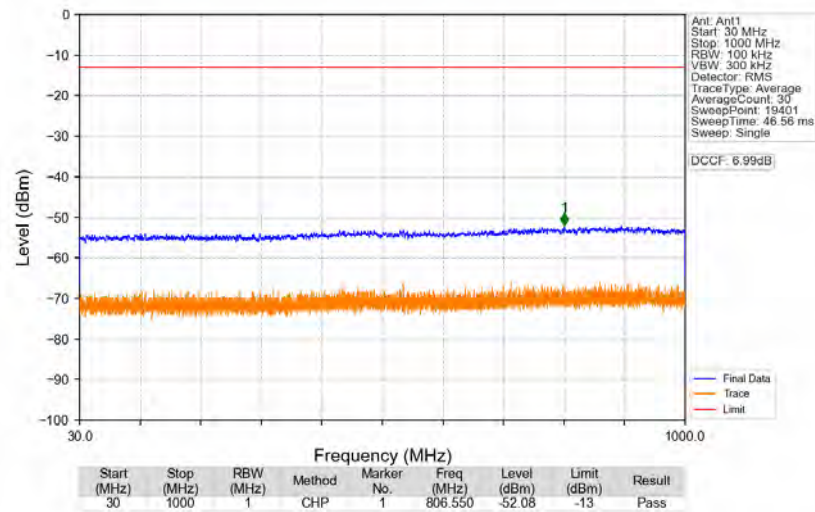
n77a_30kHz_SISO_NTNV_80MHz_DFT-s-OFDM_QPSK_3939.99MHz_Edge_1RB_Right
