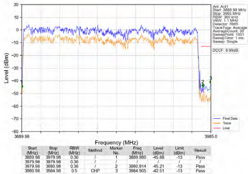
n77a_30kHz_SISO_NTNV_90MHz_DFT-s-OFDM_QPSK_3934.98MHz_Outer_Full
