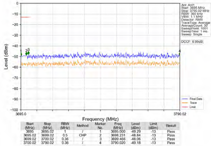
n77a_30kHz_SISO_NTNV_90MHz_DFT-s-OFDM_PI/2_BPSK_3745.02MHz_Outer_Full
