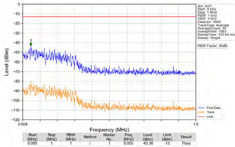
n77a_30kHz_SISO_NTNV_80MHz_CP-OFDM_QPSK_3840MHz_Edge_1RB_Left
