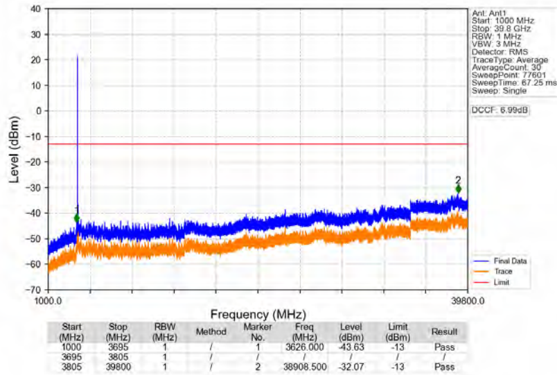
n77a 30kHz SISO_NTNV_100MHz_CP-OFDM QPSK 3750MHz_Edge_1RB_Left
