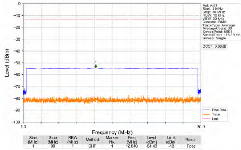
n77a_30kHz_SISO_NTNV_80MHz_CP-OFDM_QPSK_3740.01MHz_Edge_1RB_Left
