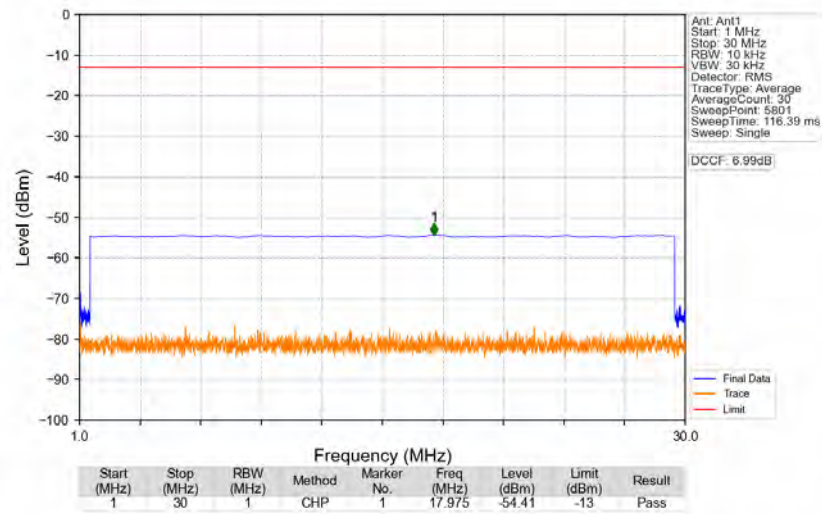
n77a_30kHz_SISO_NTNV_100MHz_DFT-s-OFDM_QPSK_3750MHz_Edge_1RB_Left
