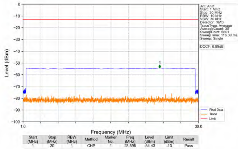
n77a_30kHz_SISO_NTNV_80MHz_DFT-s-OFDM_QPSK_3939.99MHz_Edge_1RB_Right
