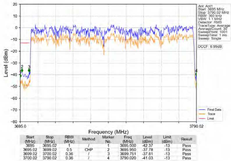
n77a_30kHz_SISO_NTNV_90MHz_DFT-s-OFDM_QPSK_3745.02MHz_Outer_Full
