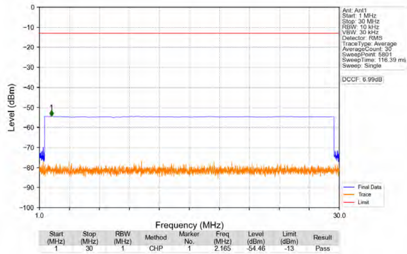
n77a_30kHz_SISO_NTNV_80MHz_DFT-s-OFDM_QPSK_3740.01MHz_Edge_1RB_Left
