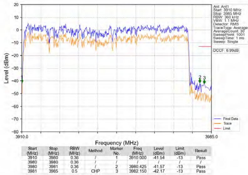
n77a 30kHz SISO NTN 70MHz DFT-s-OFDM QPSK 3945MHz Outer Full
