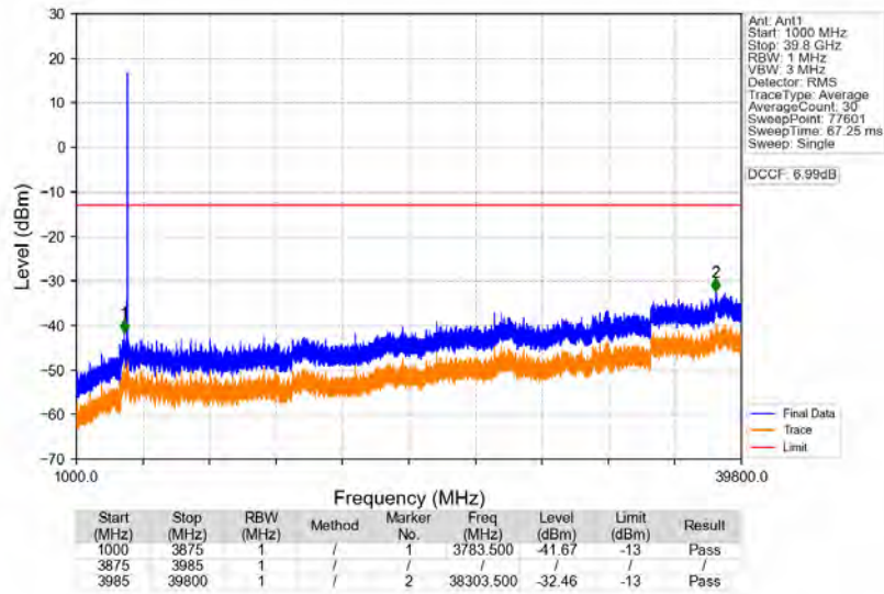
n77a_30kHz_SISO_NTNV_100MHz_CP-OFDM_QPSK_3930MHz_Edge_1RB_Right
