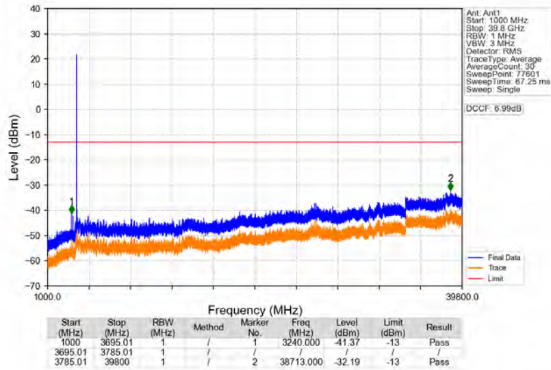
n77a_30kHz_SISO_NTNV_80MHz_DFT-s-OFDM_QPSK_3740.01MHz_Edge_1RB_Left
