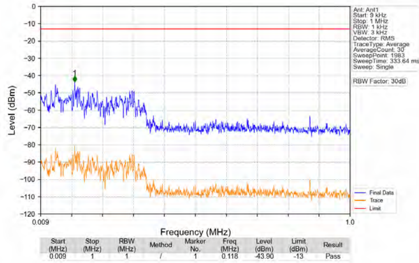
n77a_30kHz_SISO_NTNV_80MHz_DFT-s-OFDM_PI/2_BPSK_3840MHz_Edge_1RB_Left
