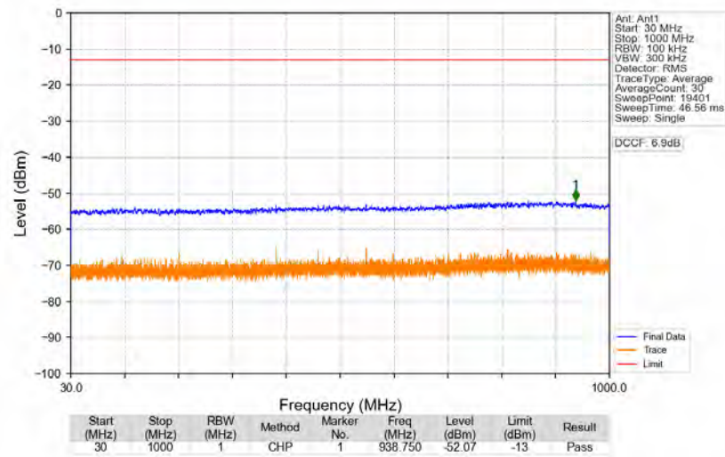
n77a_30kHz_SISO_NTNV_90MHz_DFT-s-OFDM_QPSK_3934.98MHz_Edge_1RB_Right
