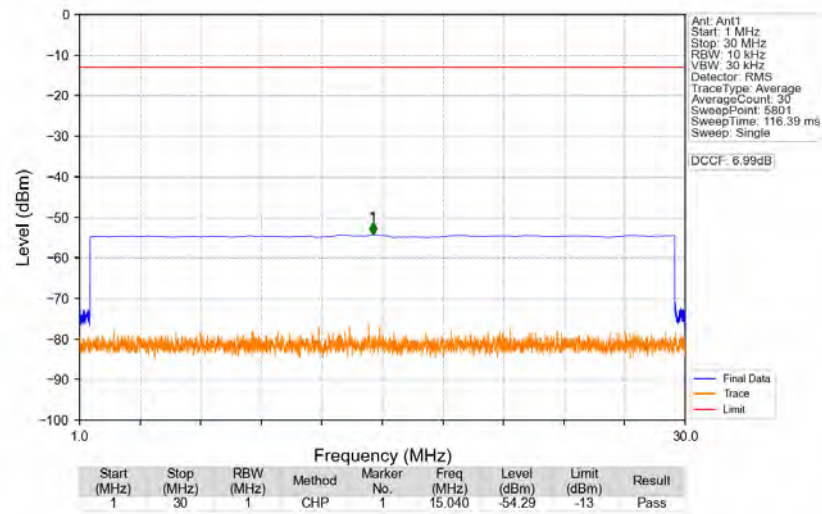
n77a_30kHz_SISO_NTNV_70MHz_CP-OFDM_QPSK_3735MHz_Edge_1RB_Left
