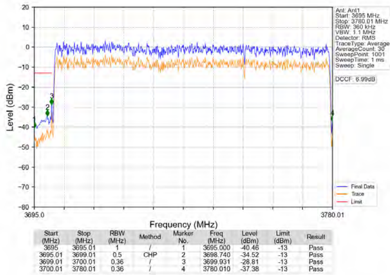
n77a_30kHz_SISO_NTNV_80MHz_CP-OFDM_QPSK_3740.01MHz_Outer_Full
