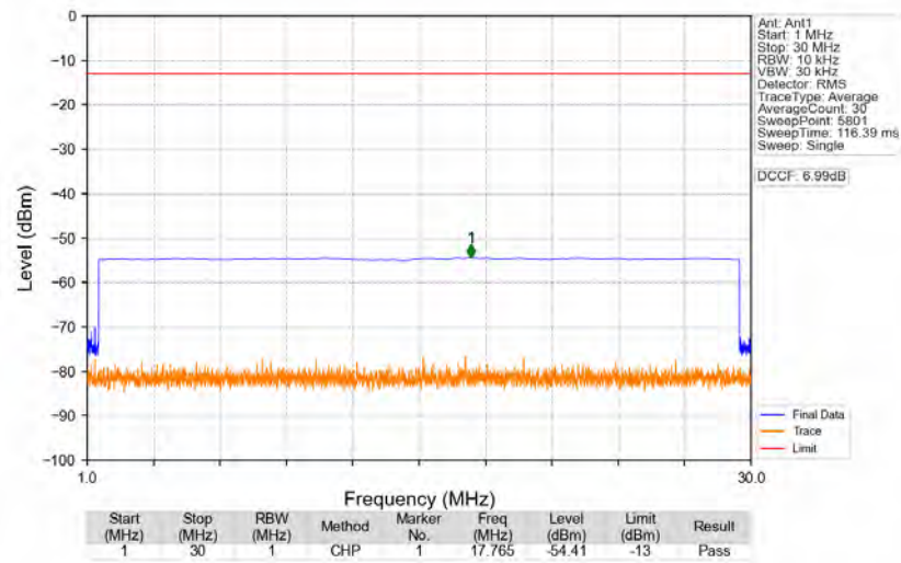
n77a_30kHz_SISO_NTNV_100MHz_DFT-s-OFDM_PI/2_BPSK_3750MHz_Edge_1RB_Left
