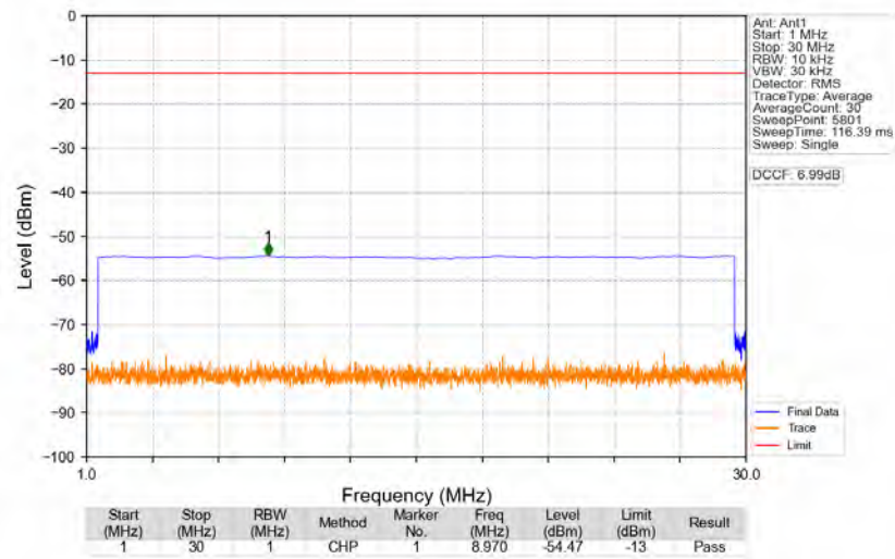
n77a_30kHz_SISO_NTNV_90MHz_DFT-s-OFDM_QPSK_3745.02MHz_Edge_1RB_Left
