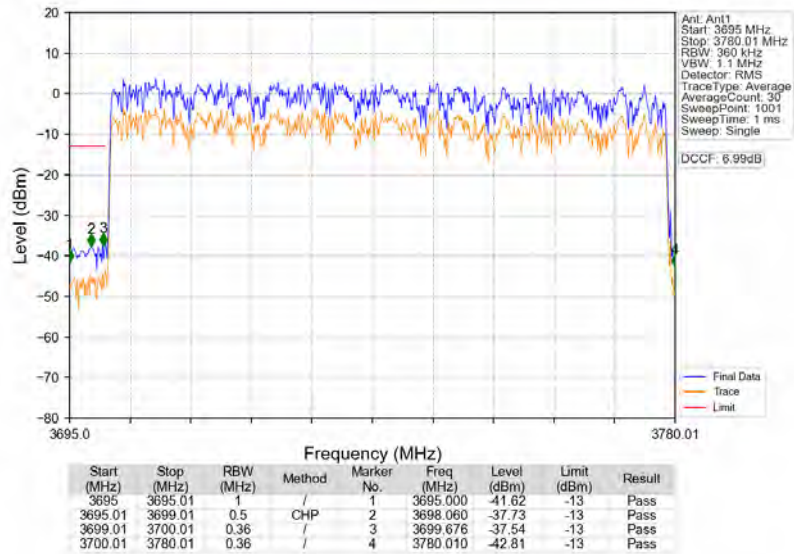
n77a_30kHz_SISO_NTNV_80MHz_DFT-s-OFDM_QPSK_3740.01MHz_Outer_Full
