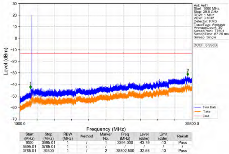
n77a_30kHz_SISO_NTNV_80MHz_CP-OFDM_QPSK_3740.01MHz_Edge_1RB_Left
