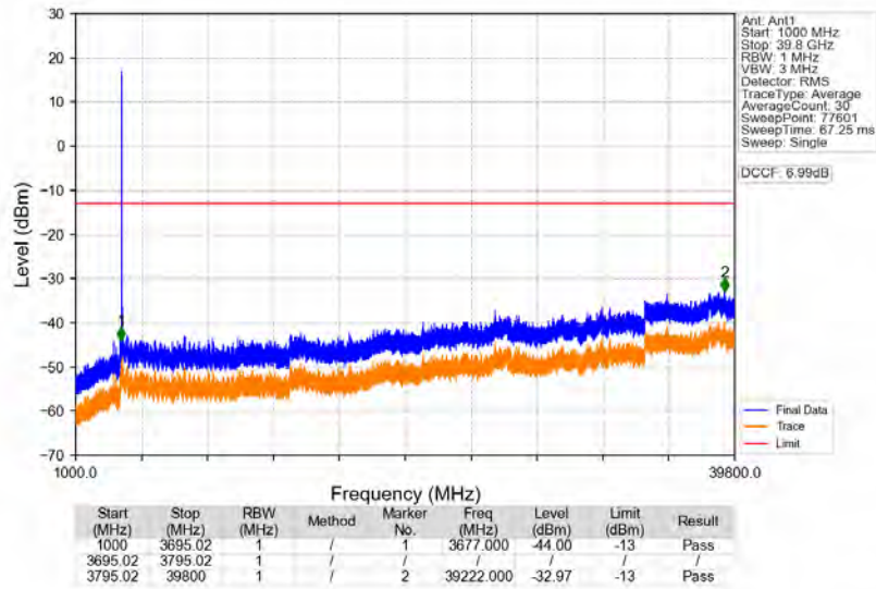
n77a_30kHz_SISO_NTNV_90MHz_CP-OFDM_QPSK_3745.02MHz_Edge_1RB_Left
