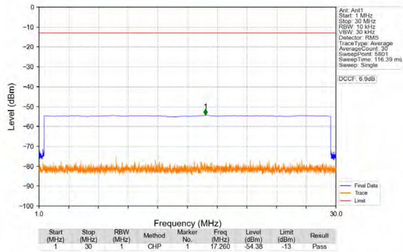
n77a_30kHz_SISO_NTNV_90MHz_DFT-s-OFDM_QPSK_3934.98MHz_Edge_1RB_Right
