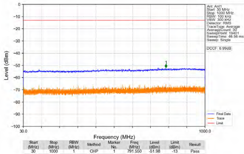
n77a_30kHz_SISO_NTNV_90MHz_CP-OFDM_QPSK_3745.02MHz_Edge_1RB_Left
