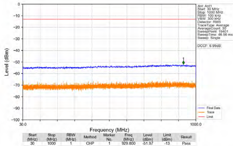
n77a_30kHz_SISO_NTNV_100MHz_DFT-s-OFDM_PI/2_BPSK_3750MHz_Edge_1RB_Left
