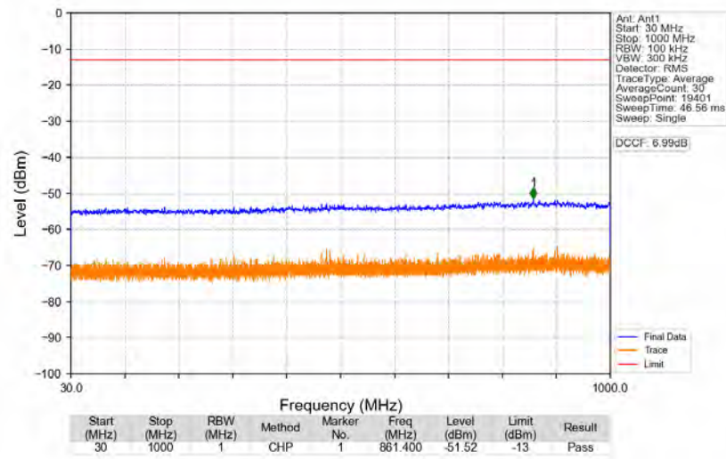
n77a_30kHz_SISO_NTNV_90MHz_DFT-s-OFDM_PI/2_BPSK_3840MHz_Edge_1RB_Left
