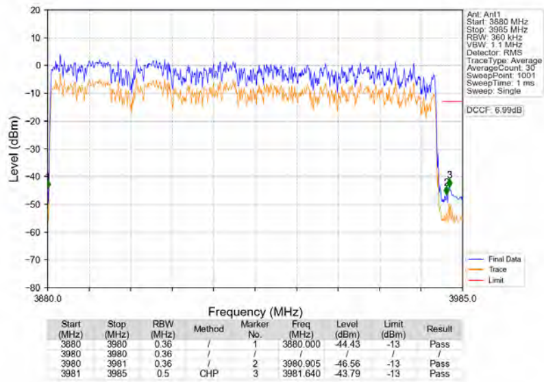
n77a_30kHz_SISO_NTNV_100MHz_DFT-s-OFDM_QPSK_3930MHz_Outer_Full
