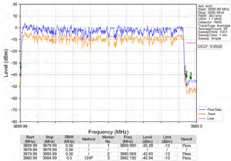
n77a_30kHz_SISO_NTNV_80MHz_DFT-s-OFDM_QPSK_3939.99MHz_Outer_Full
