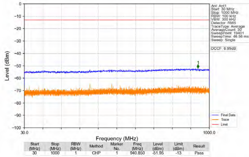
n77a_30kHz_SISO_NTNV_70MHz_CP-OFDM_QPSK_3840MHz_Edge_1RB_Left
