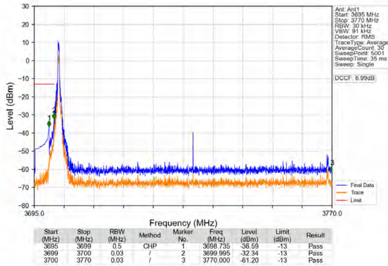
n77a_30kHz_SISO_NTNV_70MHz_CP-OFDM_QPSK_3735MHz_Edge_1RB_Left
