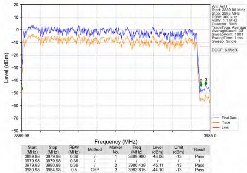
n77a_30kHz_SISO_NTNV_90MHz_DFT-s-OFDM_PI/2_BPSK_3934.98MHz_Outer_Full
