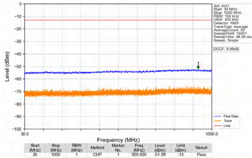
n77a_30kHz_SISO_NTNV_100MHz_DFT-s-OFDM_PI/2_BPSK_3840MHz_Edge_1RB_Left
