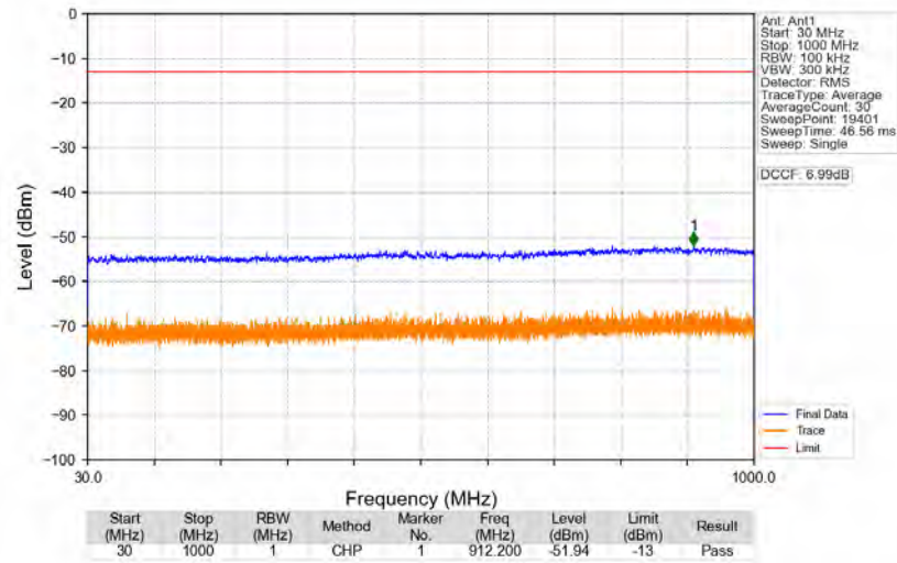
n77a_30kHz_SISO_NTNV_80MHz_CP-OFDM_QPSK_3840MHz_Edge_1RB_Left
