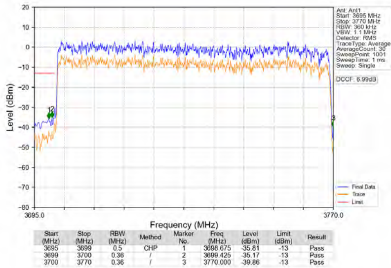
n77a_30kHz_SISO_NTNV_70MHz_CP-OFDM_QPSK_3735MHz_Outer_Full
