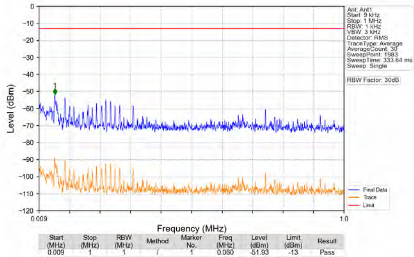
n77a_30kHz_SISO_NTNV_90MHz_CP-OFDM_QPSK_3745.02MHz_Edge_1RB_Left
