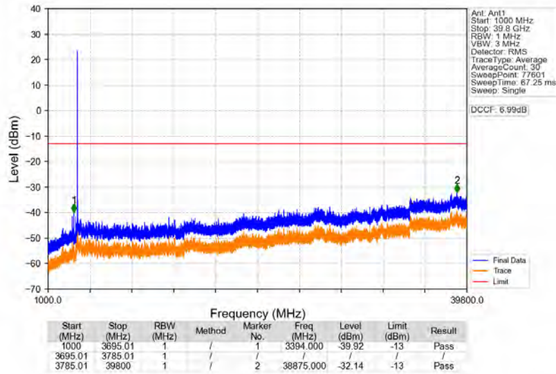
n77a_30kHz_SISO_NTNV_80MHz_DFT-s-OFDM_PI/2_BPSK_3740.01MHz_Edge_1RB_Left
