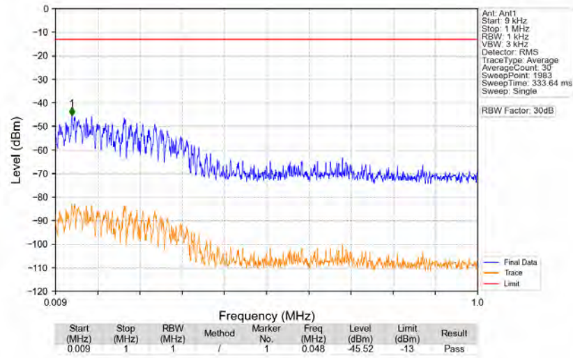
n77a_30kHz_SISO_NTNV_90MHz_CP-OFDM_QPSK_3840MHz_Edge_1RB_Left
