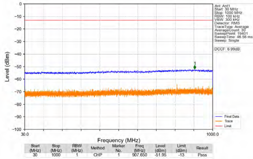
n77a_30kHz_SISO_NTNV_90MHz_CP-OFDM_QPSK_3840MHz_Edge_1RB_Left
