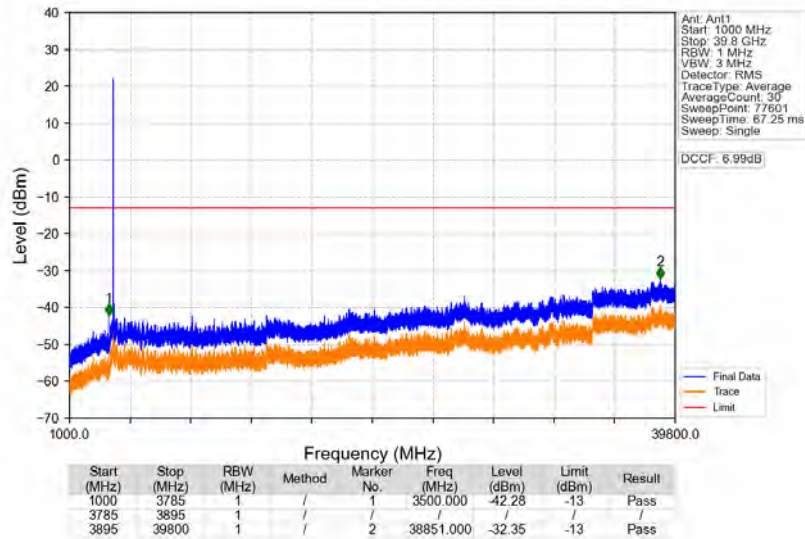
n77a_30kHz_SISO_NTNV_100MHz_DFT-s-OFDM_PI/2_BPSK_3840MHz_Edge_1RB_Left
