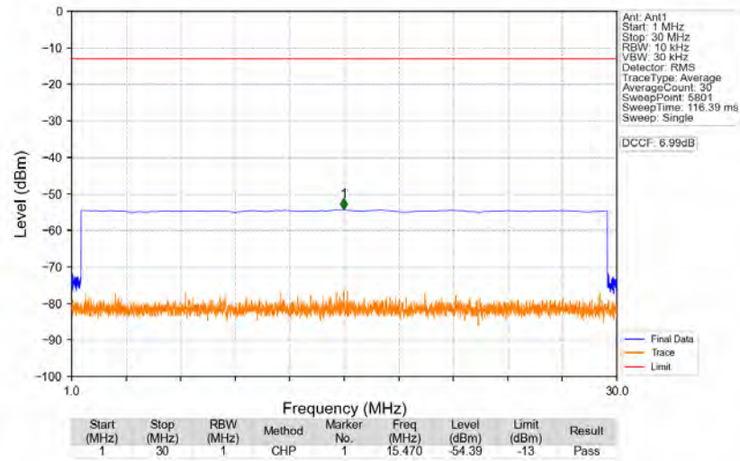
n77a_30kHz_SISO_NTNV_90MHz_CP-OFDM_QPSK_3840MHz_Edge_1RB_Left
