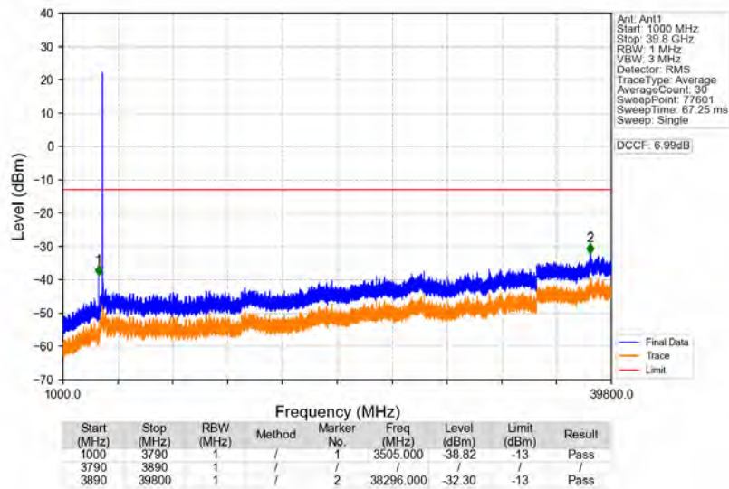
n77a_30kHz_SISO_NTNV_90MHz_DFT-s-OFDM_PI/2_BPSK_3840MHz_Edge_1RB_Left
