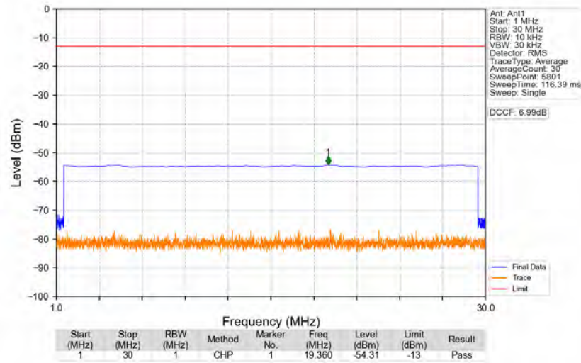
n77a_30kHz_SISO_NTNV_80MHz_DFT-s-OFDM_PI/2_BPSK_3840MHz_Edge_1RB_Left
