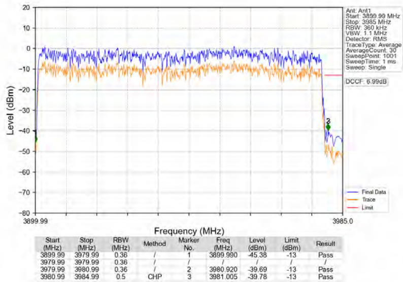
n77a 30kHz SISO NTN 80MHz CP-OFDM QPSK 3939.99MHz Outer Full
