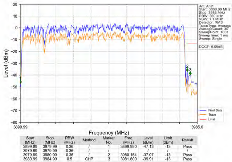
n77a_30kHz_SISO_NTNV_80MHz_DFT-s-OFDM_PI/2_BPSK_3939.99MHz_Outer_Full
