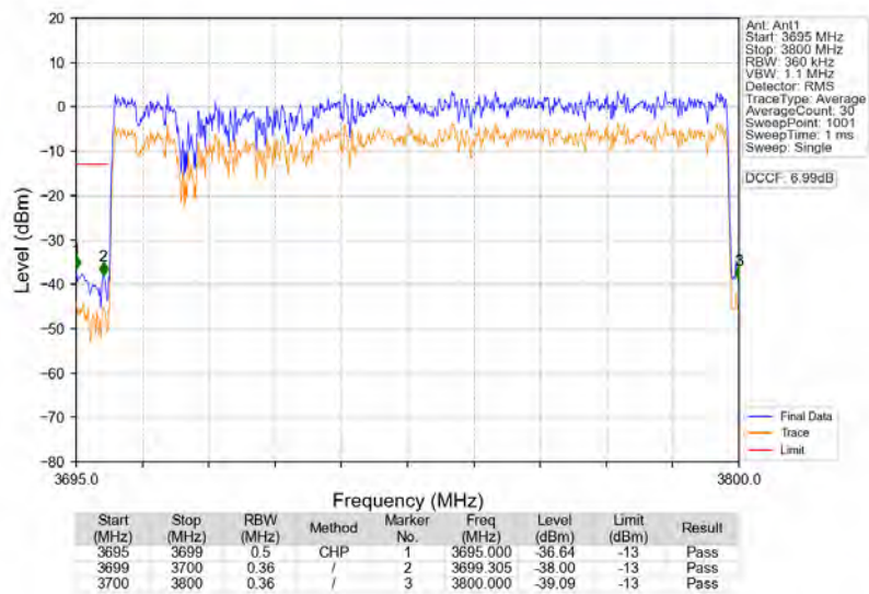
n77a 30kHz SISO_NTNV_100MHz_DFT-s-OFDM QPSK 3750MHz_Outer_Full
