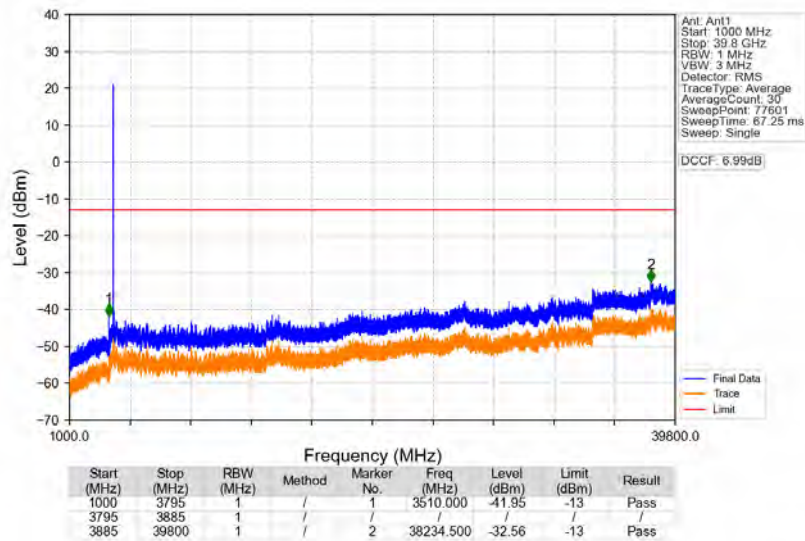
n77a_30kHz_SISO_NTNV_80MHz_DFT-s-OFDM_PI/2_BPSK_3840MHz_Edge_1RB_Left
