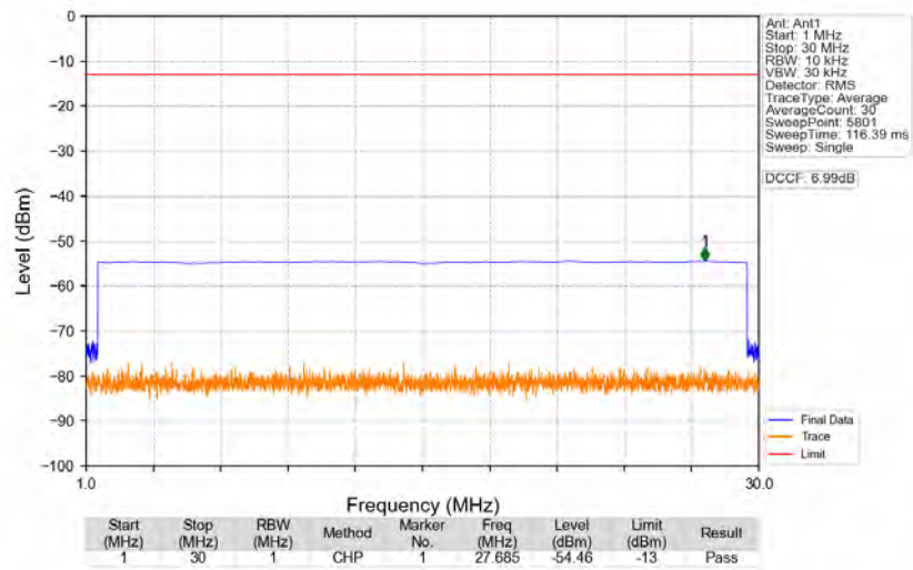
n77a_30kHz_SISO_NTNV_90MHz_DFT-s-OFDM_QPSK_3840MHz_Edge_1RB_Left
