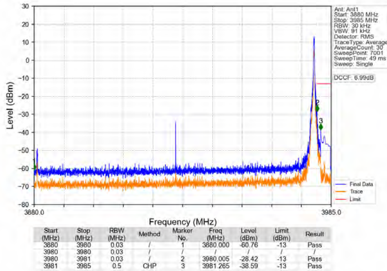
n77a_30kHz_SISO_NTNV_100MHz_DFT-s-OFDM_PI/2_BPSK_3930MHz_Edge_1RB_Right
