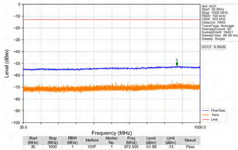
n77a_30kHz_SISO_NTNV_90MHz_DFT-s-OFDM_QPSK_3745.02MHz_Edge_1RB_Left
