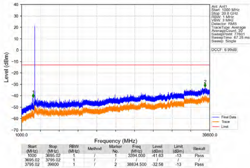
n77a_30kHz_SISO_NTNV_90MHz_DFT-s-OFDM_QPSK_3745.02MHz_Edge_1RB_Left
