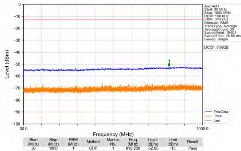
n77a_30kHz_SISO_NTNV_100MHz_DFT-s-OFDM_QPSK_3930MHz_Edge_1RB_Right
