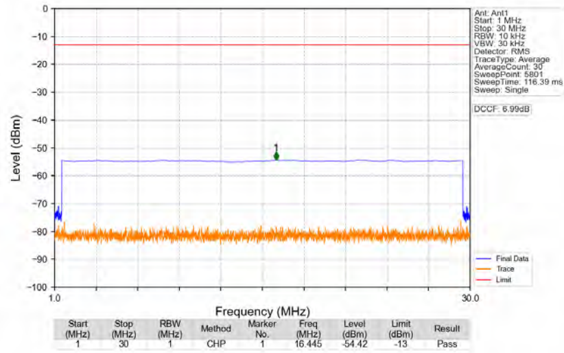
n77a_30kHz_SISO_NTNV_100MHz_CP-OFDM_QPSK_3930MHz_Edge_1RB_Right
