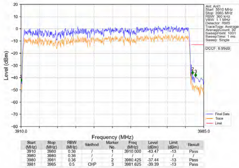
n77a 30kHz SISO NTN 70MHz CP-OFDM QPSK 3945MHz Outer Full
