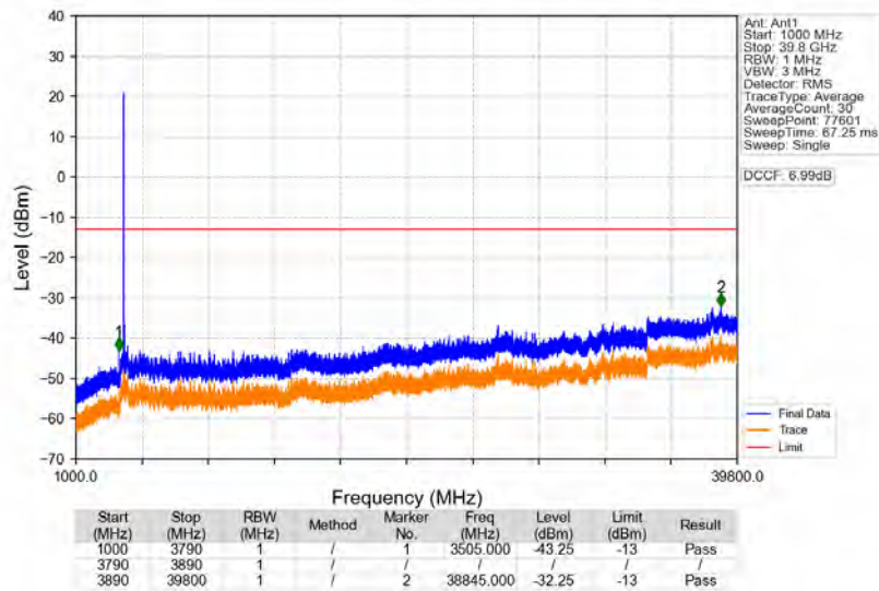
n77a_30kHz_SISO_NTNV_90MHz_CP-OFDM_QPSK_3840MHz_Edge_1RB_Left
