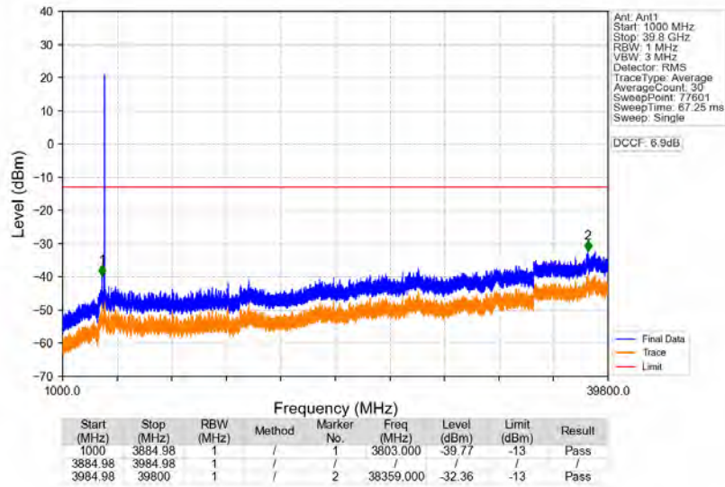
n77a_30kHz_SISO_NTNV_90MHz_DFT-s-OFDM_QPSK_3934.98MHz_Edge_1RB_Right
