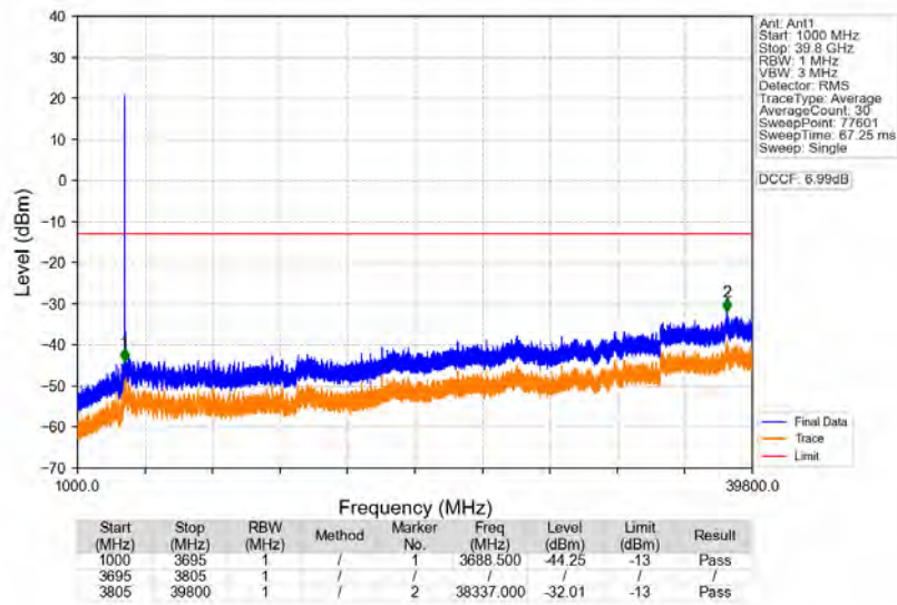
n77a 30kHz SISO_NTNV_100MHz_DFT-s-OFDM QPSK 3750MHz_Edge_1RB_Left
