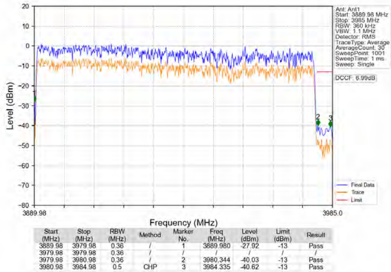
n77a 30kHz SISO NTN 90MHz CP-OFDM QPSK 3934.98MHz Outer Full
