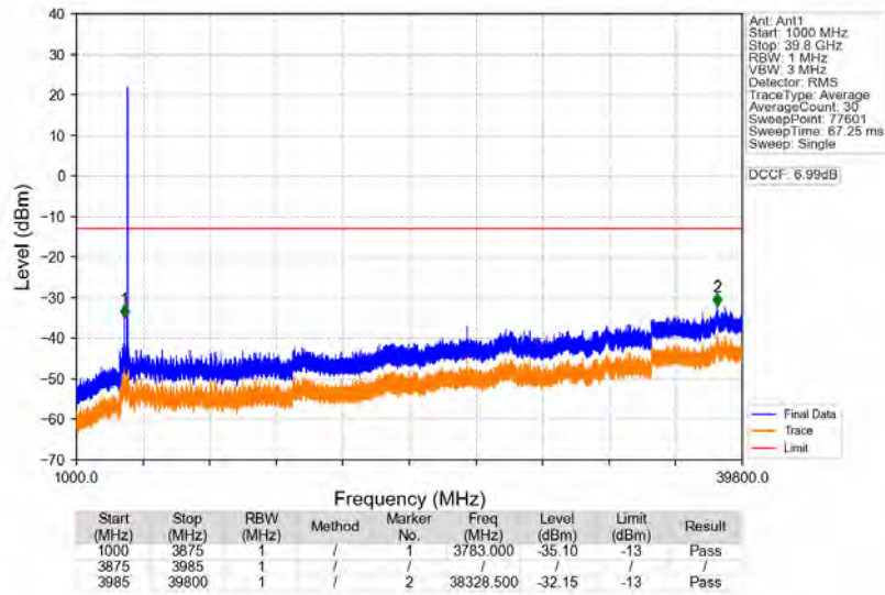
n77a 30kHz SISO NTN 100MHz DFT-s-OFDM PI/2 BPSK 3930MHz Edge_1RB_Right
