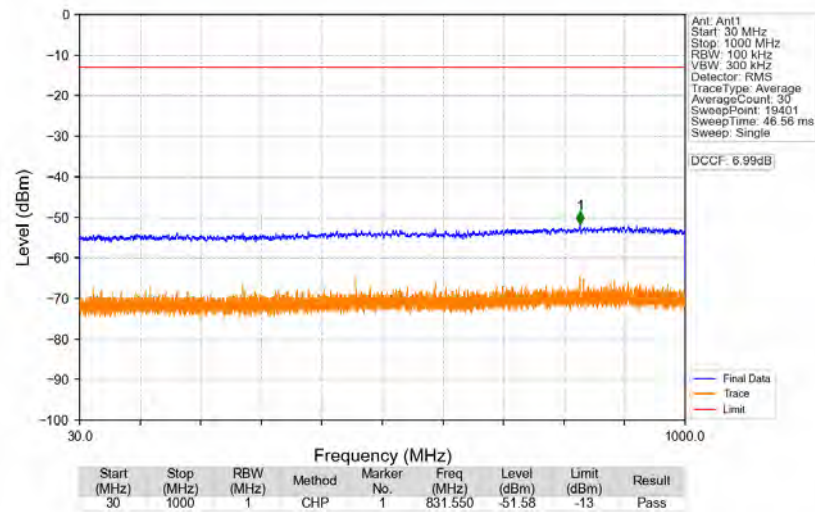
n77a_30kHz_SISO_NTNV_80MHz_DFT-s-OFDM_QPSK_3740.01MHz_Edge_1RB_Left
