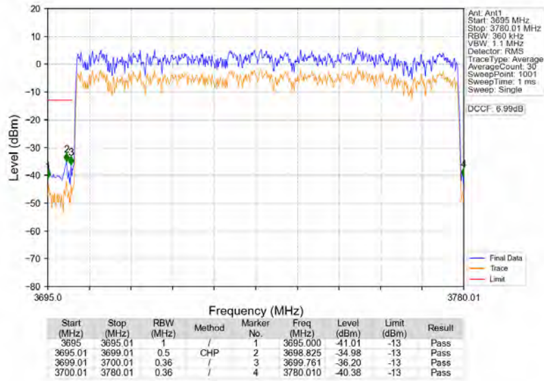
n77a_30kHz_SISO_NTNV_80MHz_DFT-s-OFDM_PI/2_BPSK_3740.01MHz_Outer_Full
