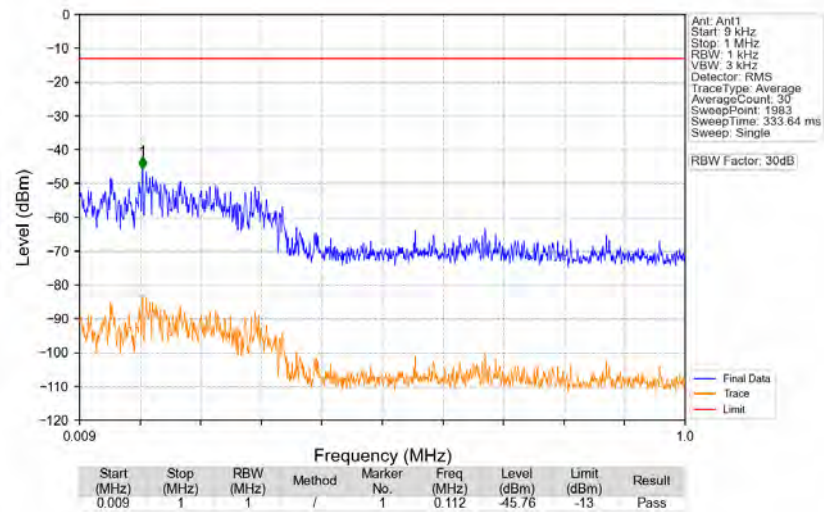
n77a_30kHz_SISO_NTNV_80MHz_DFT-s-OFDM_QPSK_3939.99MHz_Edge_1RB_Right
