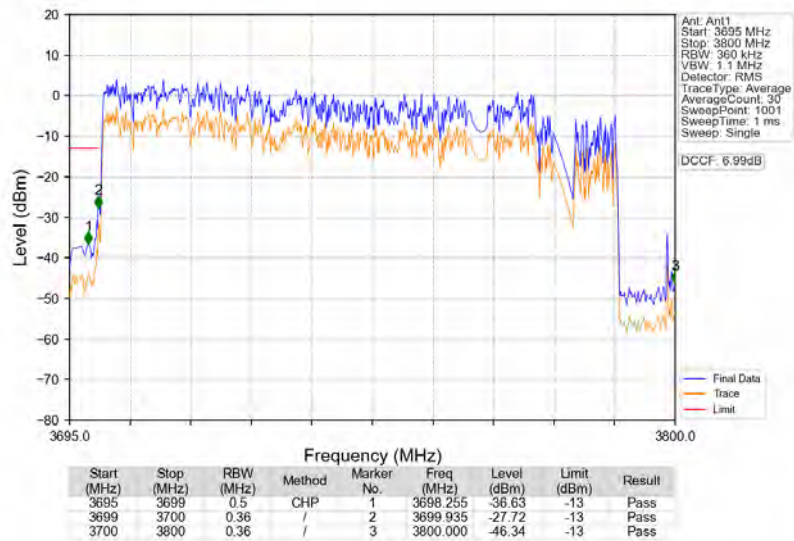
n77a_30kHz_SISO_NTNV_100MHz_DFT-s-OFDM_PI/2_BPSK_3750MHz_Outer_Full
