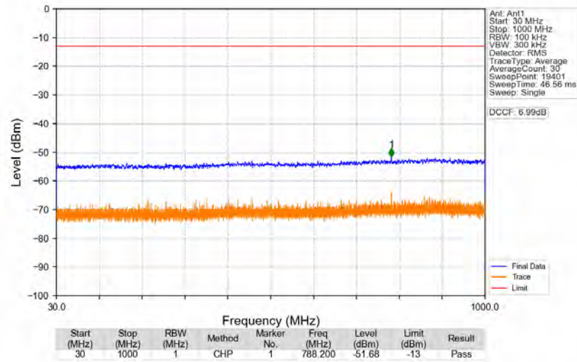
n77a_30kHz_SISO_NTNV_80MHz_CP-OFDM_QPSK_3740.01MHz_Edge_1RB_Left
