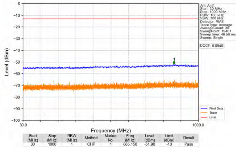
n77a_30kHz_SISO_NTNV_80MHz_DFT-s-OFDM_PI/2_BPSK_3840MHz_Edge_1RB_Left
