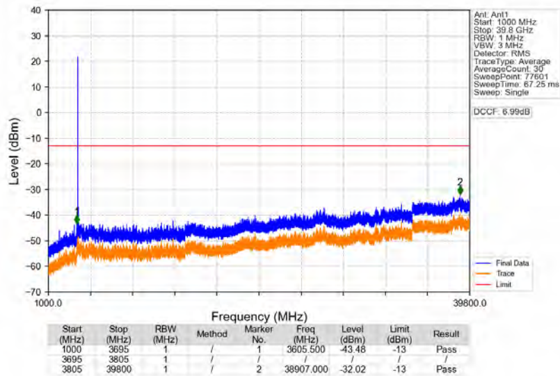
n77a_30kHz_SISO_NTNV_100MHz_DFT-s-OFDM_PI/2_BPSK_3750MHz_Edge_1RB_Left
