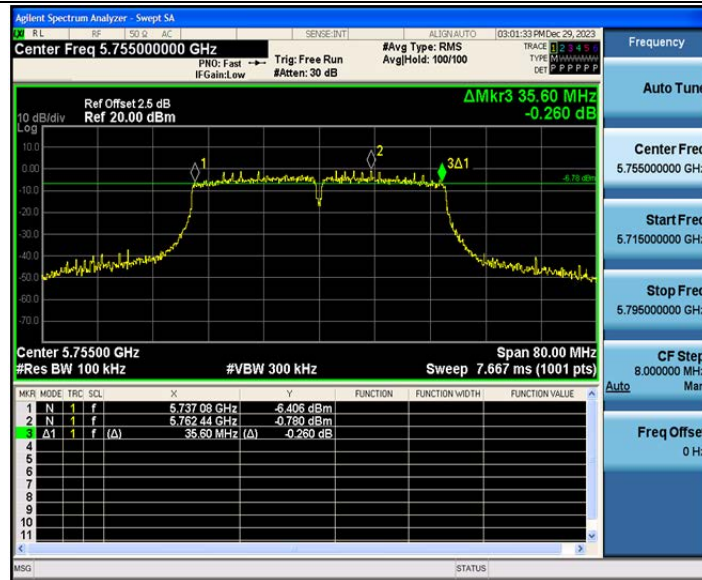
802.11n(HT40)_Ant2_5755
