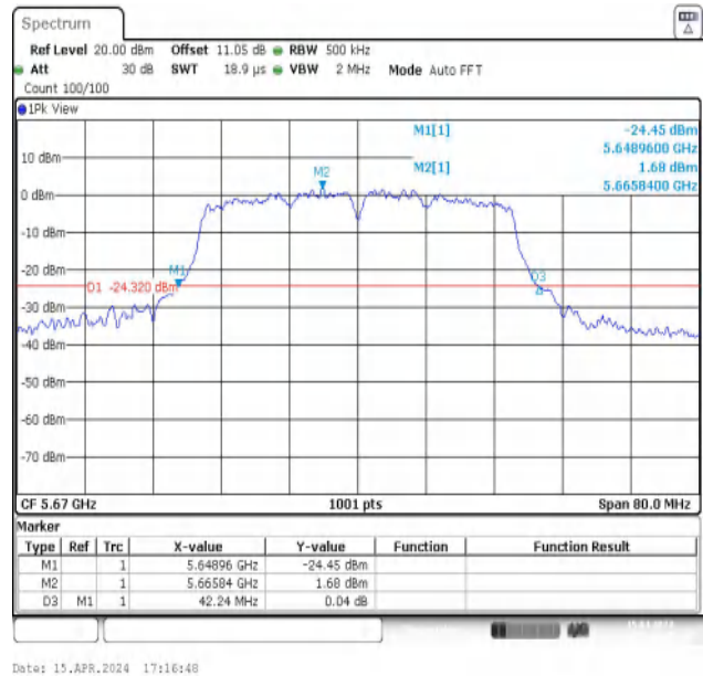
11N40MIMO-Ant2-5670
