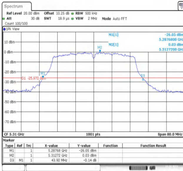
11AC40MIMO-Ant1-5310
