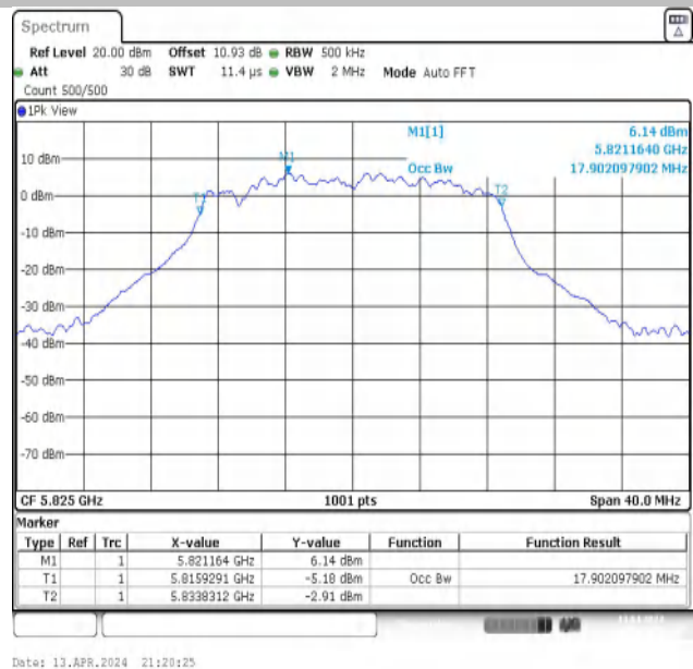
11N20MIMO-Ant2-5825
