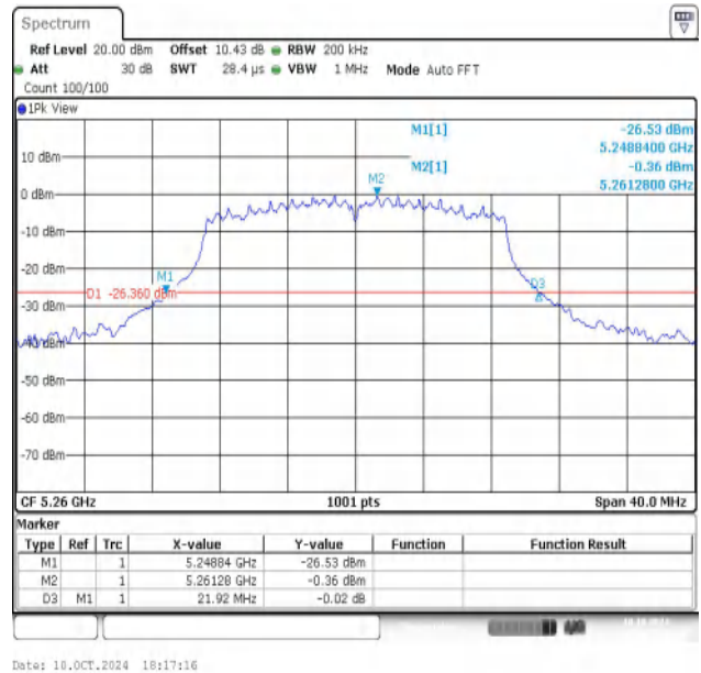
11AC20MIMO-Ant2-5260
