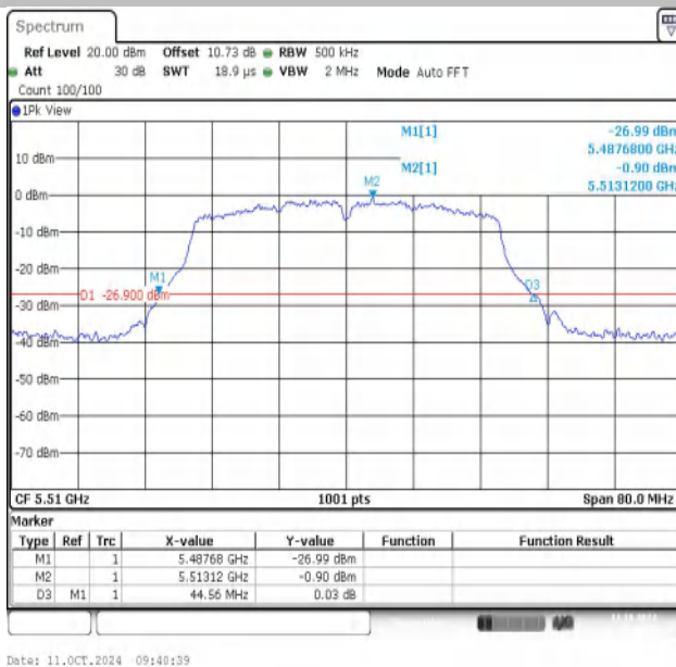
11AC40MIMO-Ant1-5510
