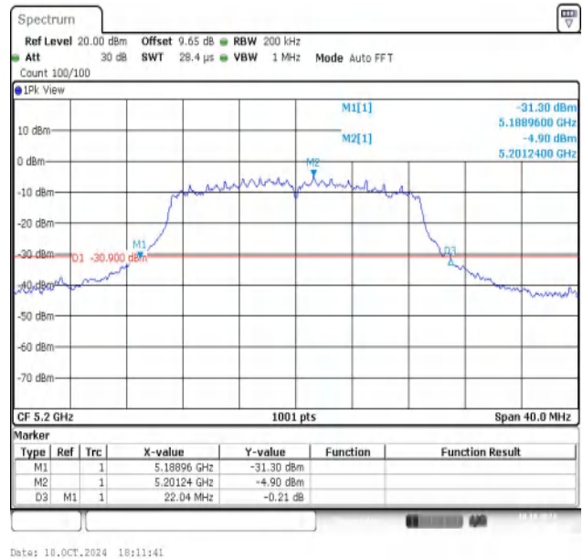
11AC20MIMO-Ant2-5200
