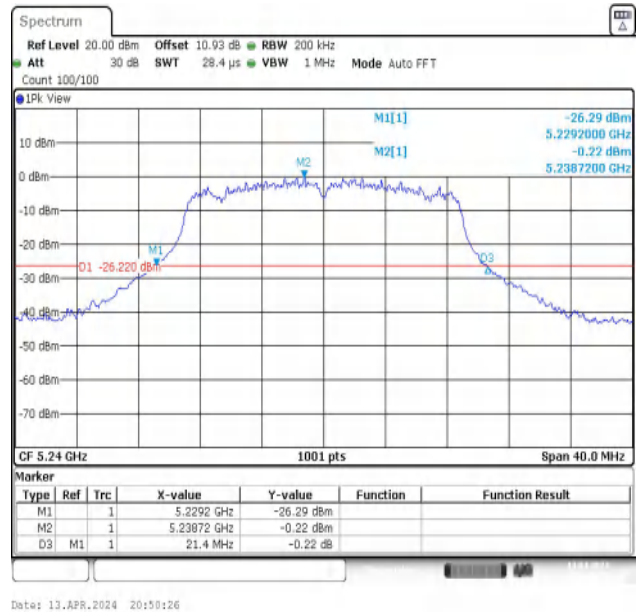
11N20MIMO-Ant2-5240
