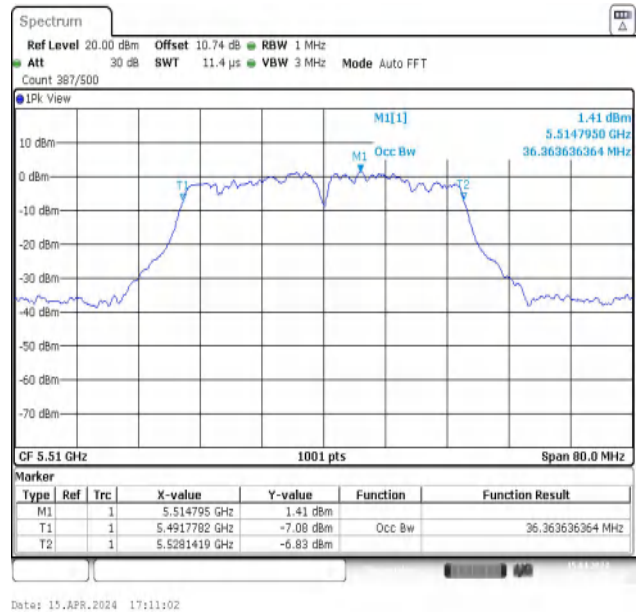
11N40MIMO-Ant2-5510
