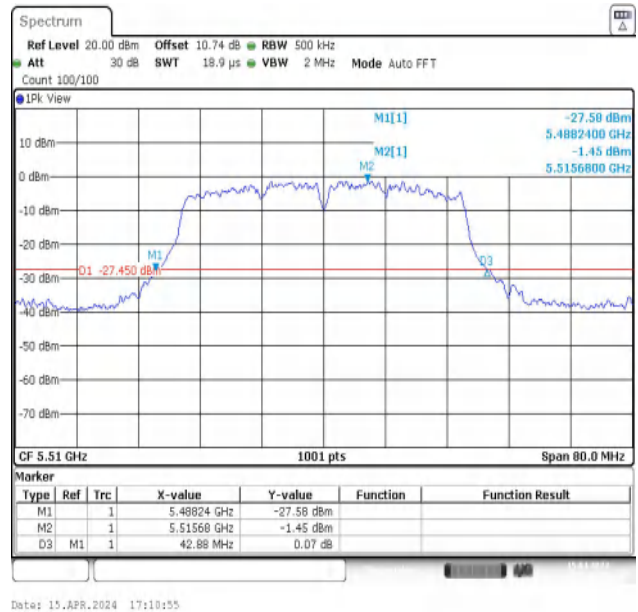
11N40MIMO-Ant2-5510
