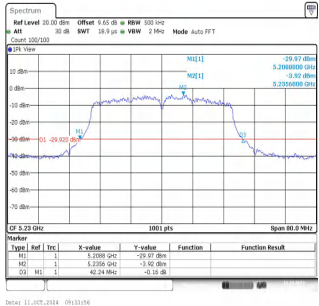
11AC40MIMO-Ant2-5230
