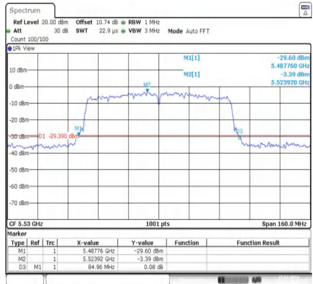
11AC80MIMO-Ant2-5530
