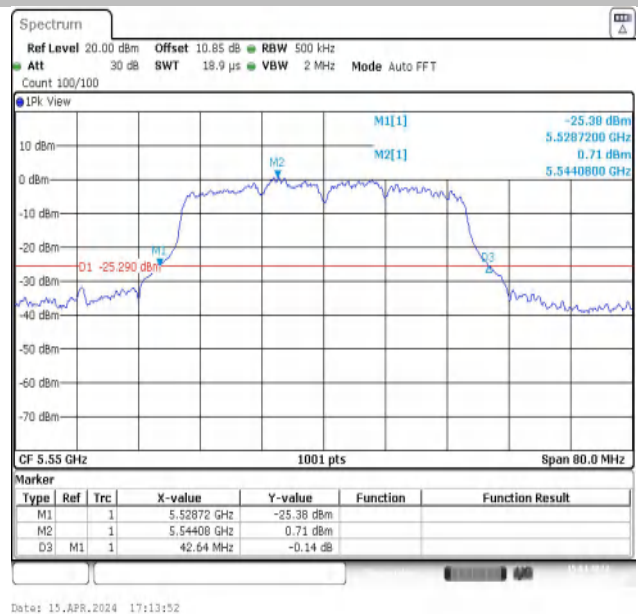
11N40MIMO-Ant2-5550
