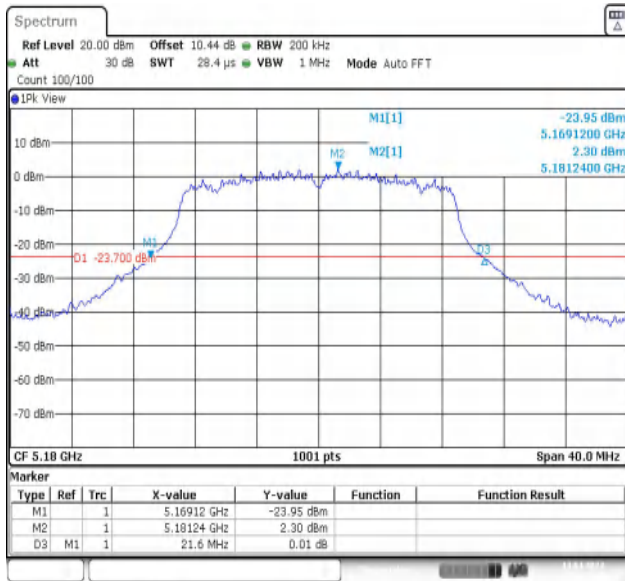
11N20MIMO-Ant1-5180
