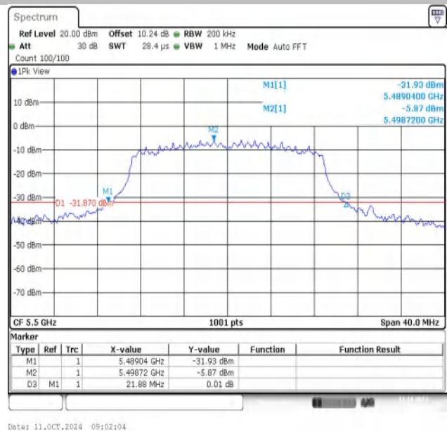
11AC20MIMO-Ant2-5500
