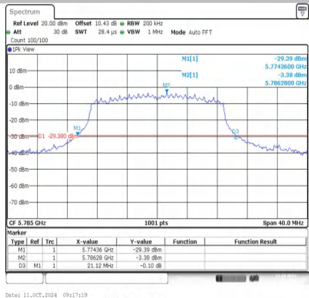
11AC20MIMO-Ant2-5785
