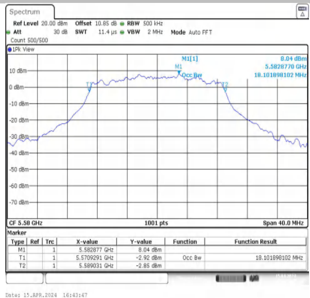
11N20MIMO-Ant2-5580
