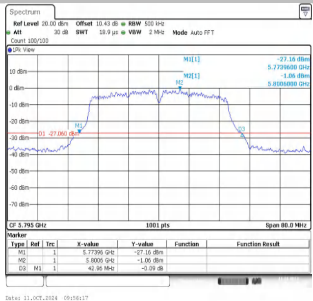
11AC40MIMO-Ant2-5795
