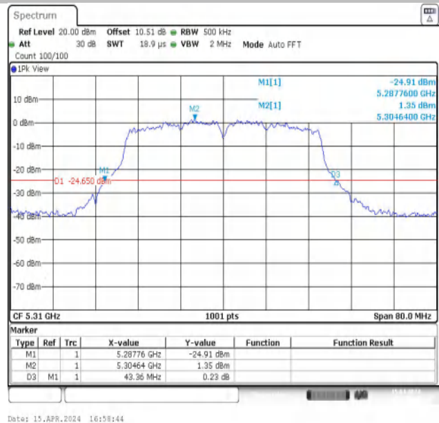
11N40MIMO-Ant2-5310
