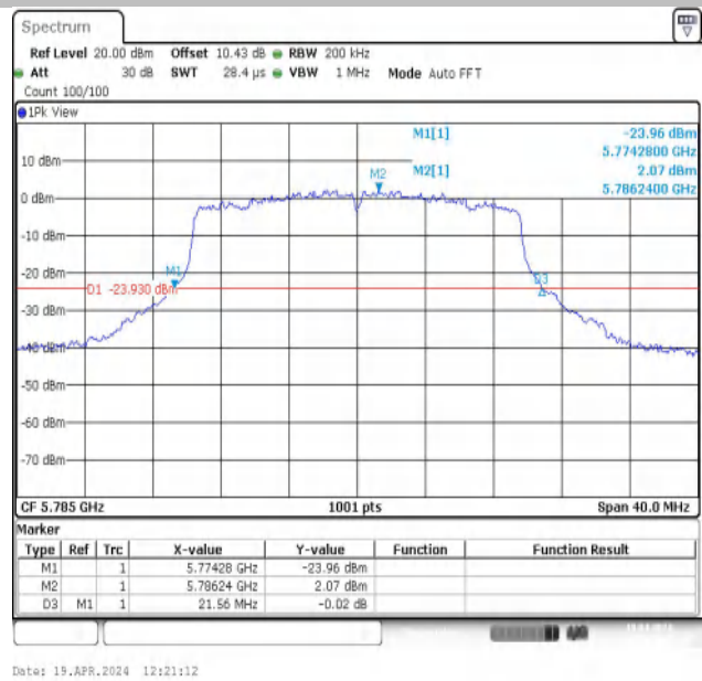
11AX20MIMO-Ant2-5785
