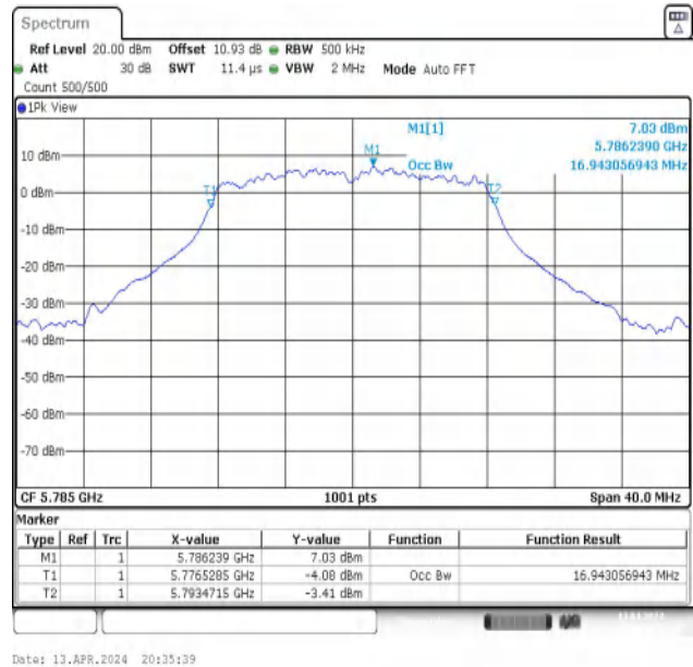
11A-Ant2-5785
