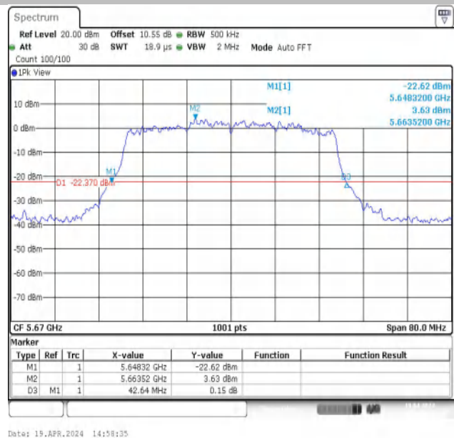
11AX40MIMO-Ant2-5670
