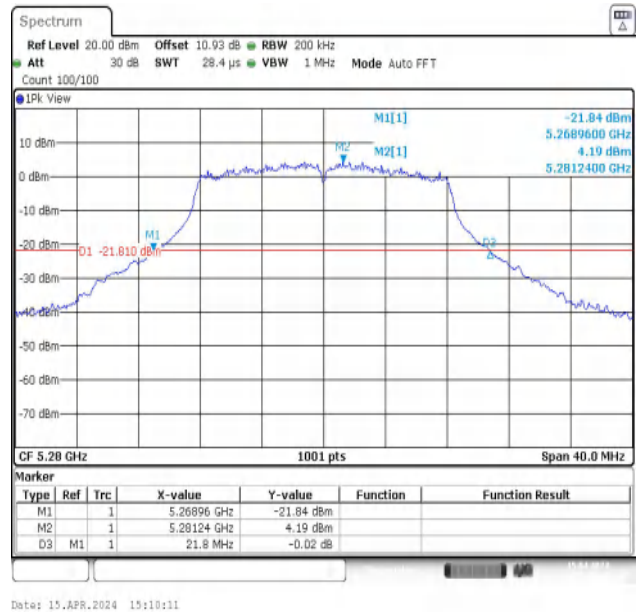
11A-Ant2-5280
