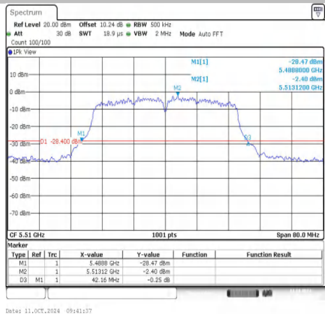
11AC40MIMO-Ant2-5510
