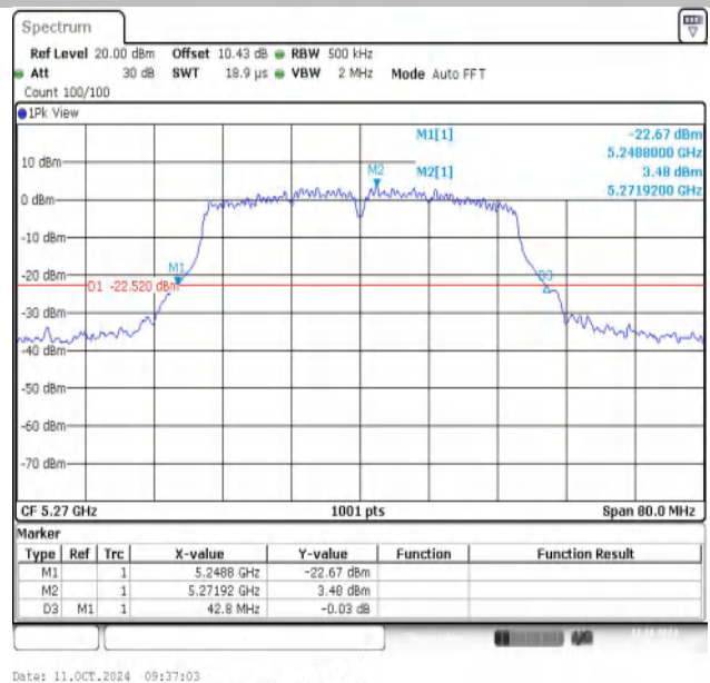
11AC40MIMO-Ant2-5270
