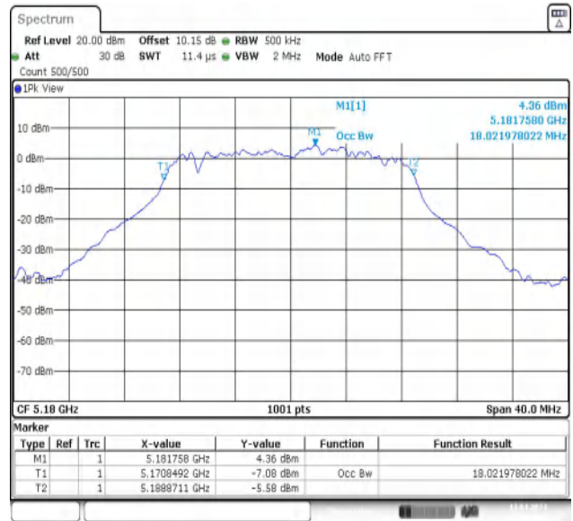
11N20MIMO-Ant2-5180
