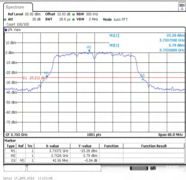
11N40MIMO-Ant2-5755
