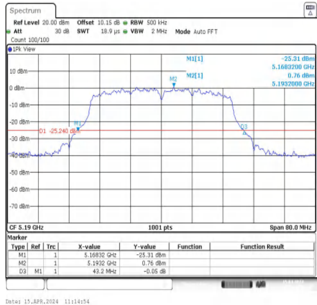
11N40MIMO-Ant2-5190
