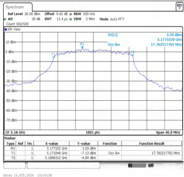
11AC20MIMO-Ant2-5180
