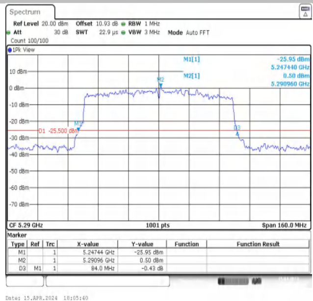
11AX80MIMO-Ant2-5290
