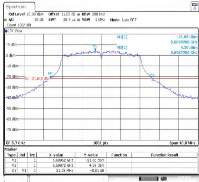
11A-Ant2-5700
