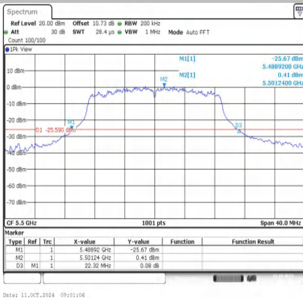
11AC20MIMO-Ant1-5500
