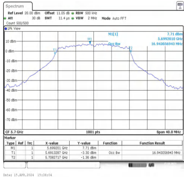
11A-Ant2-5700
