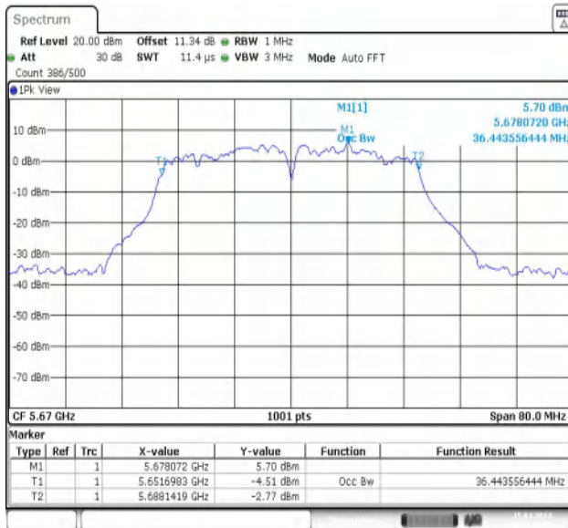
11N40MIMO-Ant1-5670
