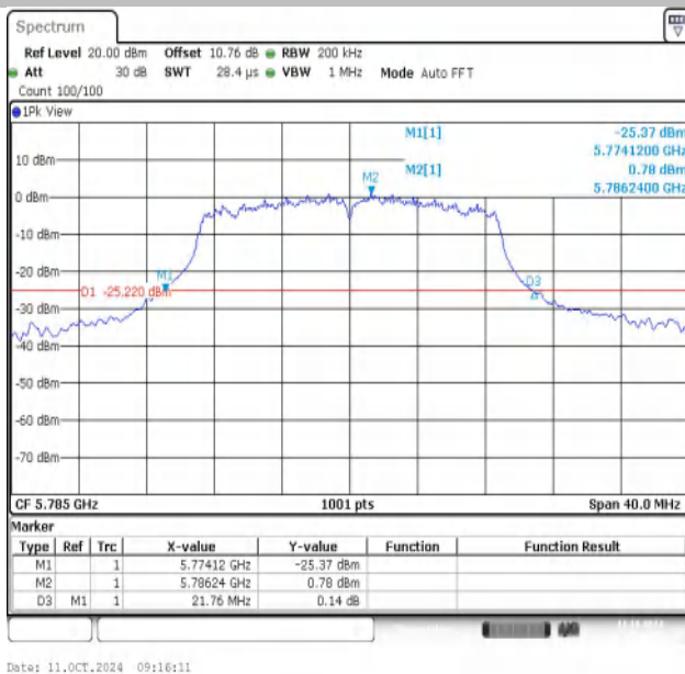
11AC20MIMO-Ant1-5785
