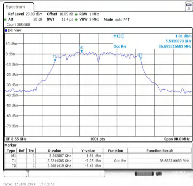
11N40MIMO-Ant2-5550
