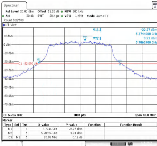
11A-Ant1-5785
