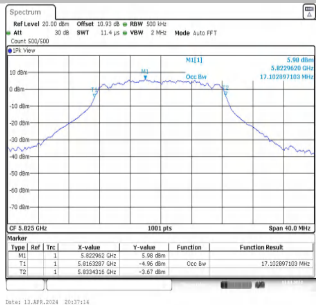
11A-Ant2-5825
