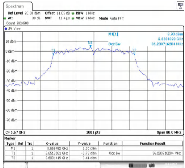
11N40MIMO-Ant2-5670
