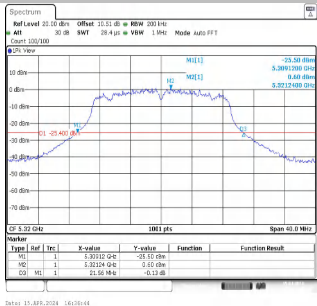
11N20MIMO-Ant2-5320
