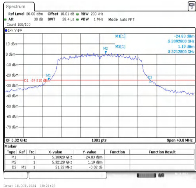
11AC20MIMO-Ant2-5320
