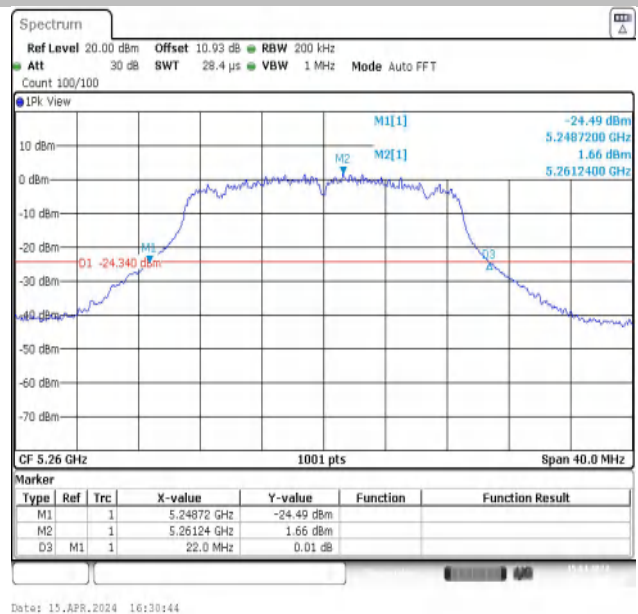
11N20MIMO-Ant2-5260
