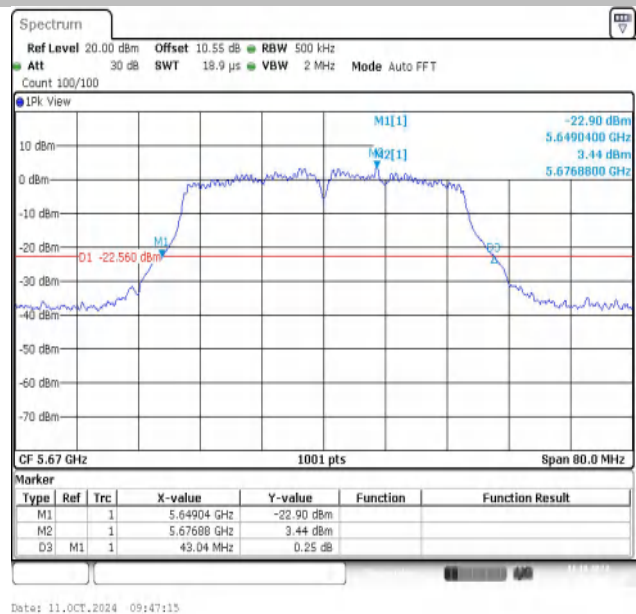
11AC40MIMO-Ant2-5670
