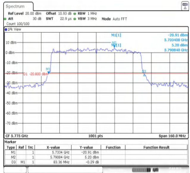
11AX80MIMO-Ant2-5775
