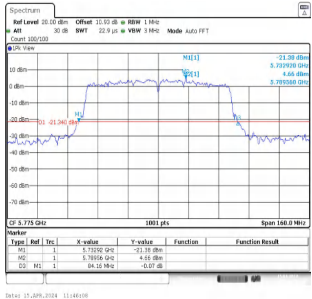
11AC80MIMO-Ant2-5775
