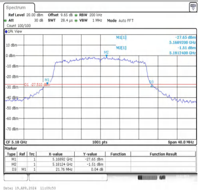
11AX20MIMO-Ant2-5180
