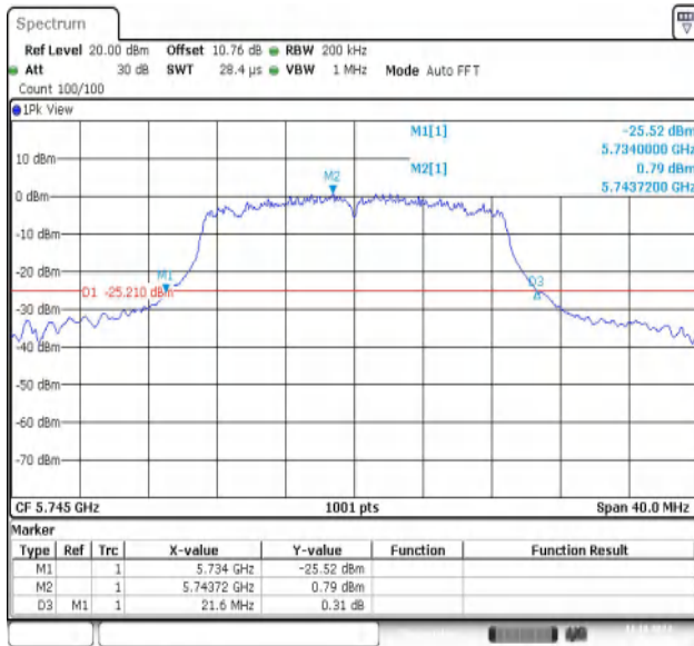
11AC20MIMO-Ant1-5745
