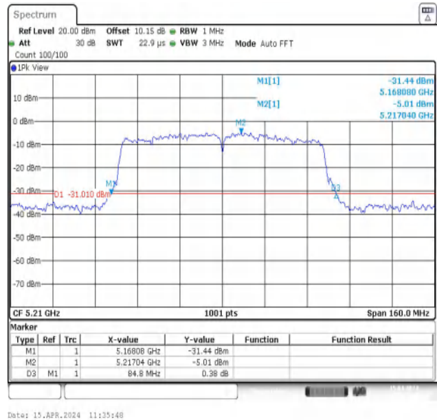
11AC80MIMO-Ant2-5210
