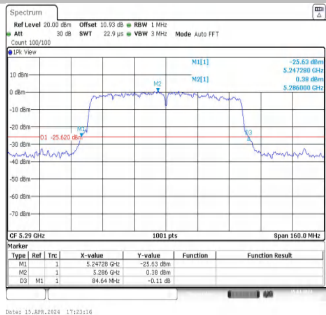
11AC80MIMO-Ant2-5290
