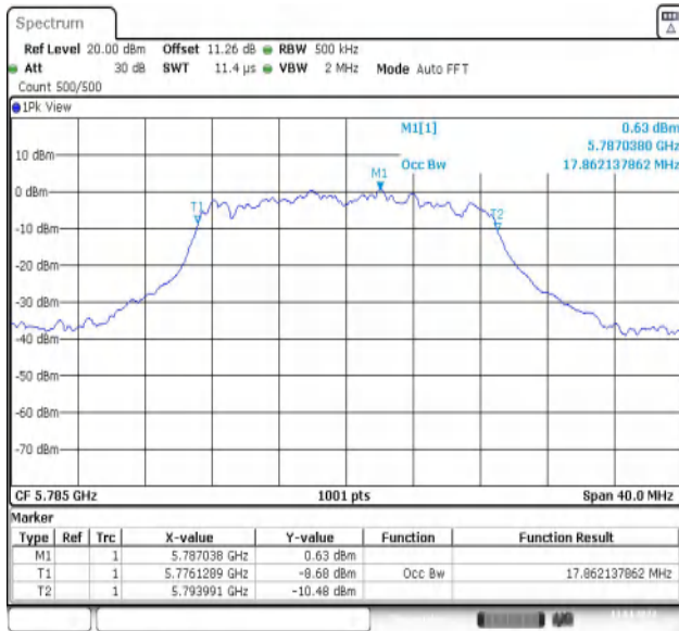
11N20MIMO-Ant1-5785
