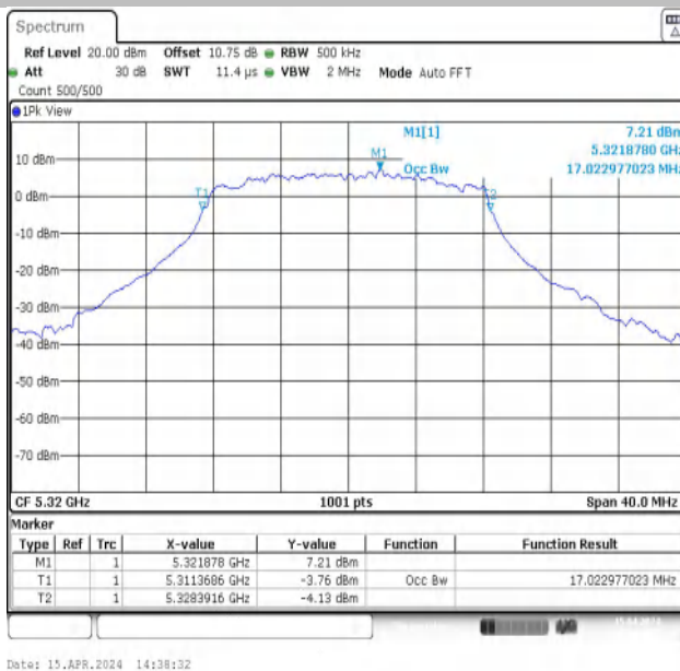
11A-Ant1-5320
