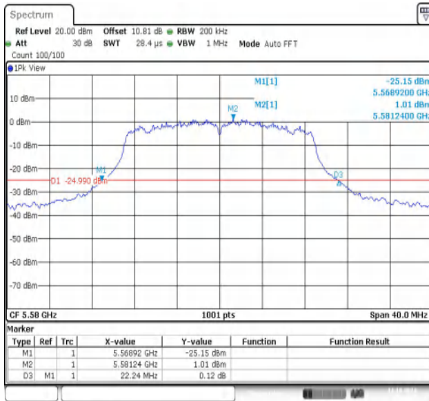
11AC20MIMO-Ant1-5580
