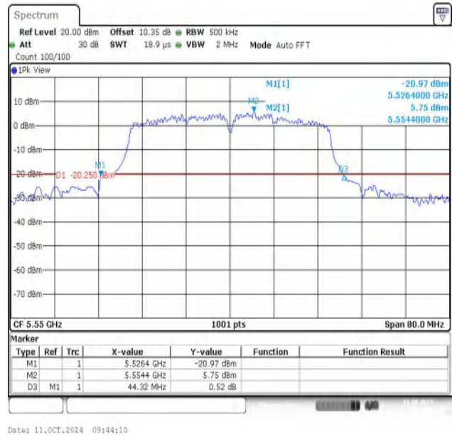
11AC40MIMO-Ant2-5550
