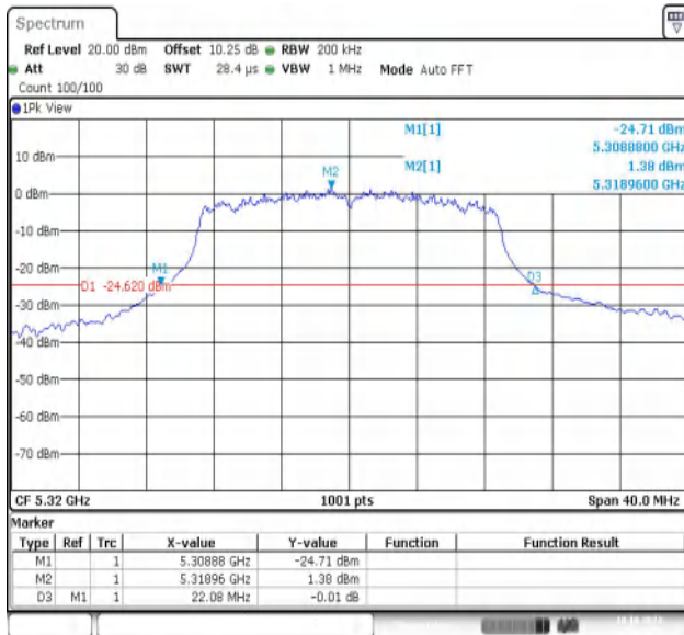
11AC20MIMO-Ant1-5320
