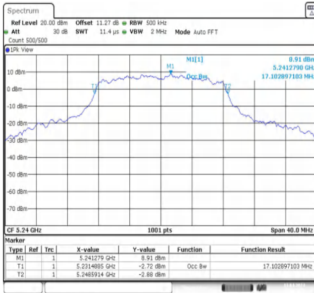
11A-Ant1-5240
