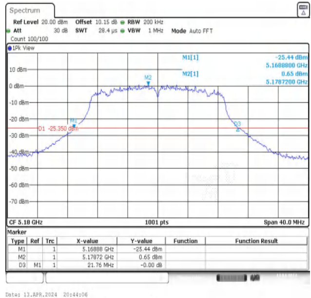
11N20MIMO-Ant2-5180
