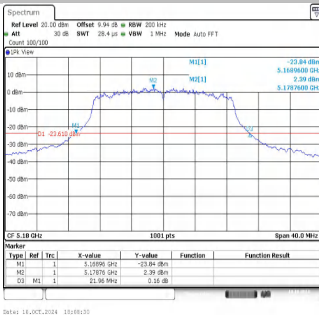
11AC20MIMO-Ant1-5180
