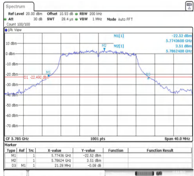
11A-Ant2-5785
