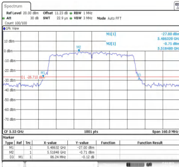
11AC80MIMO-Ant1-5530
