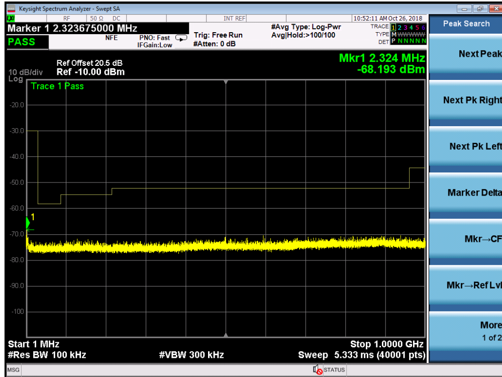
Channel Position M for FCC - QPSK / 1MHz – 1GHz
