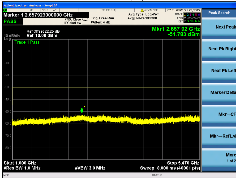
Channel Position M for FCC - QPSK / 1GHz – 5.47GHz
