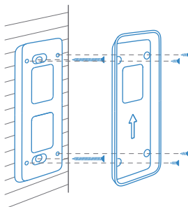
Mounting Wedge
