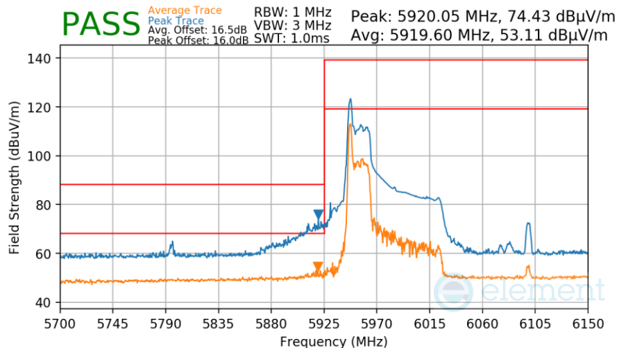
Plot 7-1041. Antenna WF7a Radiated Lower Band Edge (Peak & Average – UNII Band 5 – RU26)
