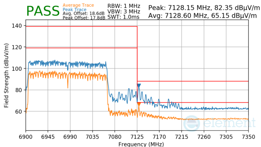
Plot 7-1072. SDM Radiated Lower Band Edge (Peak & Average – UNII Band 8 – RU996x2)
