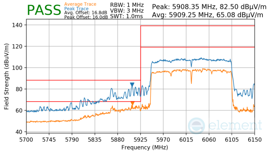
Plot 7-1048. Antenna WF7a Radiated Lower Band Edge (Peak & Average – UNII Band 5 – RU996x2)
