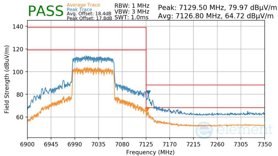
Plot 7-1066. SDM Radiated Lower Band Edge (Peak & Average – UNII Band 8 – RU996)
