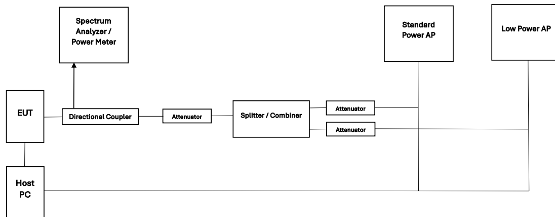
Figure 7-11. Test Instrument & Measurement Setup
