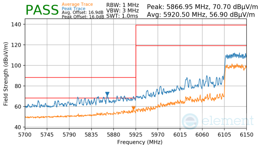
Plot 7-1070. SDM Radiated Lower Band Edge (Peak & Average – UNII Band 5 – RU996x2)
