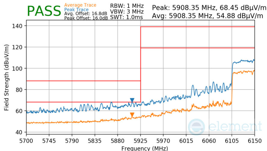
Plot 7-1049. Antenna WF7a Radiated Lower Band Edge (Peak & Average – UNII Band 5 – RU996x2)
