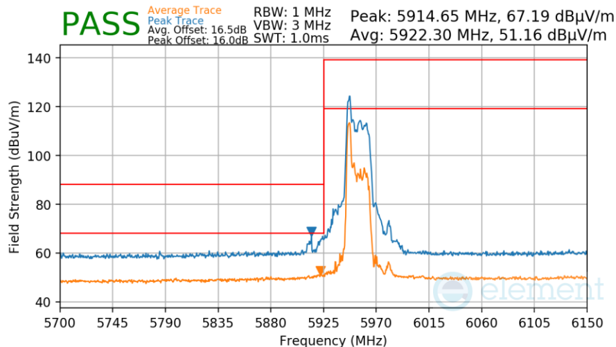
Plot 7-1052. SDM Radiated Lower Band Edge (Peak/Average – UNII Band 5 – RU26)
