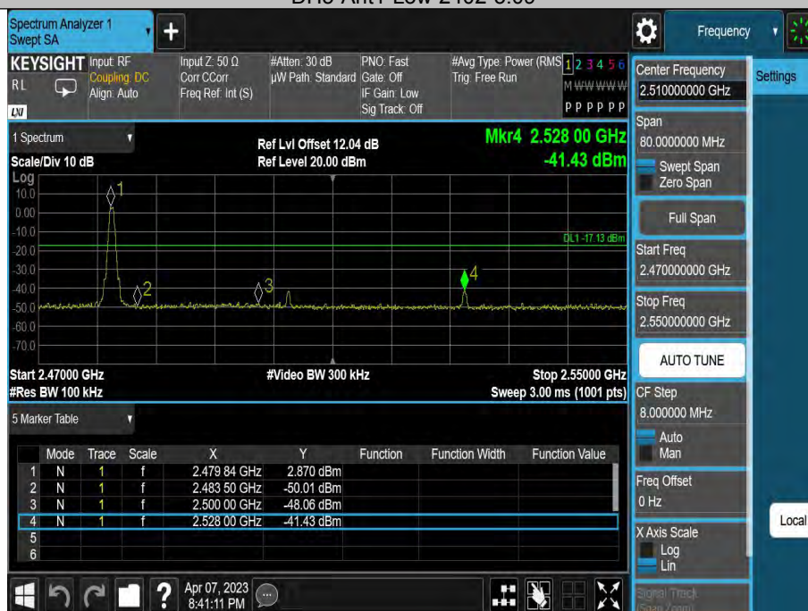
DH5-Ant1-High-2480-2.87
