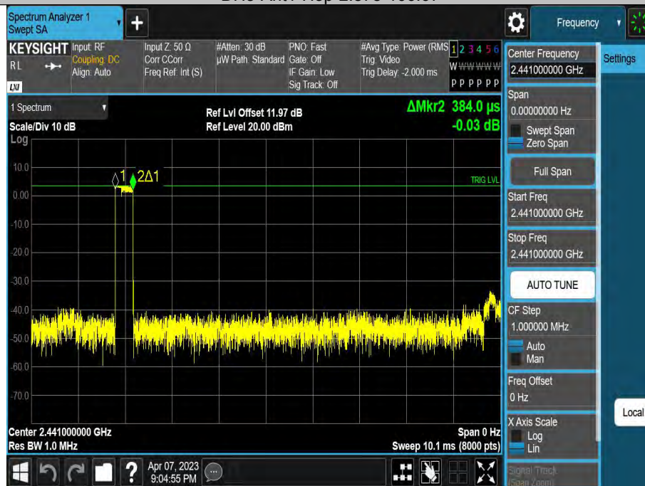
2DH1-Ant1-Hop-0.384-320
