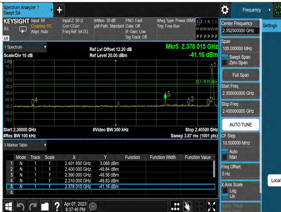
DH5-Ant1-Low-2402-3.09
