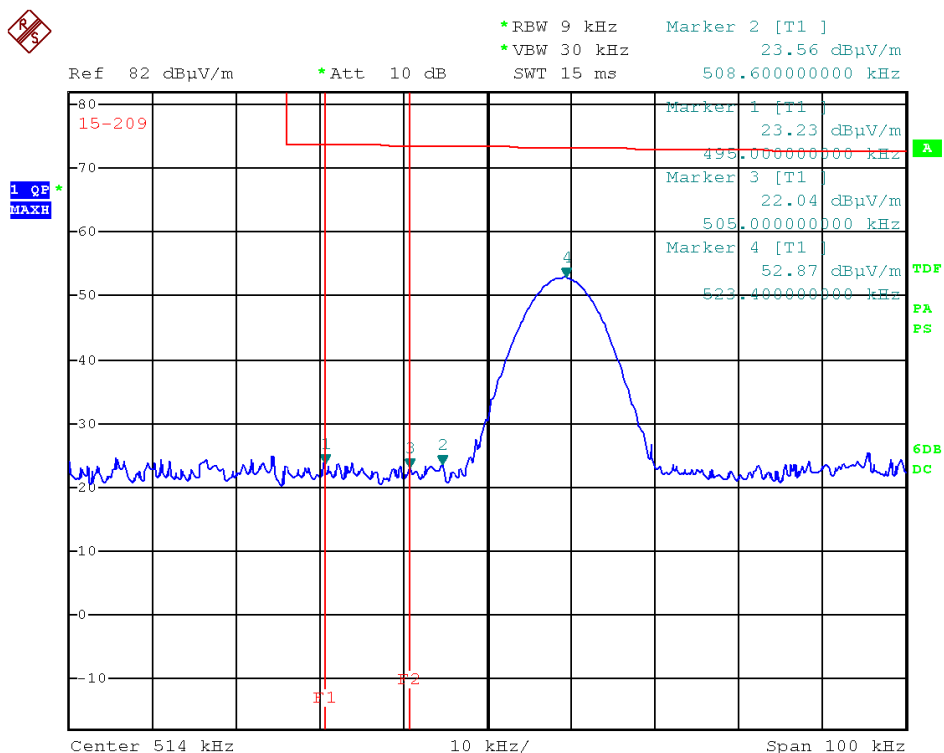
Picture 10: Restricted Band - QP @ 3m distance
