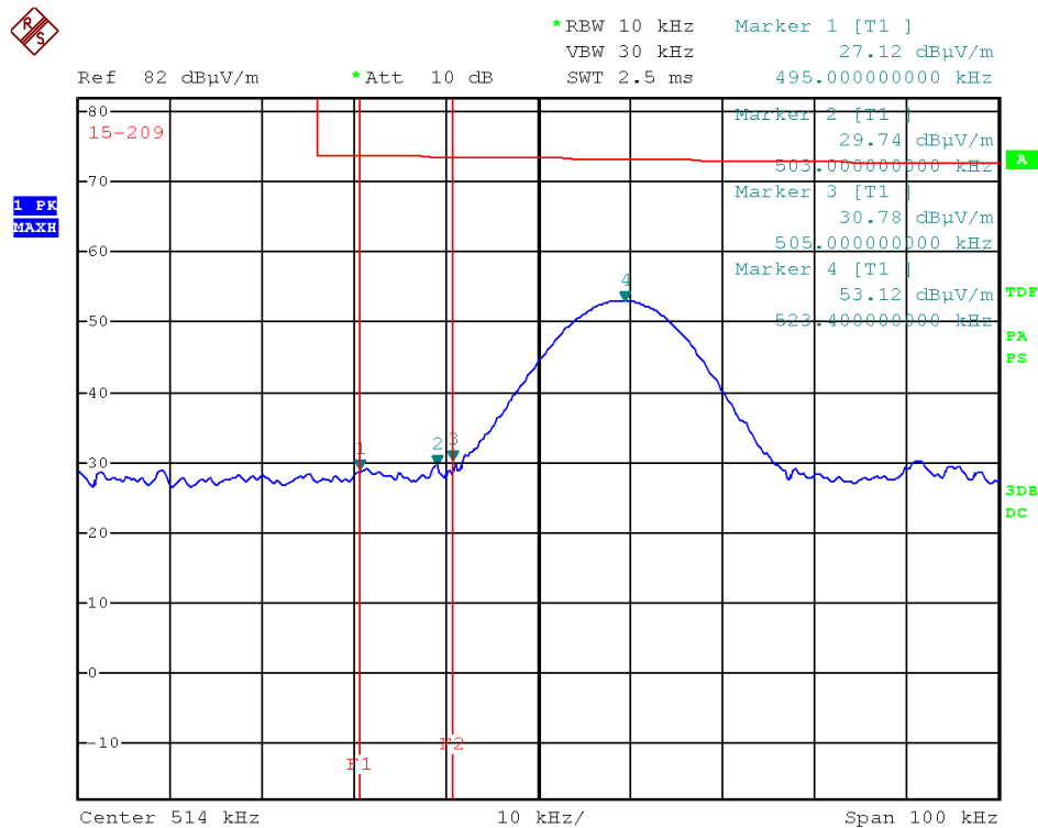
Picture 9: Restricted Band - PK @ 3m distance
