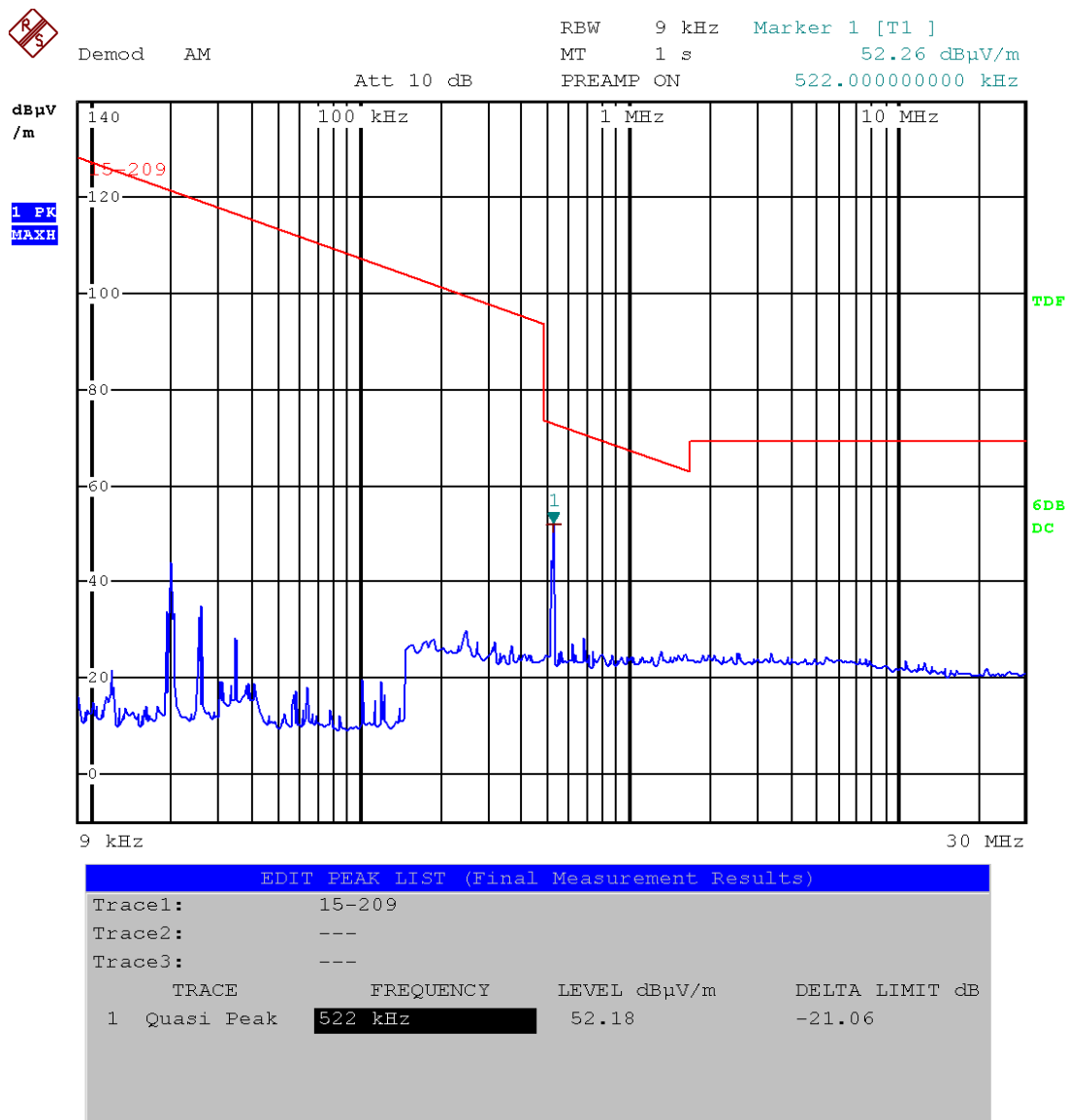
Picture 8: Radiated emission 9 kHz – 30 MHz @ 3m distance
