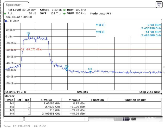
Right bandedge
