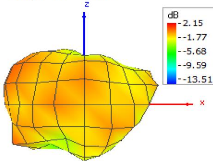
Figure A-3 Pattern at 2412 MHz (Left / Right view)
